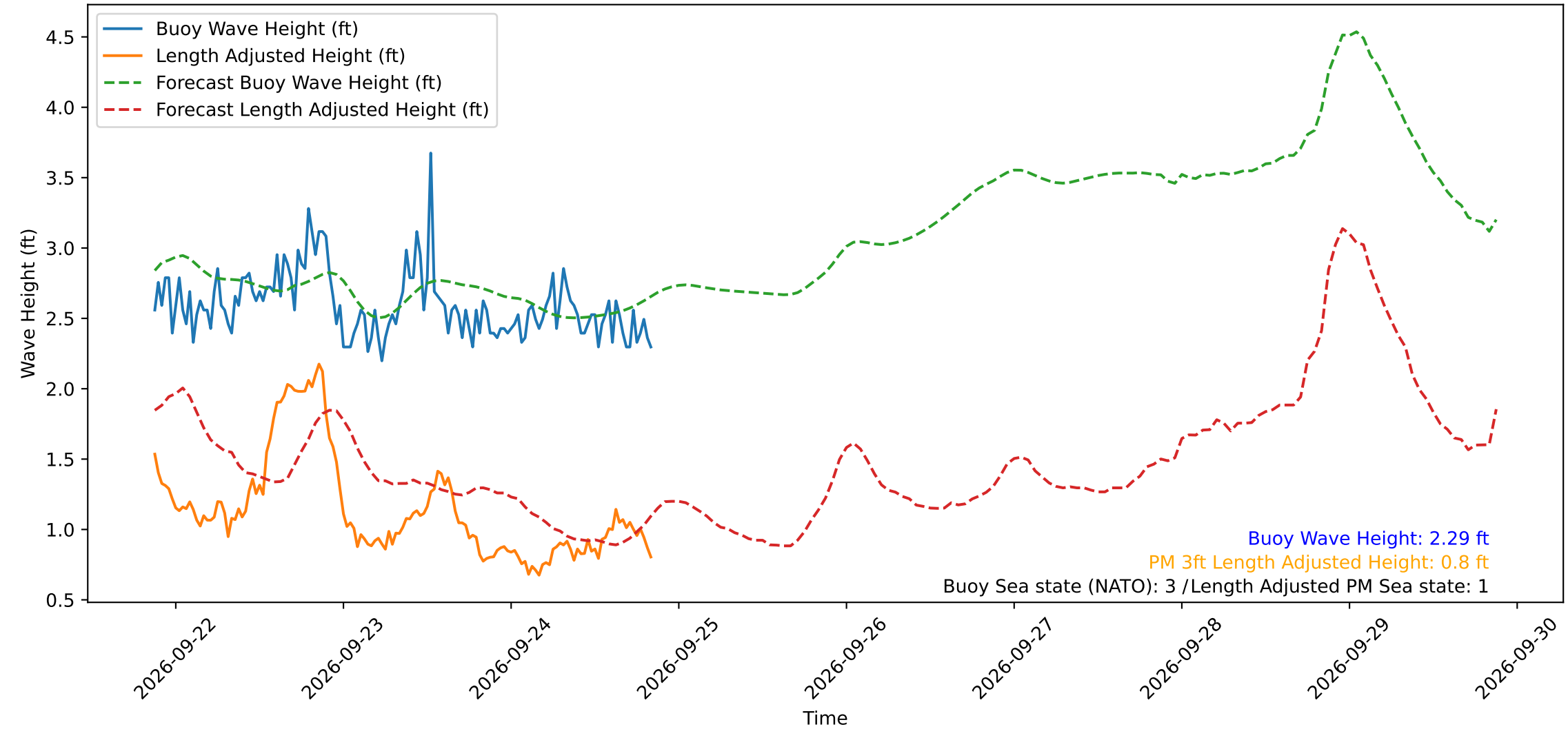
Wave Heights over Time for Red Beach at 2026-09-24 20:50:51
