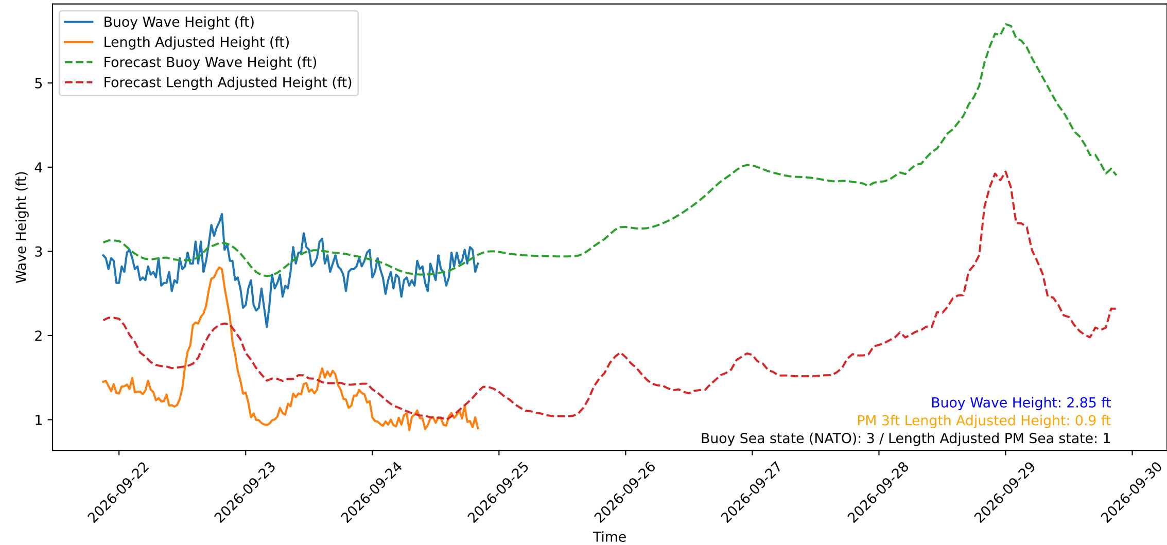
Wave Heights over Time for Green Beach at 2026-09-24 20:51:15
