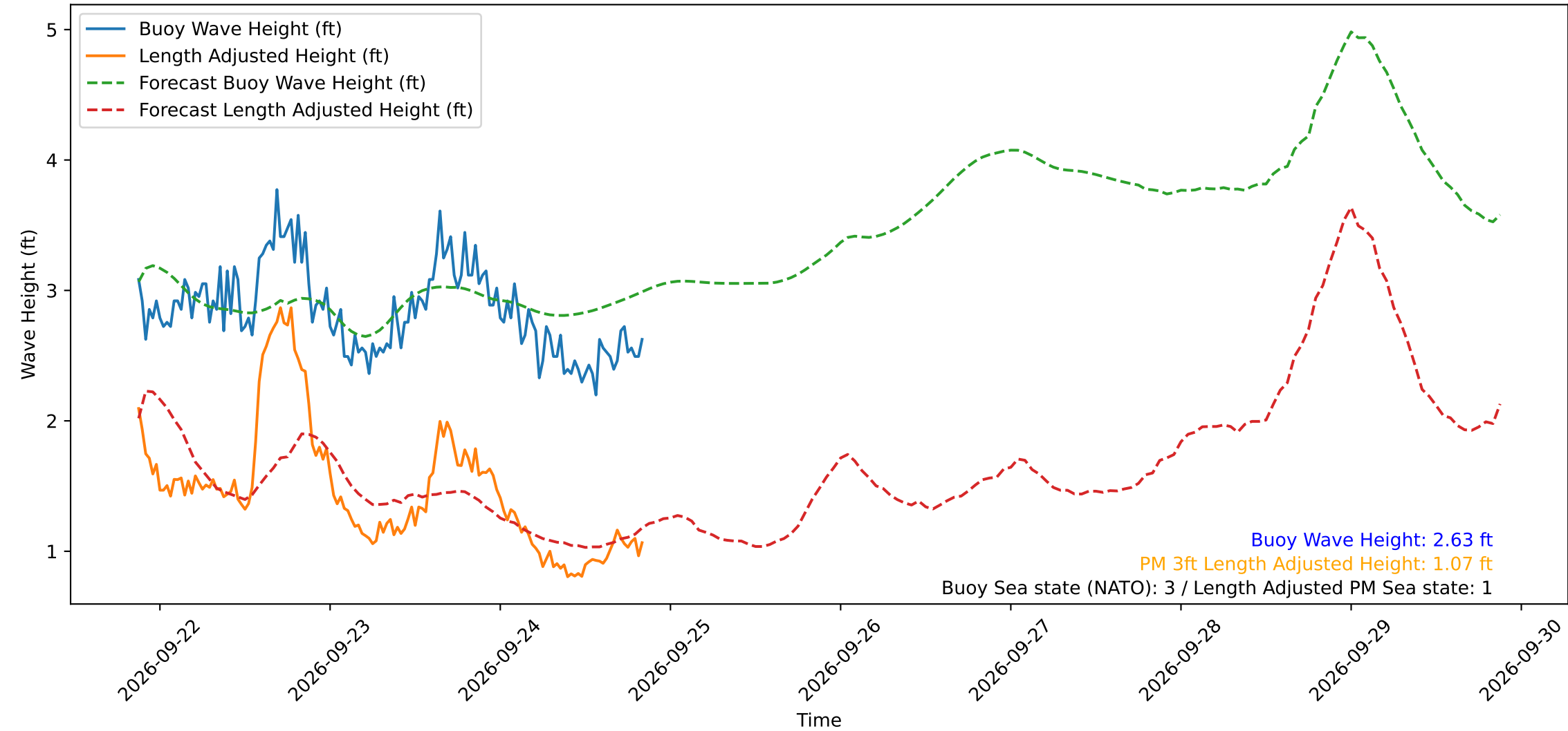
Wave Heights over Time for Oceanside Harbor at 2026-09-24 20:50:30
