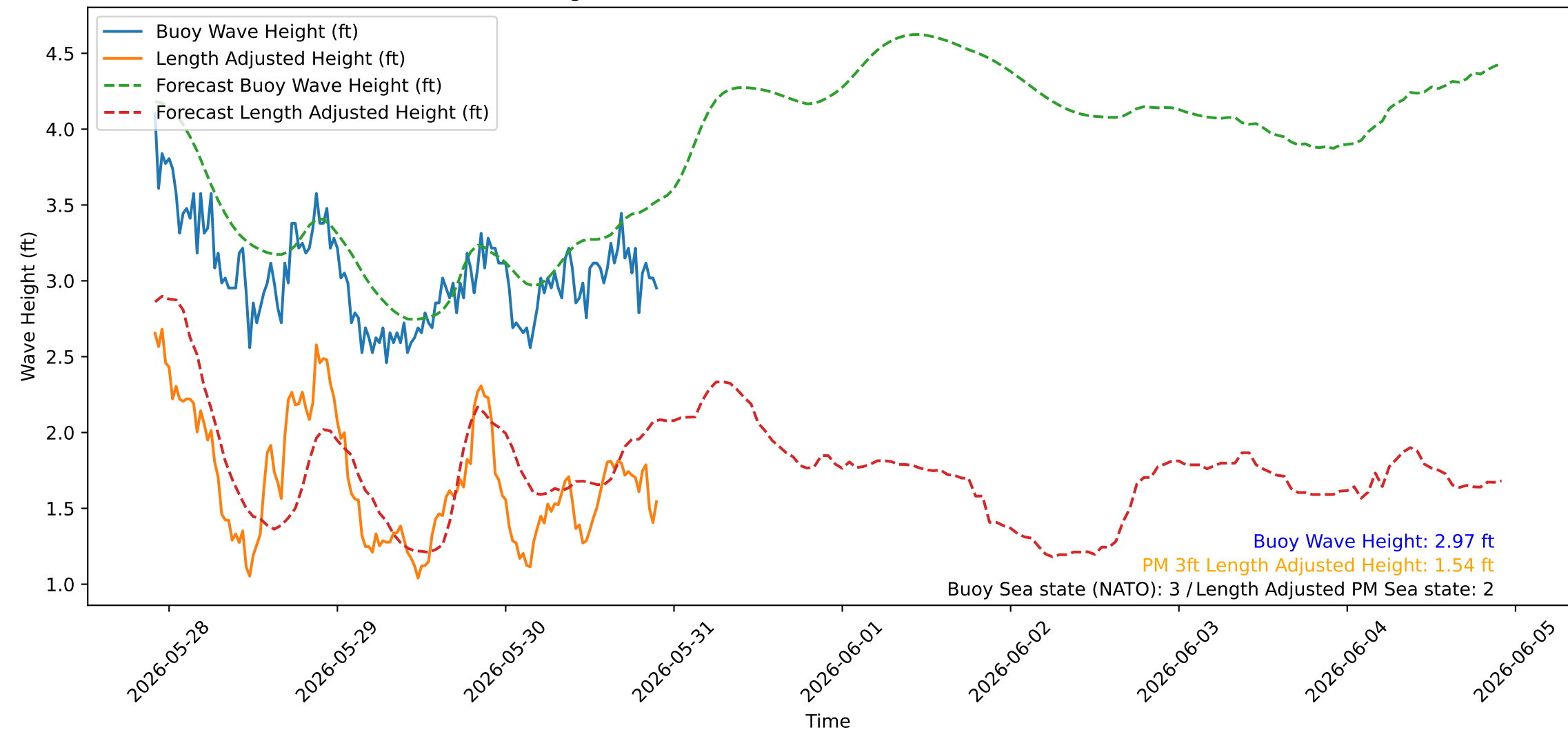
Wave Heights over Time for Green Beach at 2026-05-30 22:11:06
