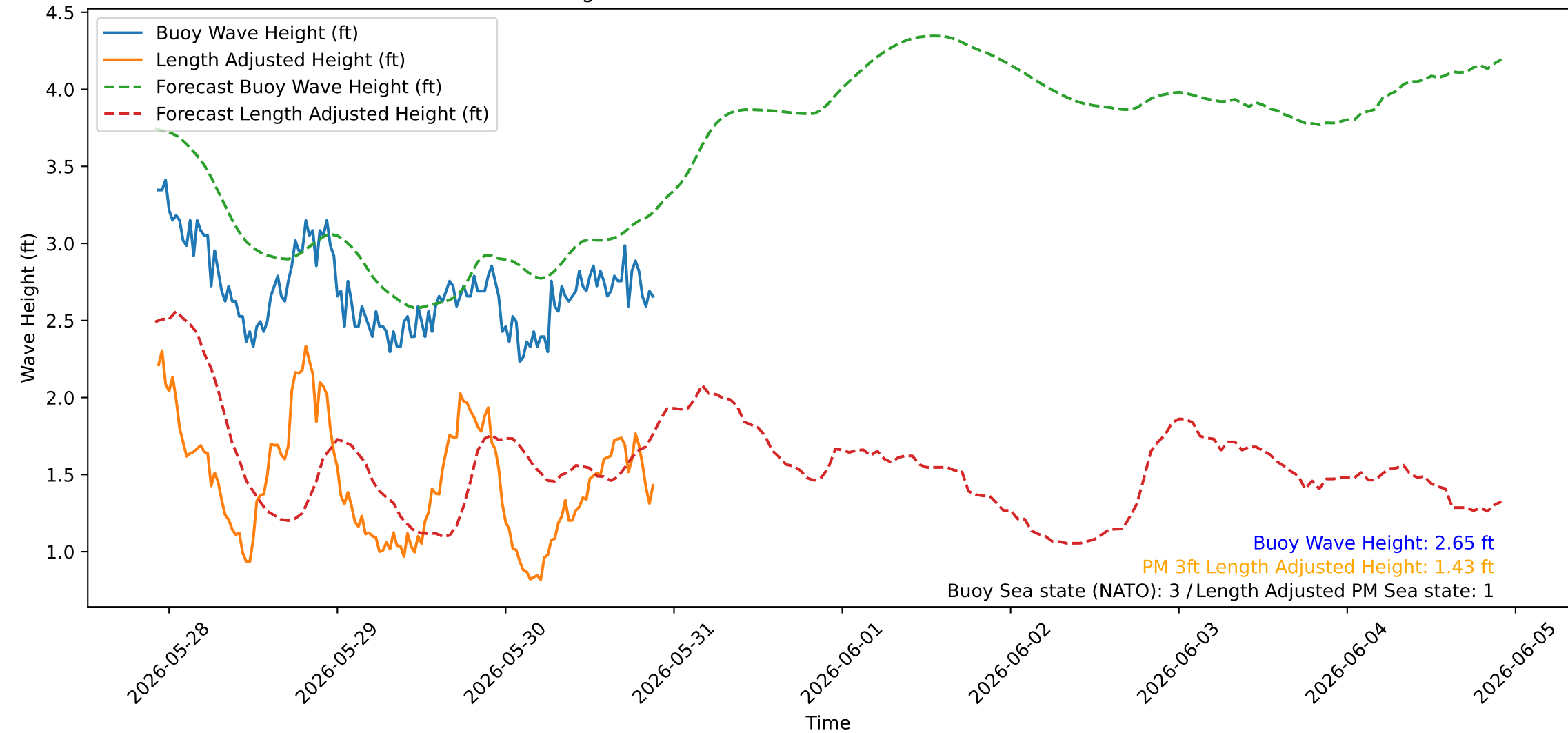
Wave Heights over Time for Red Beach at 2026-05-30 22:10:44
