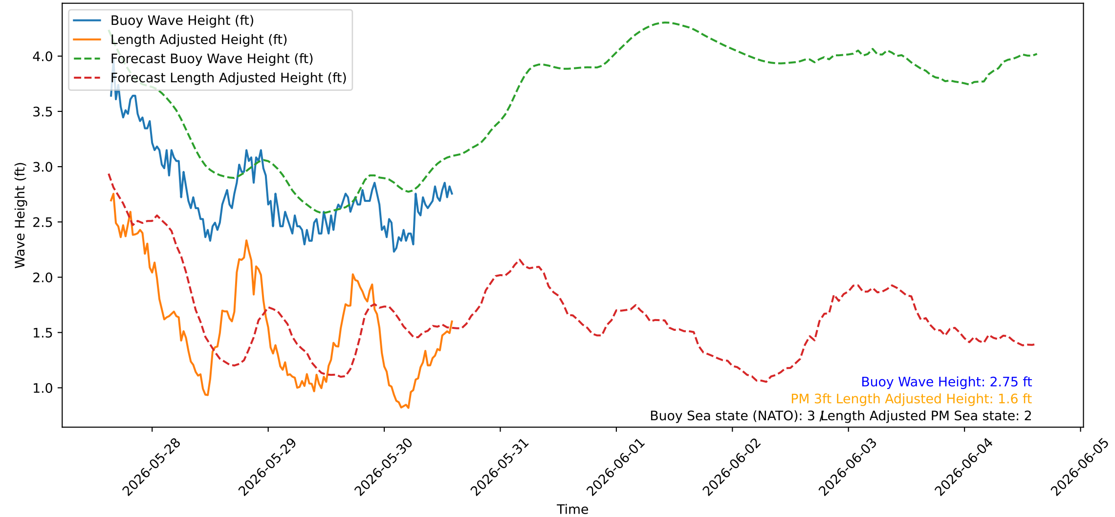
Wave Heights over Time for Red Beach at 2026-05-30 15:10:42
