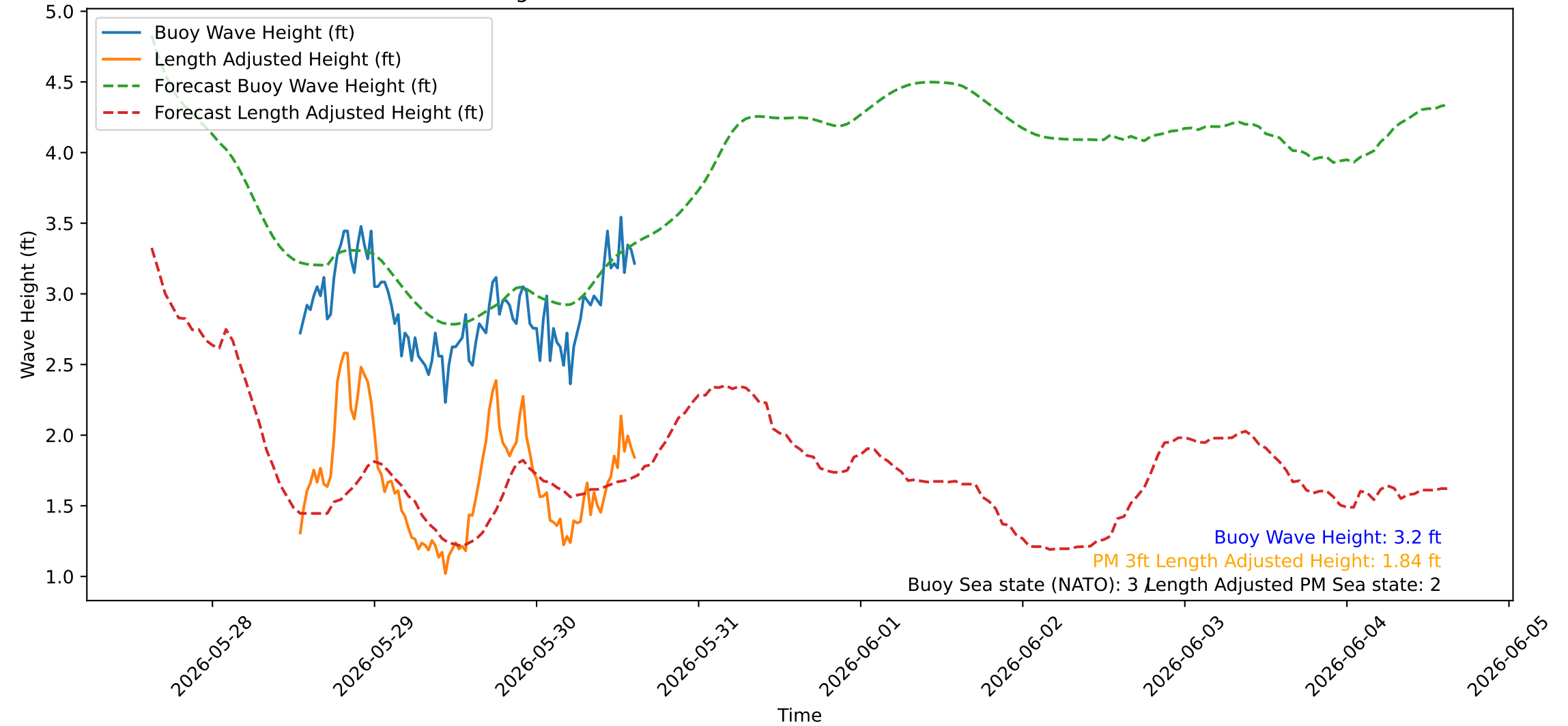
Wave Heights over Time for Oceanside Harbor at 2026-05-30 15:10:23
