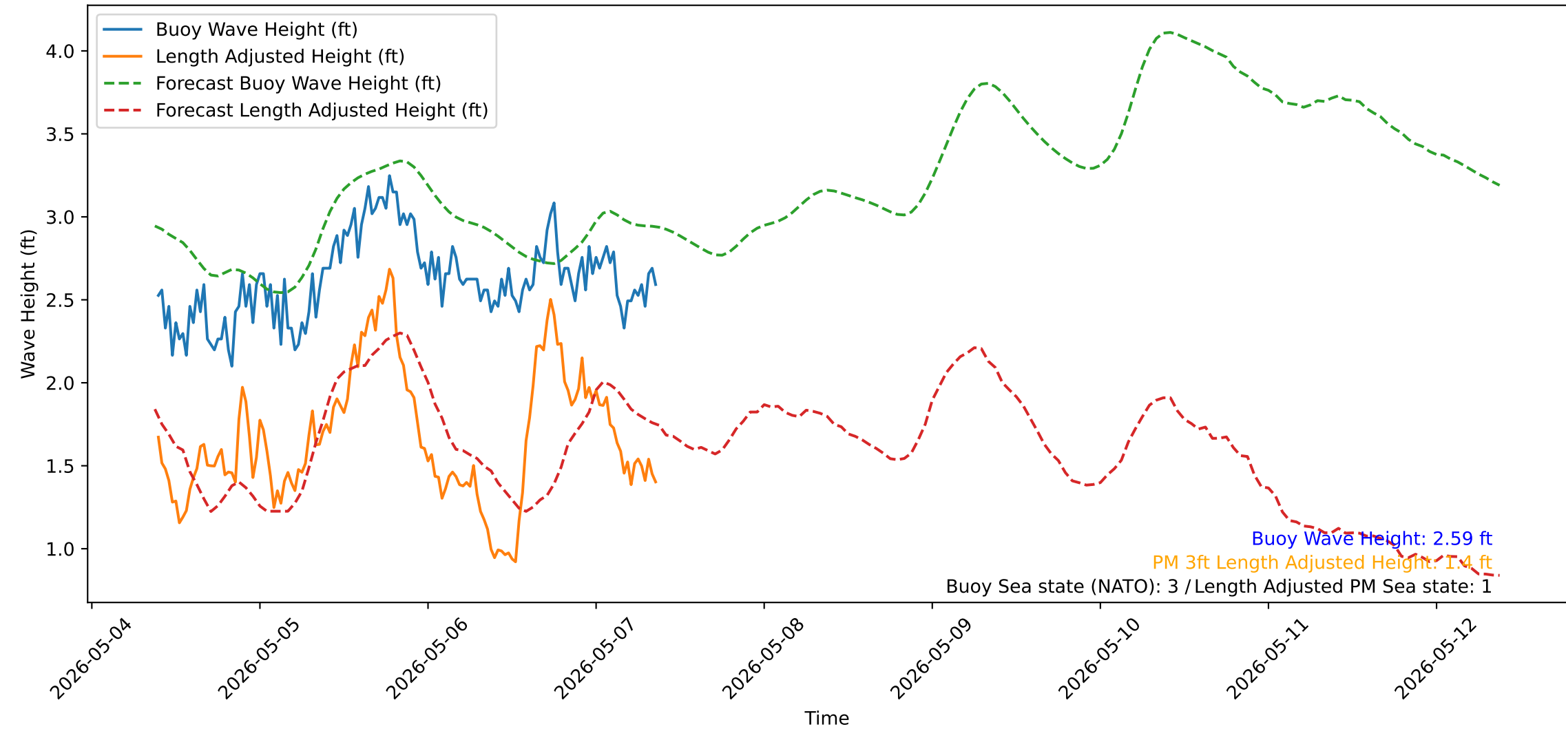
Wave Heights over Time for Oceanside Harbor at 2026-05-07 09:20:31
