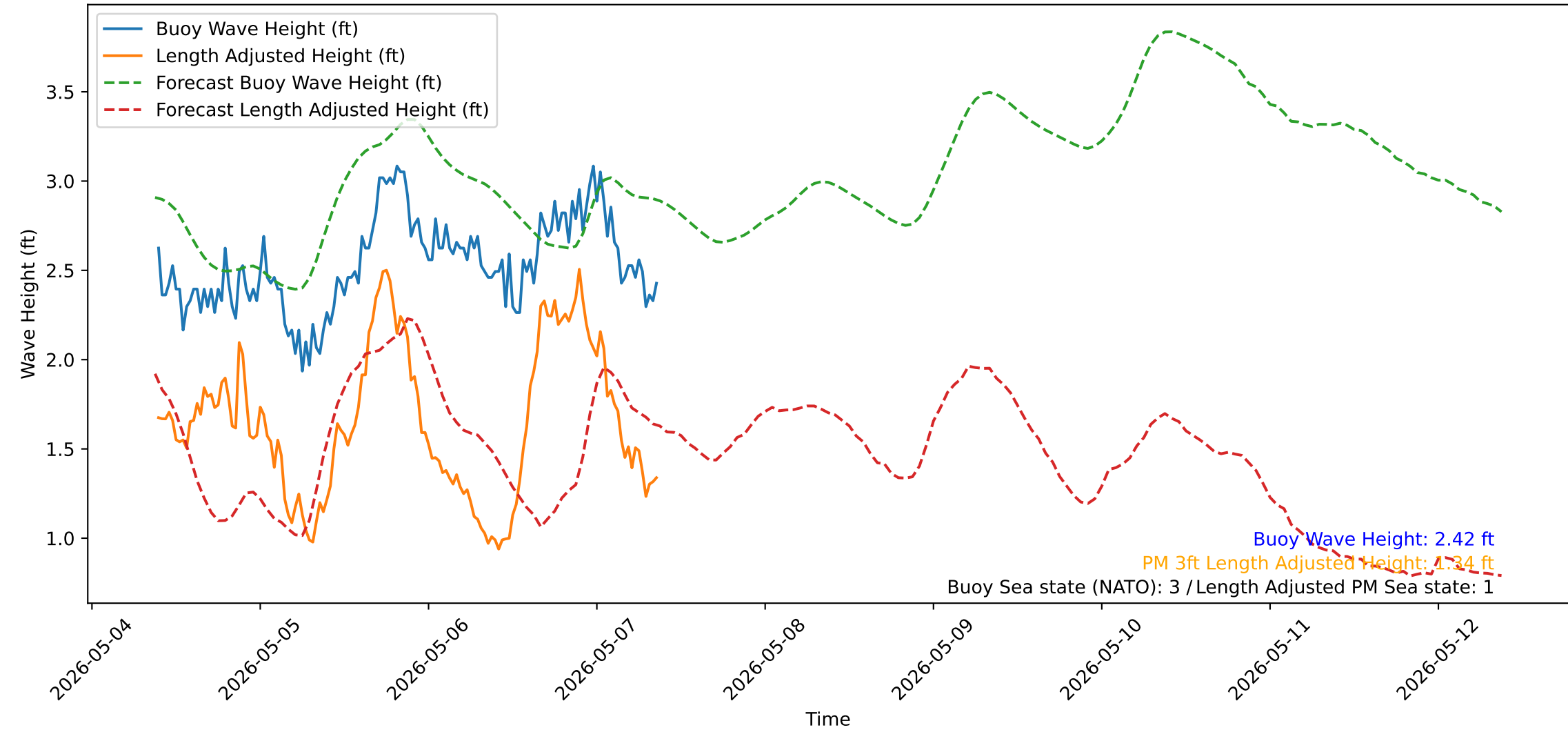
Wave Heights over Time for Red Beach at 2026-05-07 09:20:52
