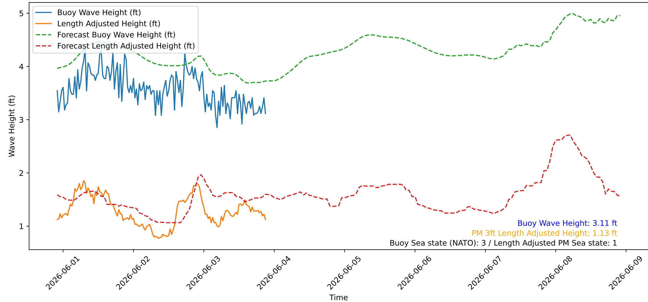
Wave Heights over Time for Green Beach at 2026-06-03 22:01:08
