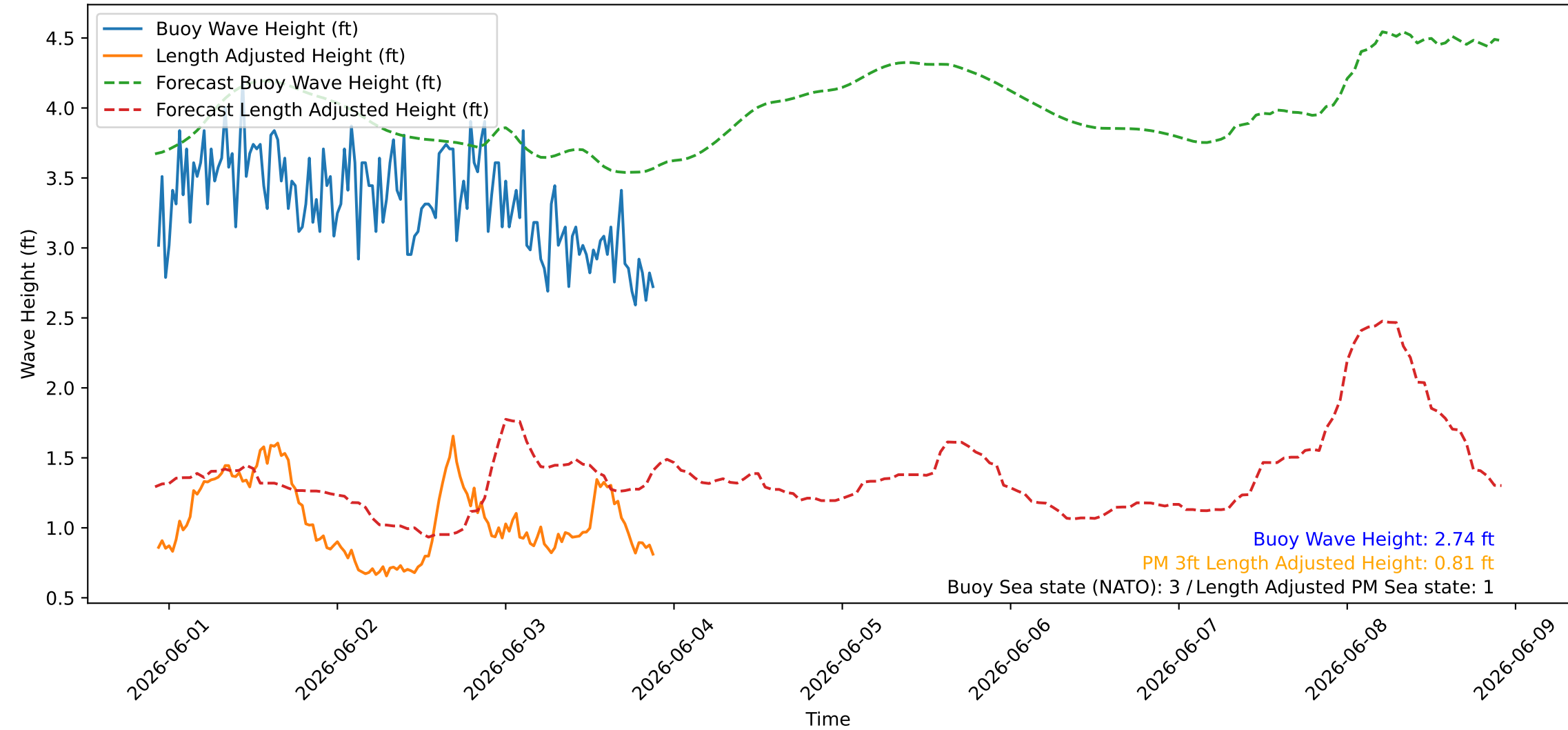
Wave Heights over Time for Red Beach at 2026-06-03 22:00:45
