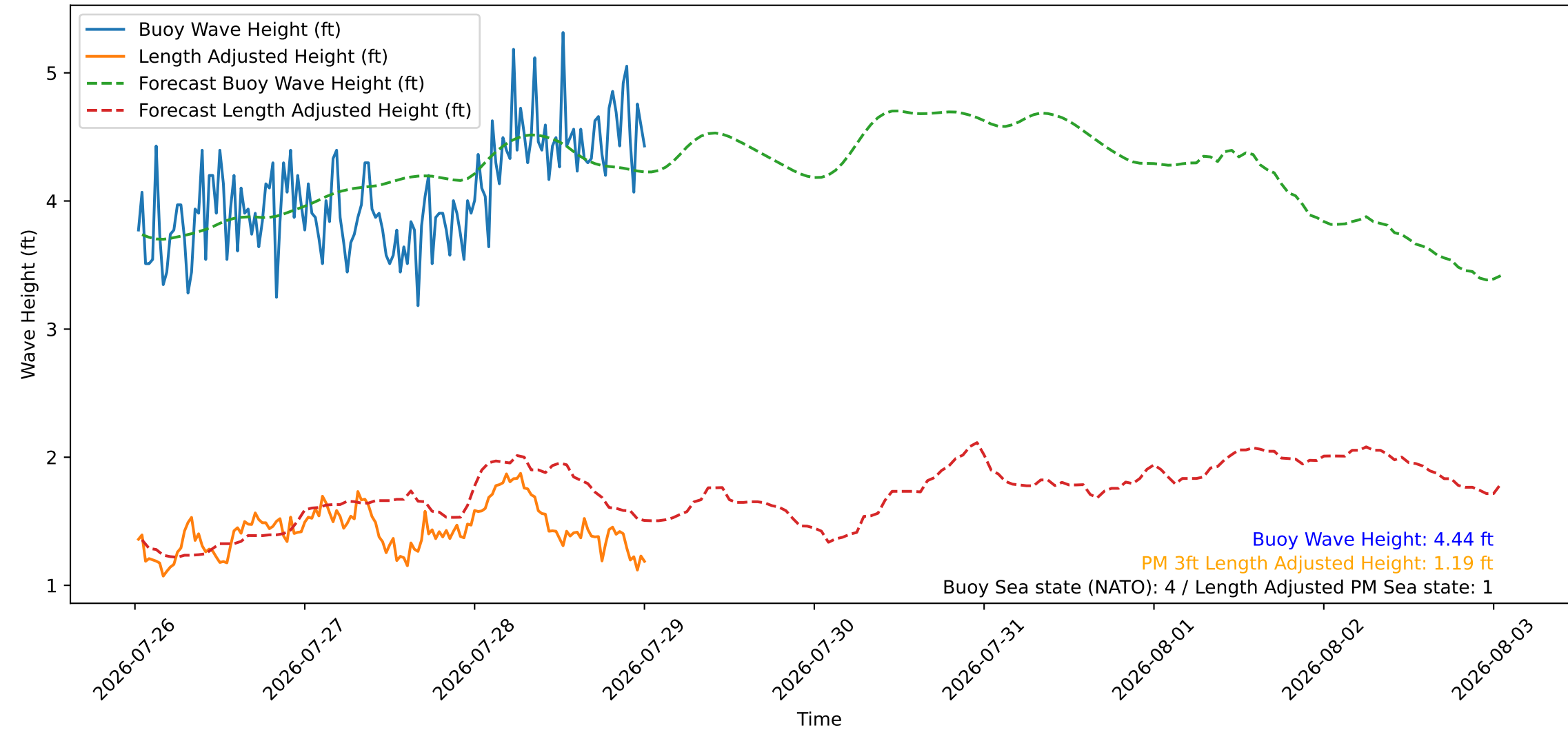
Wave Heights over Time for Oceanside Harbor at 2026-07-29 00:40:27
