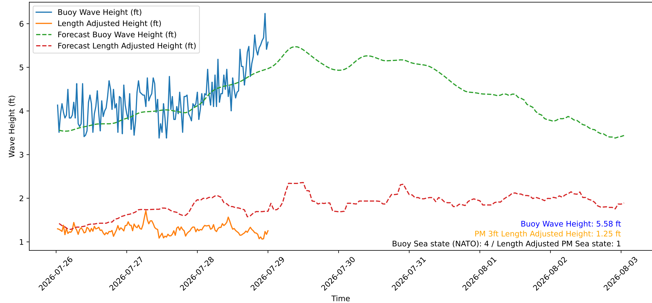
Wave Heights over Time for Green Beach at 2026-07-29 00:41:08
