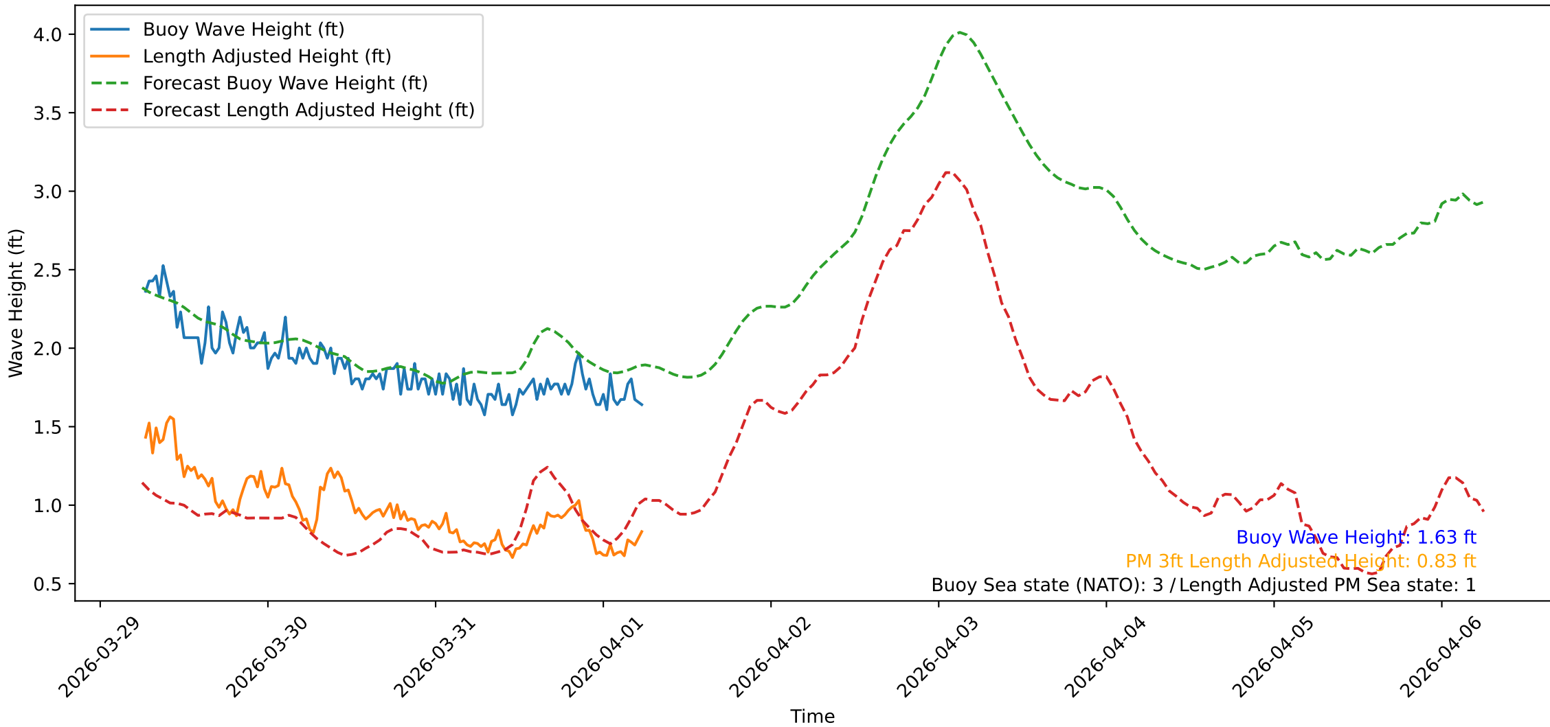
Wave Heights over Time for Oceanside Harbor at 2026-04-01 06:20:31
