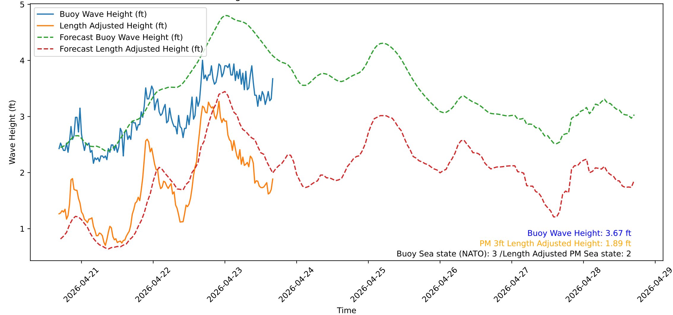
Wave Heights over Time for Green Beach at 2026-04-23 16:41:13
