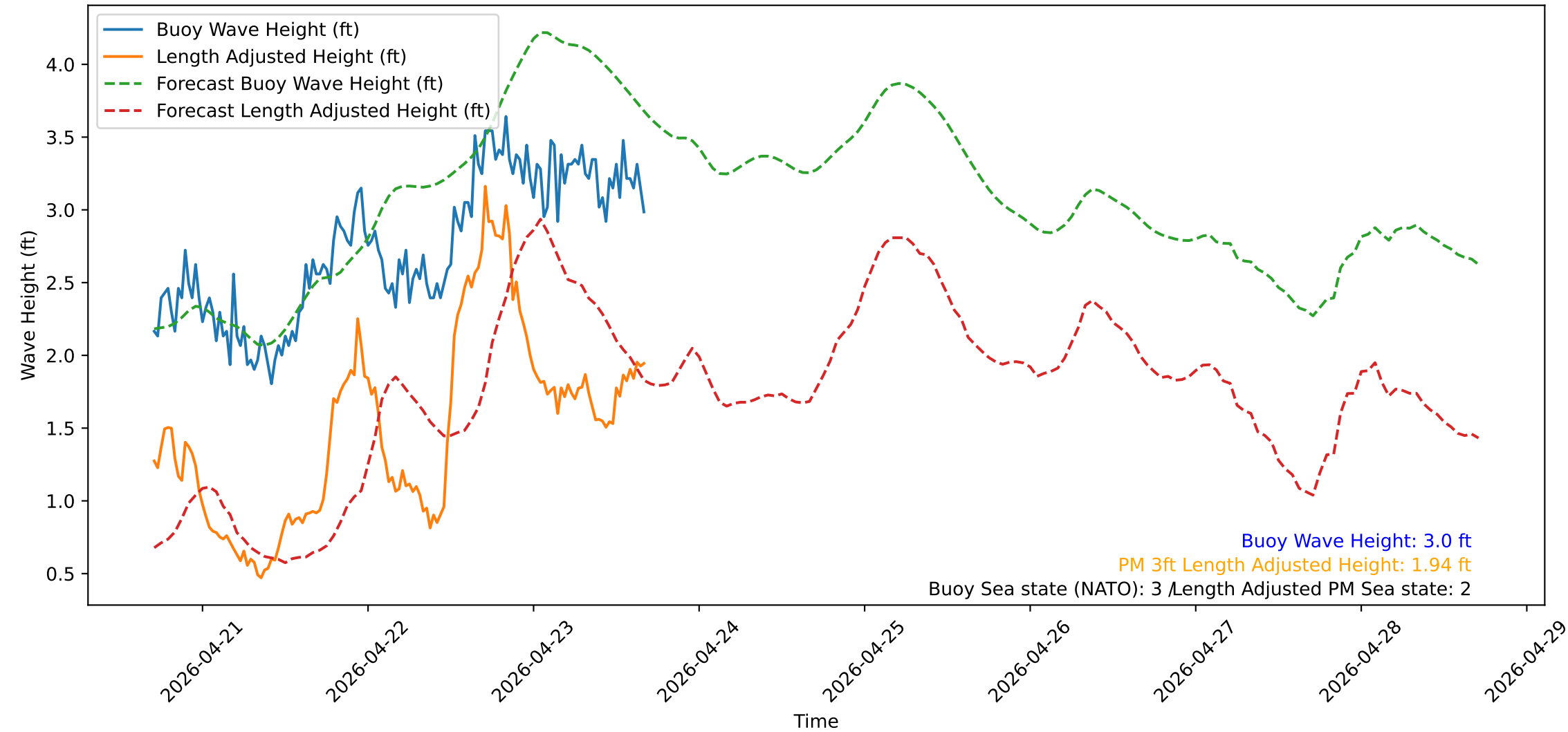
Wave Heights over Time for Red Beach at 2026-04-23 16:40:50
