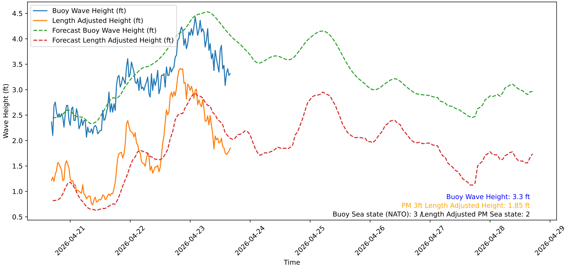
Wave Heights over Time for Oceanside Harbor at 2026-04-23 16:40:31
