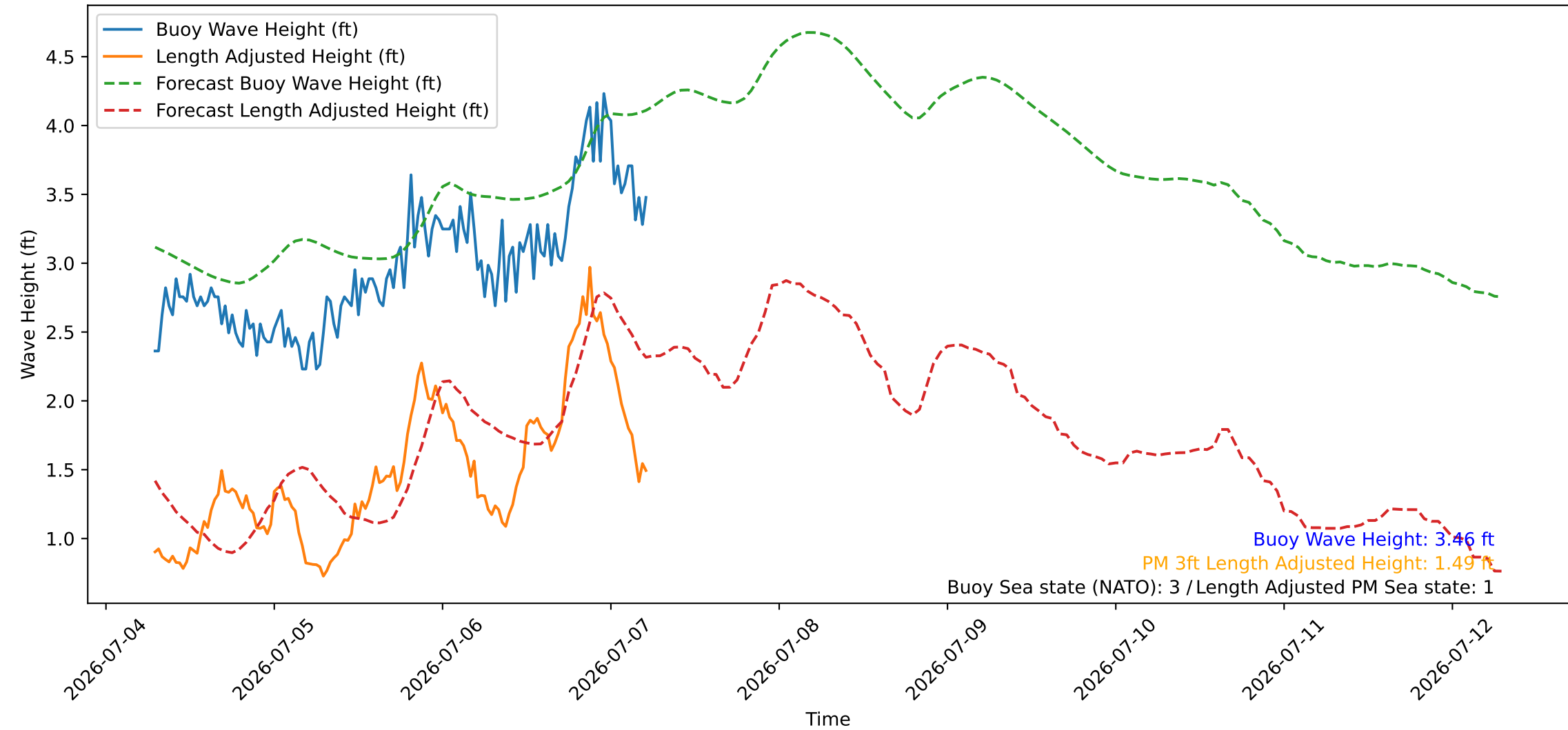
Wave Heights over Time for Red Beach at 2026-07-07 06:30:46
