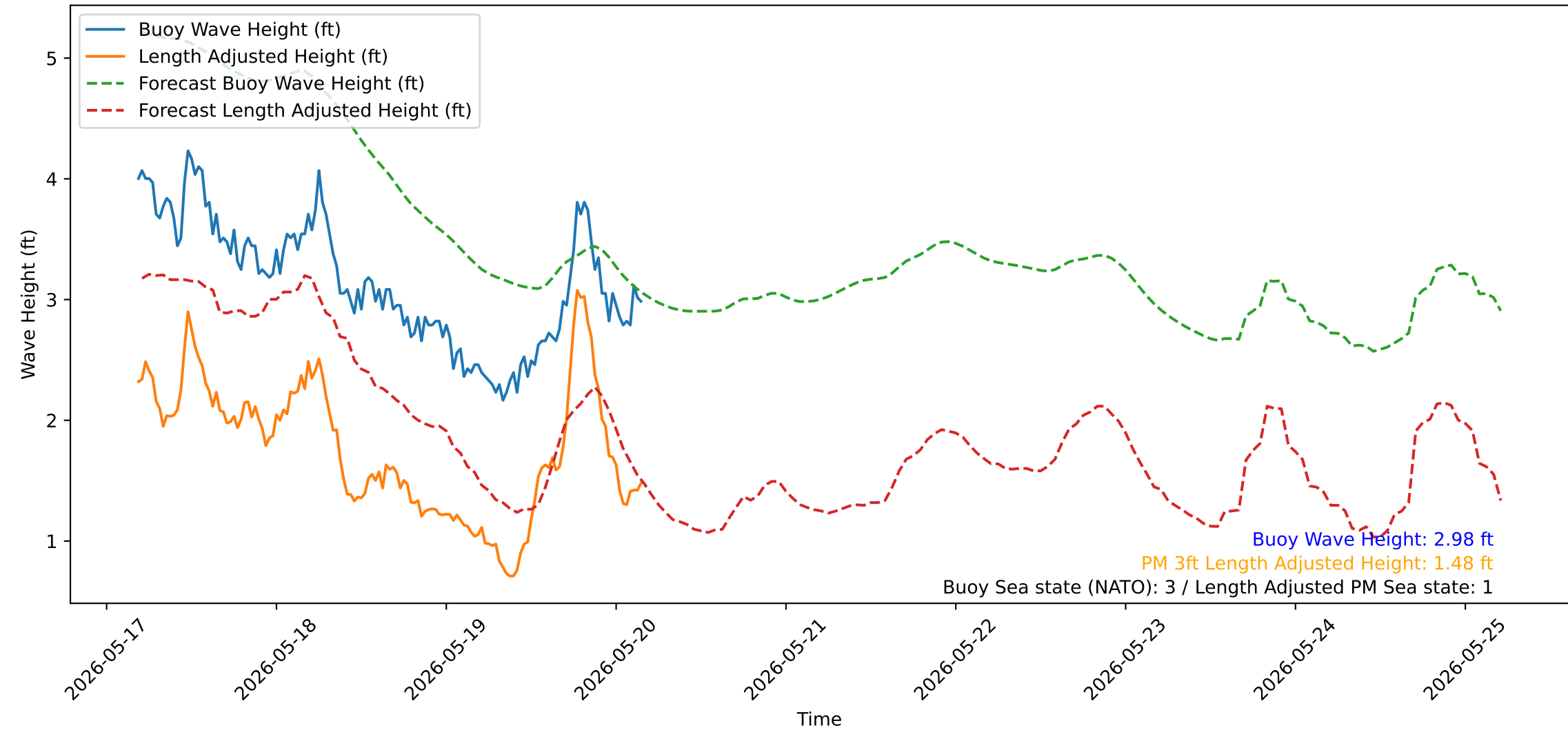
Wave Heights over Time for Green Beach at 2026-05-20 04:41:13
