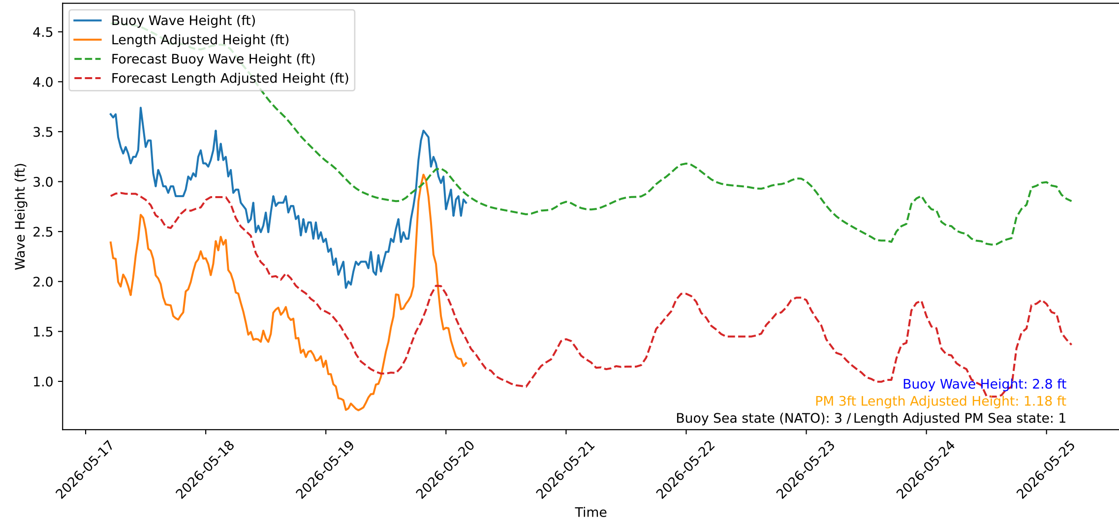
Wave Heights over Time for Red Beach at 2026-05-20 04:40:50
