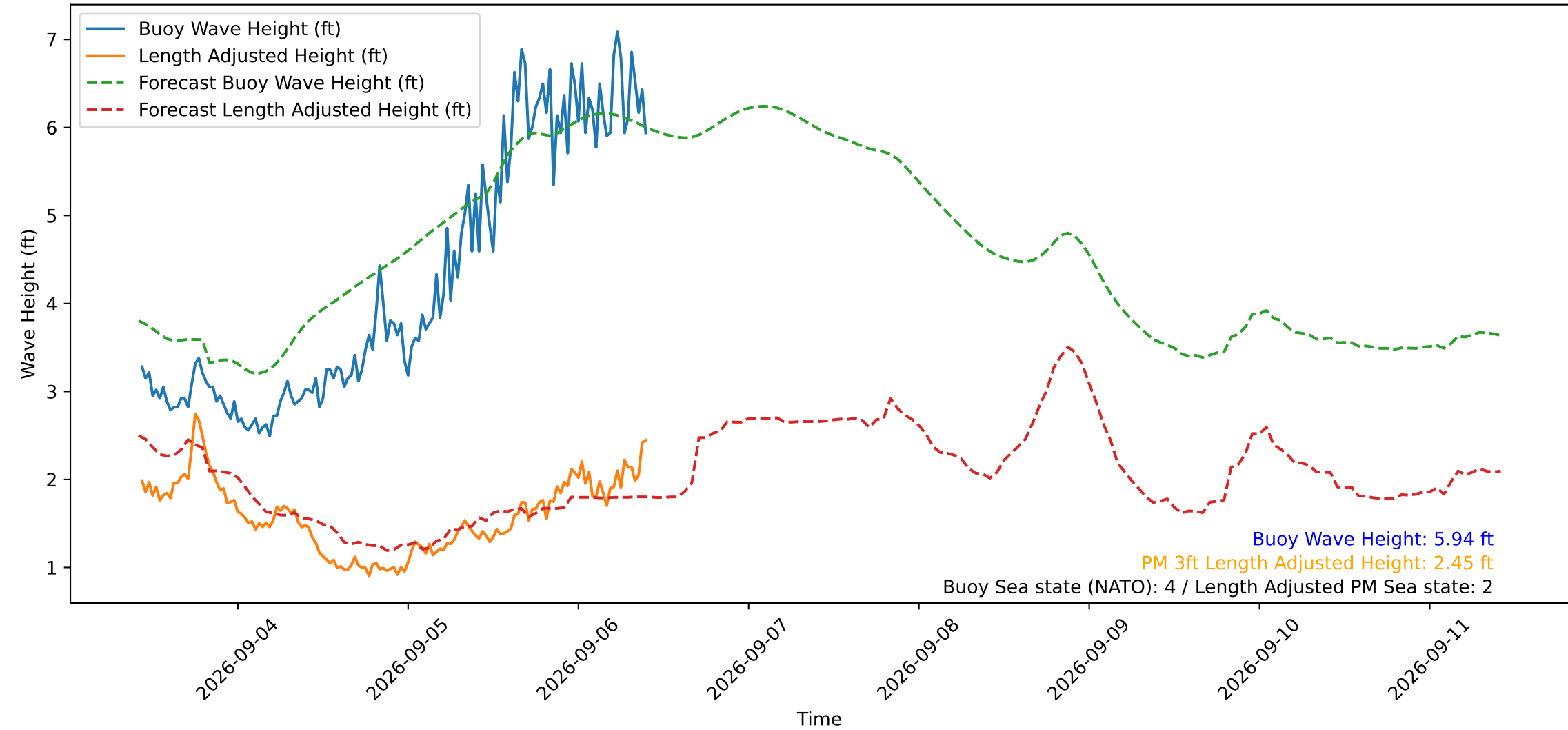
Wave Heights over Time for Green Beach at 2026-09-06 10:11:11
