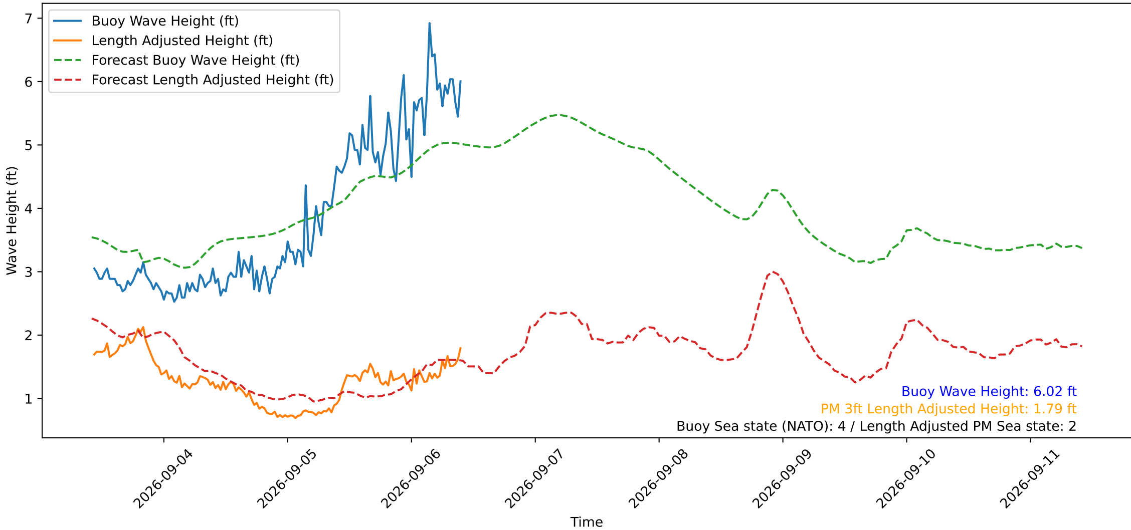
Wave Heights over Time for Red Beach at 2026-09-06 10:10:49
