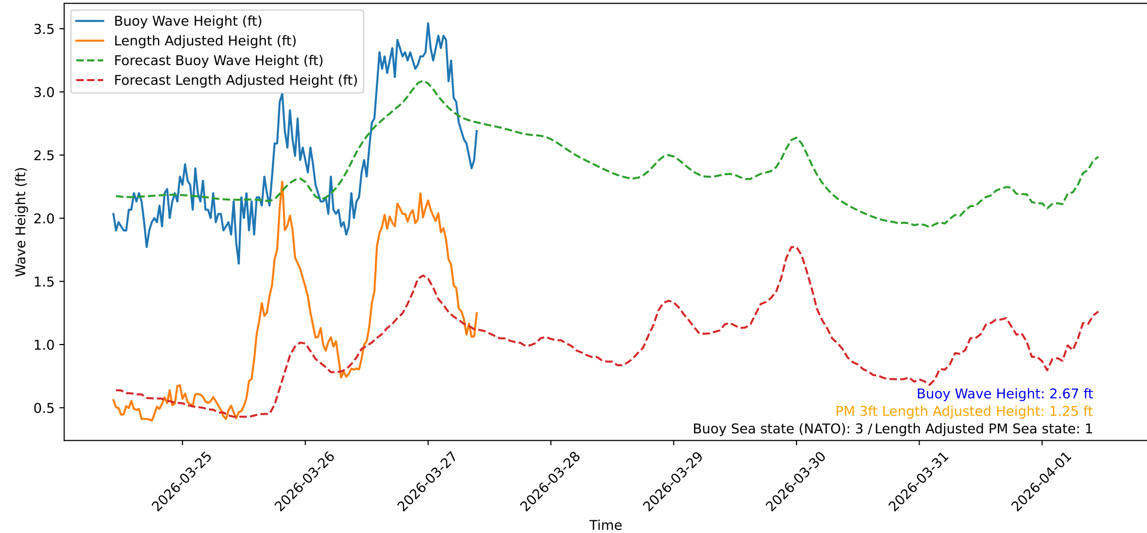
Wave Heights over Time for Green Beach at 2026-03-27 10:31:10
