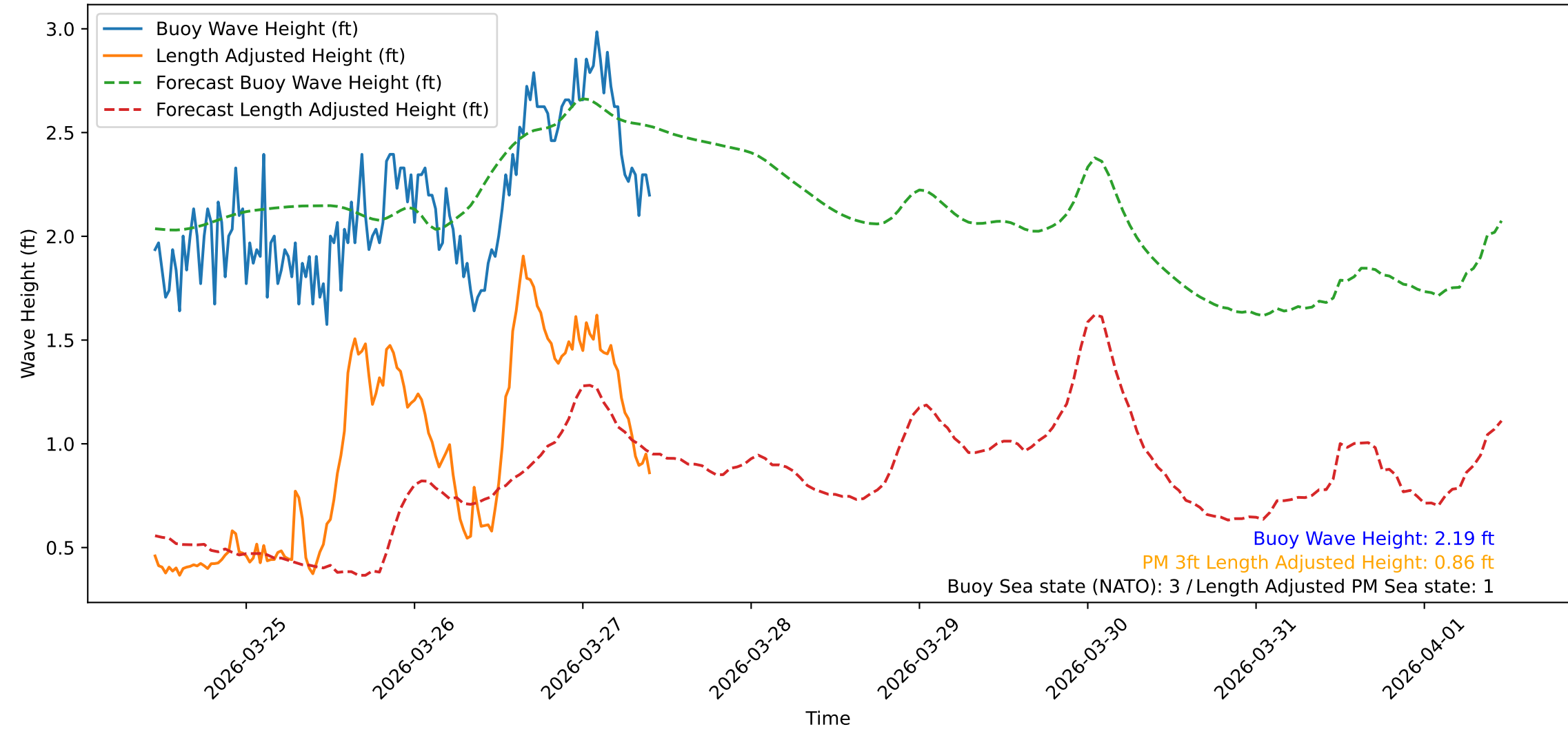
Wave Heights over Time for Red Beach at 2026-03-27 10:30:48
