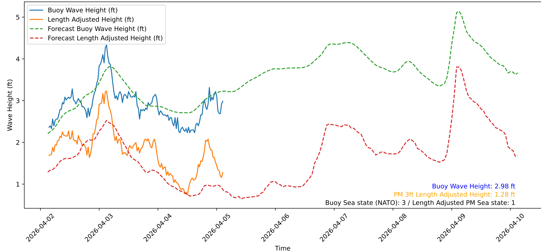
Wave Heights over Time for Green Beach at 2026-04-05 03:21:09
