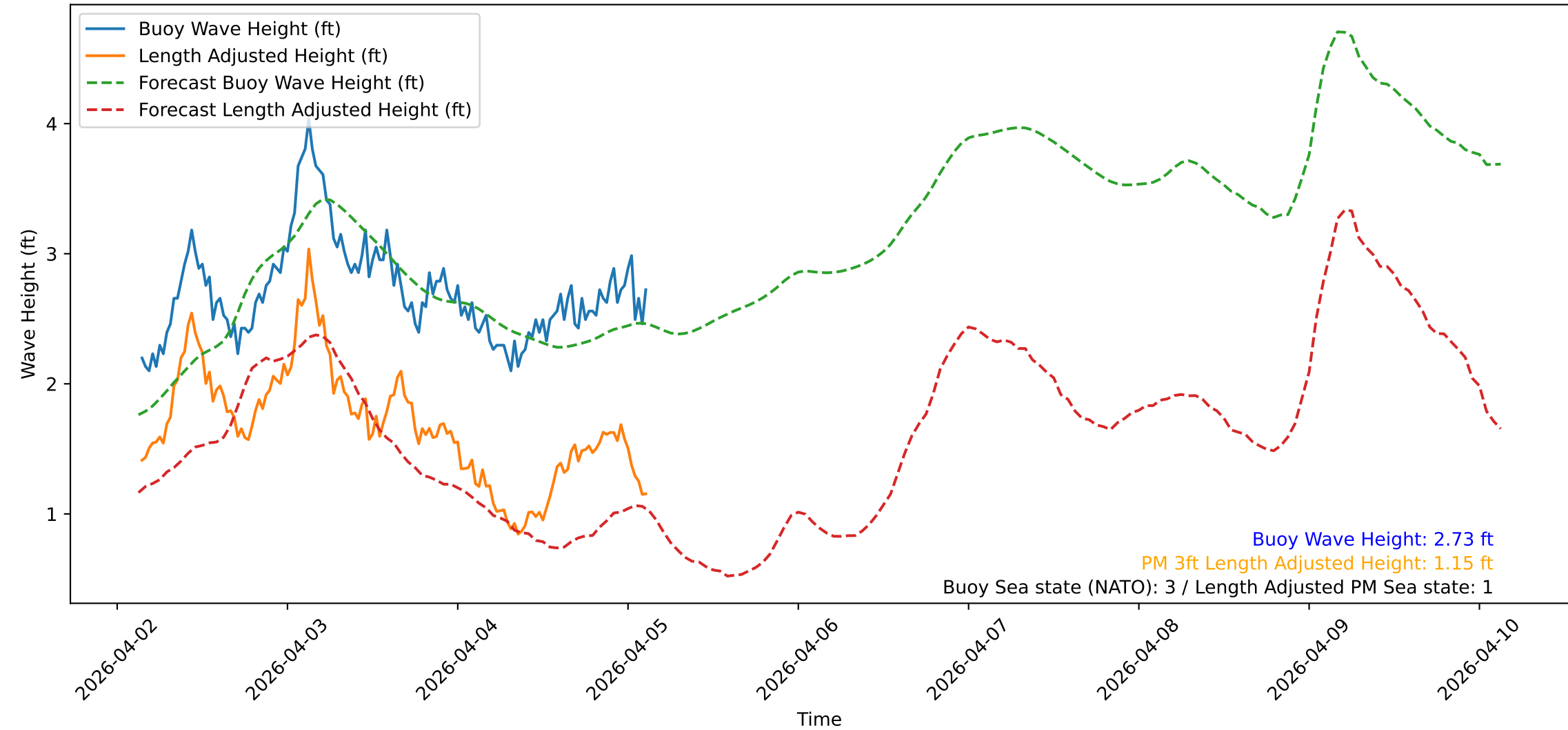
Wave Heights over Time for Oceanside Harbor at 2026-04-05 03:20:31
