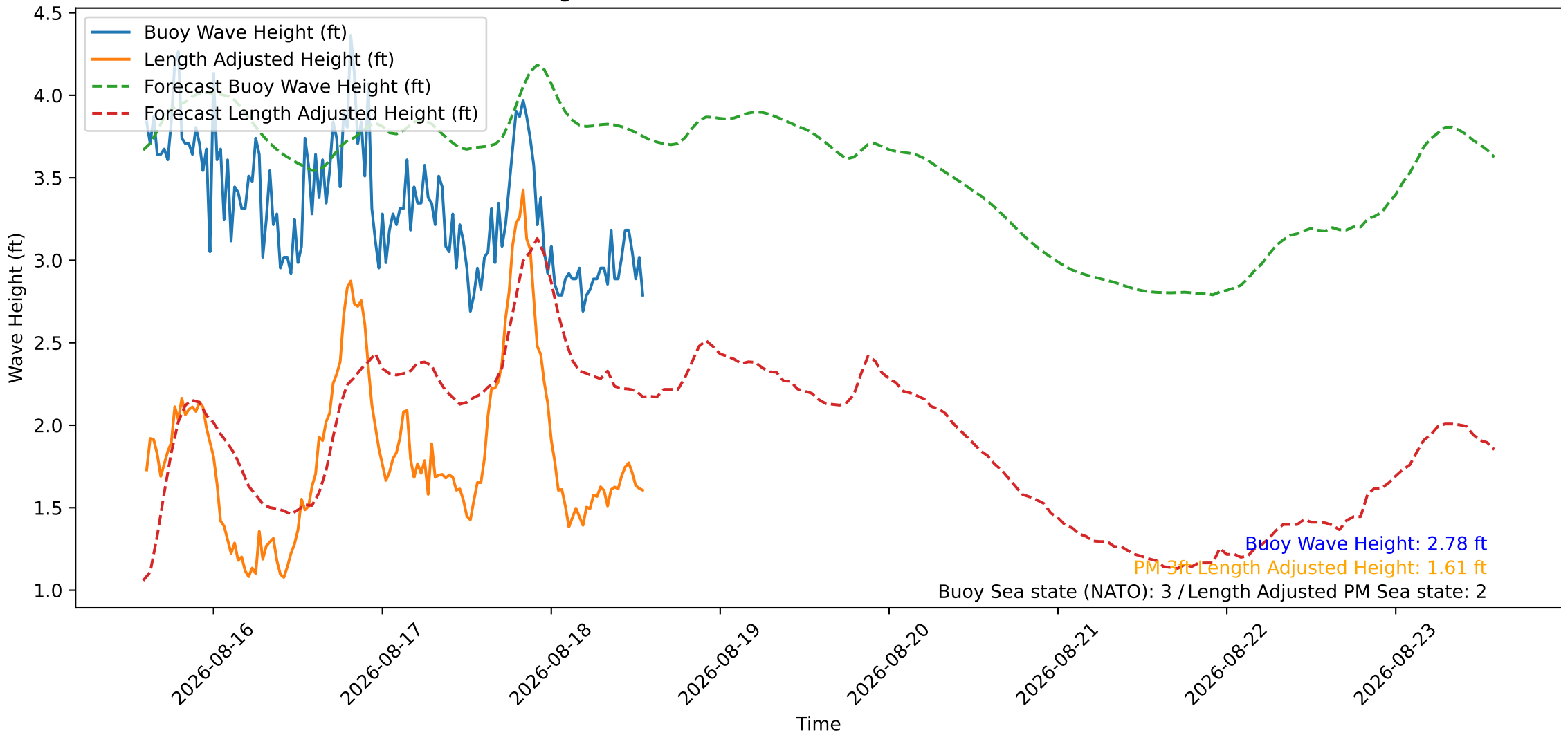
Wave Heights over Time for Green Beach at 2026-08-18 14:01:08
