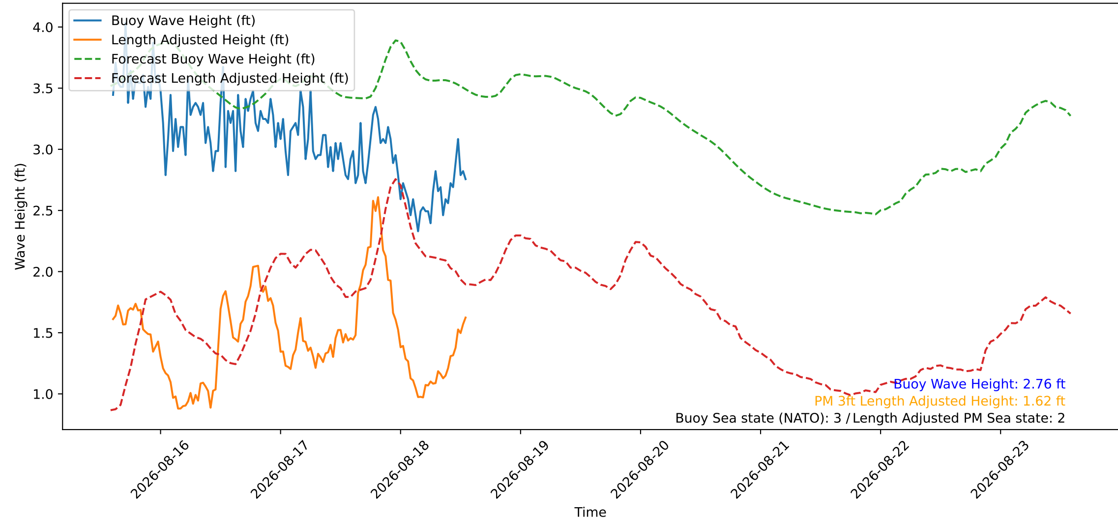
Wave Heights over Time for Red Beach at 2026-08-18 14:00:46
