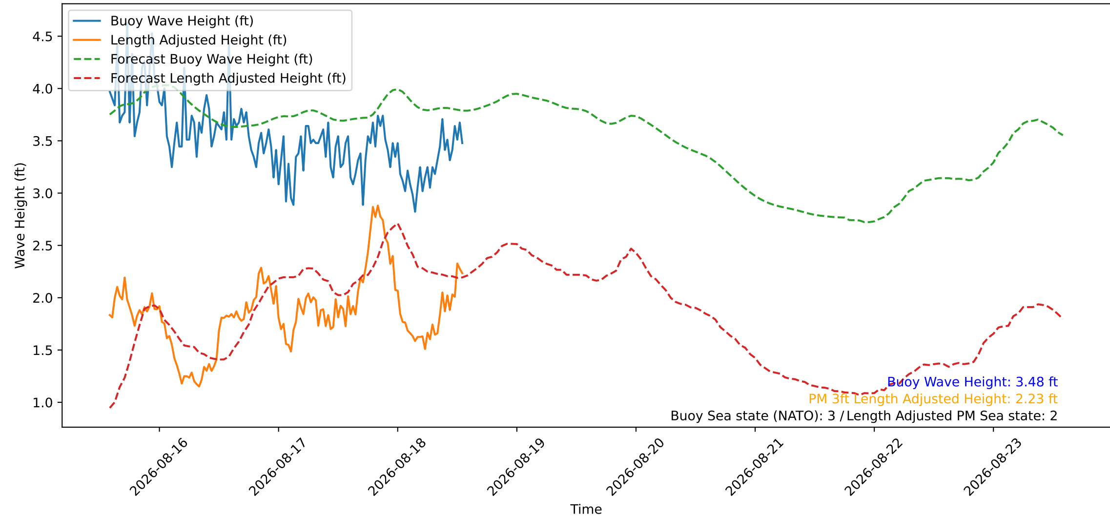
Wave Heights over Time for Oceanside Harbor at 2026-08-18 14:00:26
