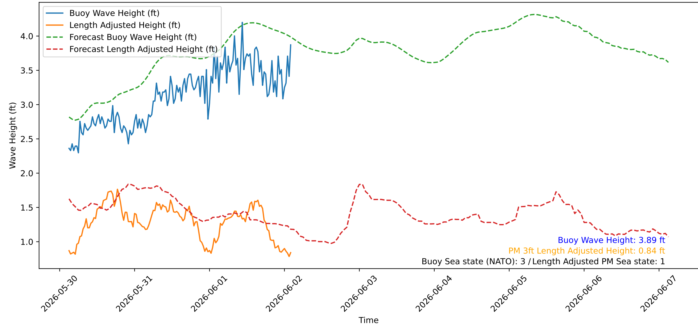
Wave Heights over Time for Red Beach at 2026-06-02 02:50:47
