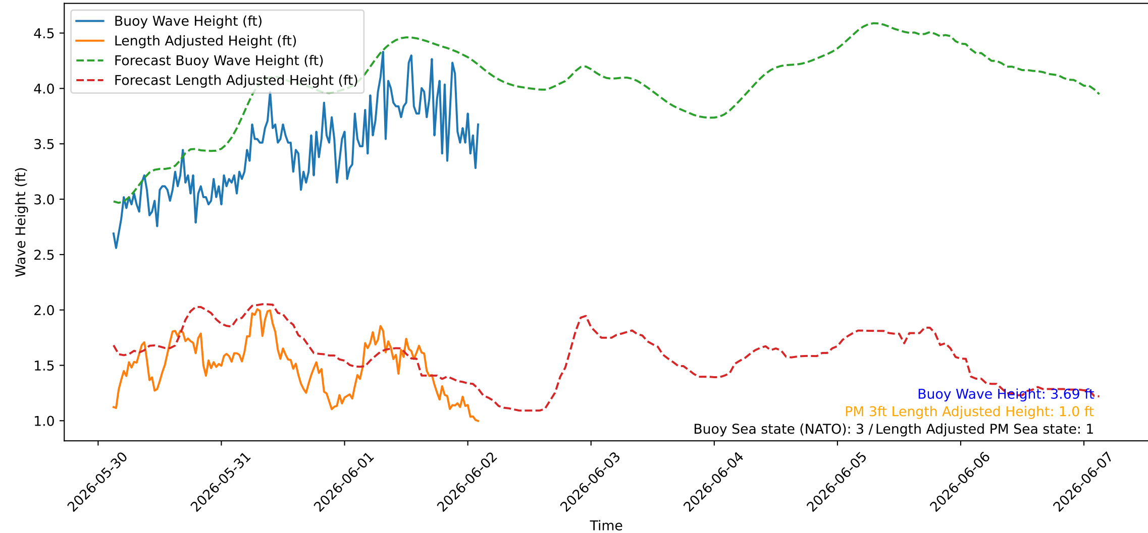
Wave Heights over Time for Green Beach at 2026-06-02 02:51:09
