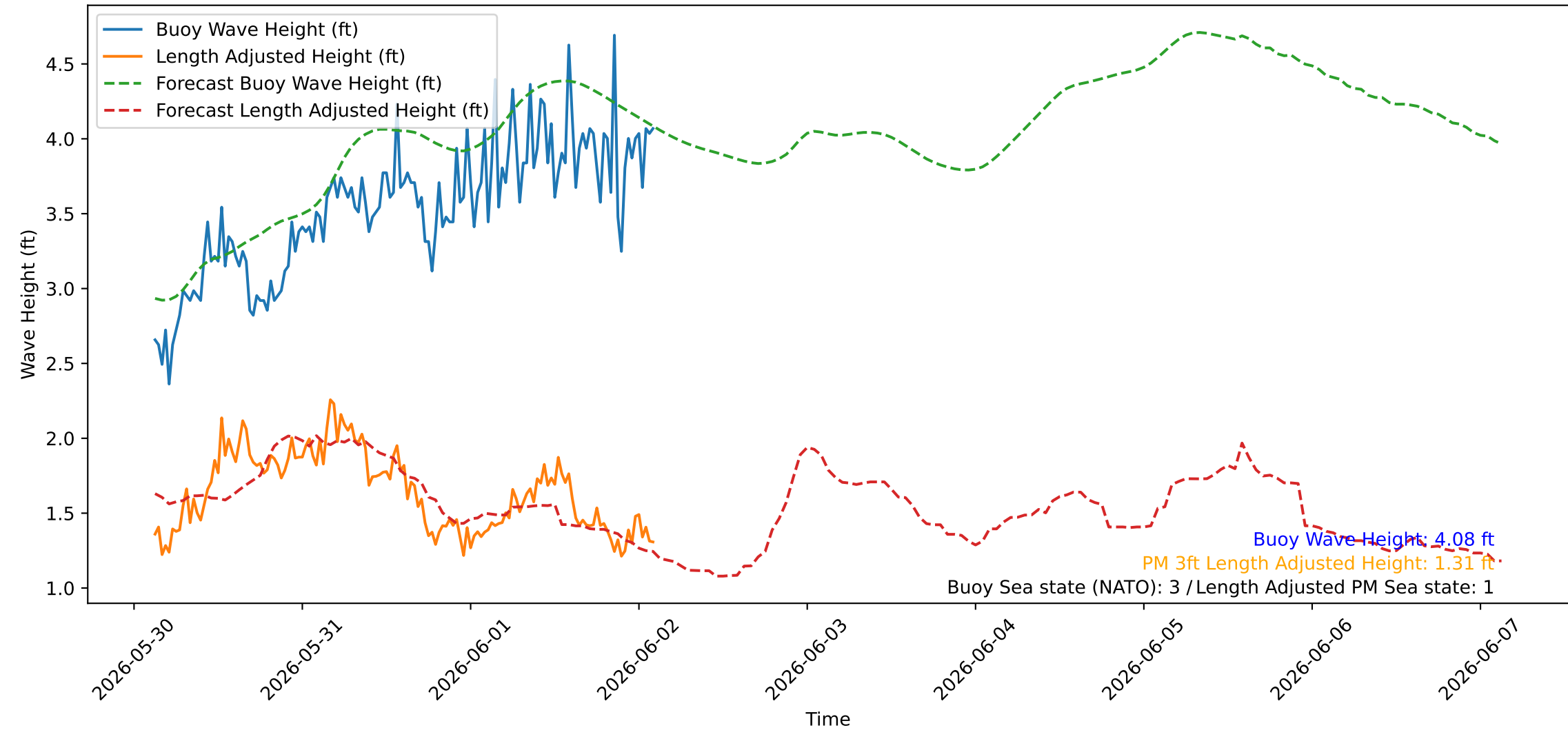
Wave Heights over Time for Oceanside Harbor at 2026-06-02 02:50:26
