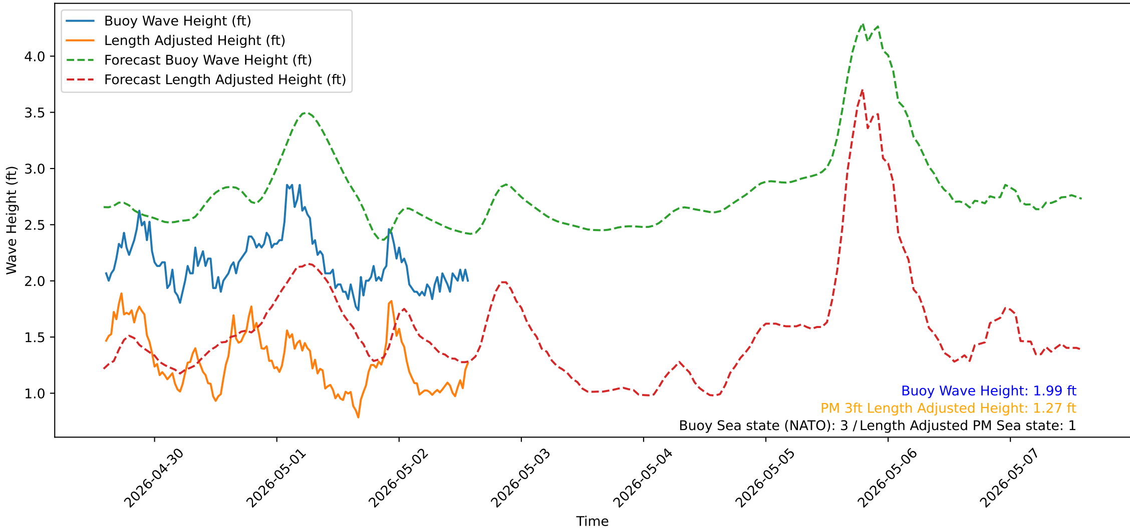
Wave Heights over Time for Green Beach at 2026-05-02 14:21:15
