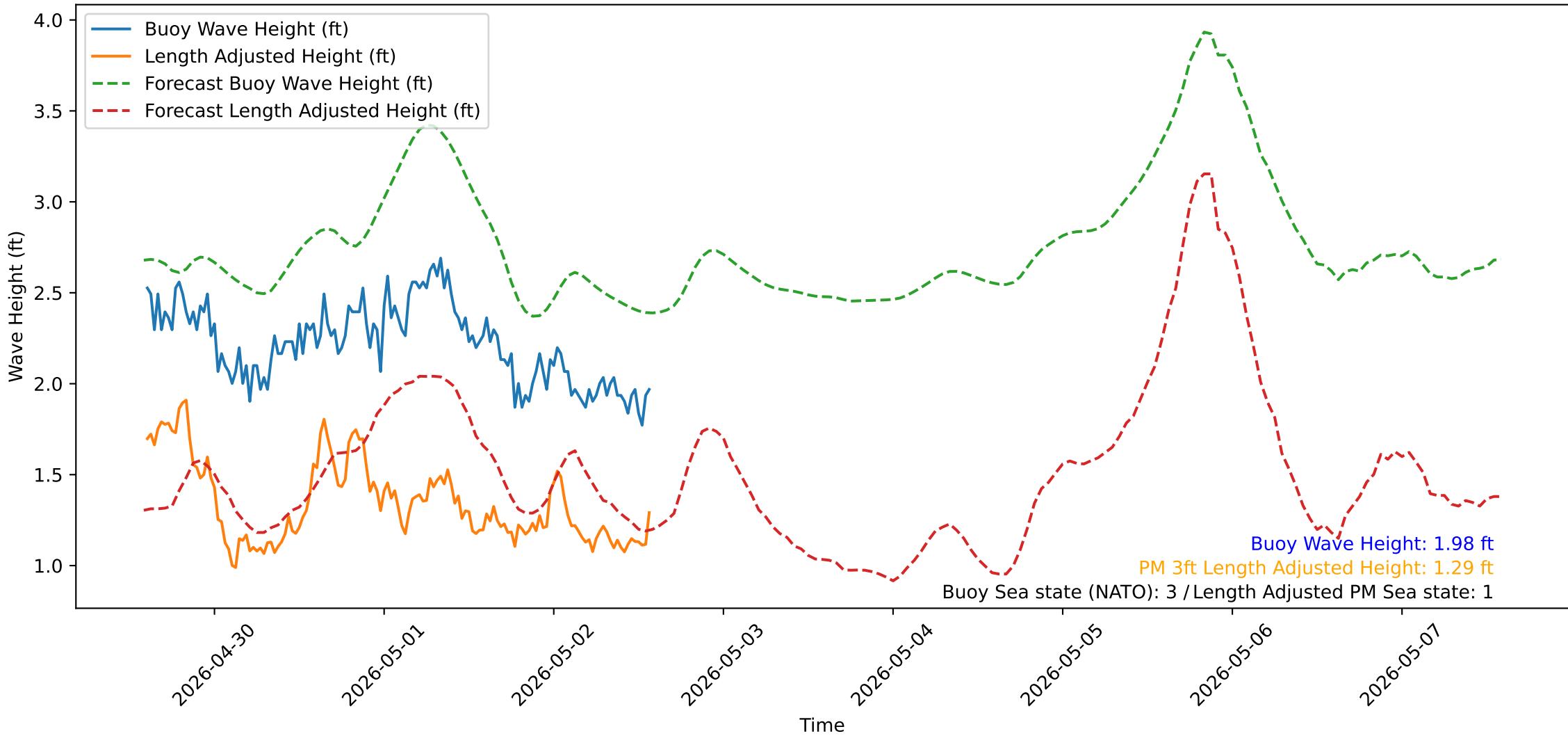
Wave Heights over Time for Oceanside Harbor at 2026-05-02 14:20:32
