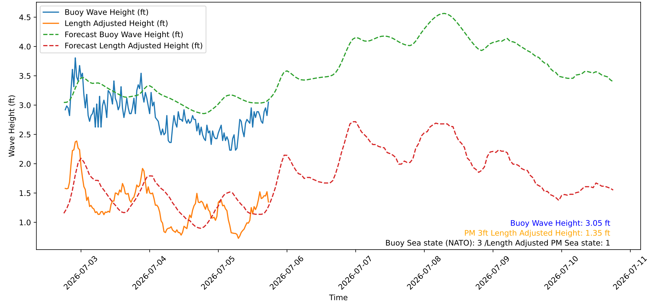
Wave Heights over Time for Red Beach at 2026-07-05 18:10:46
