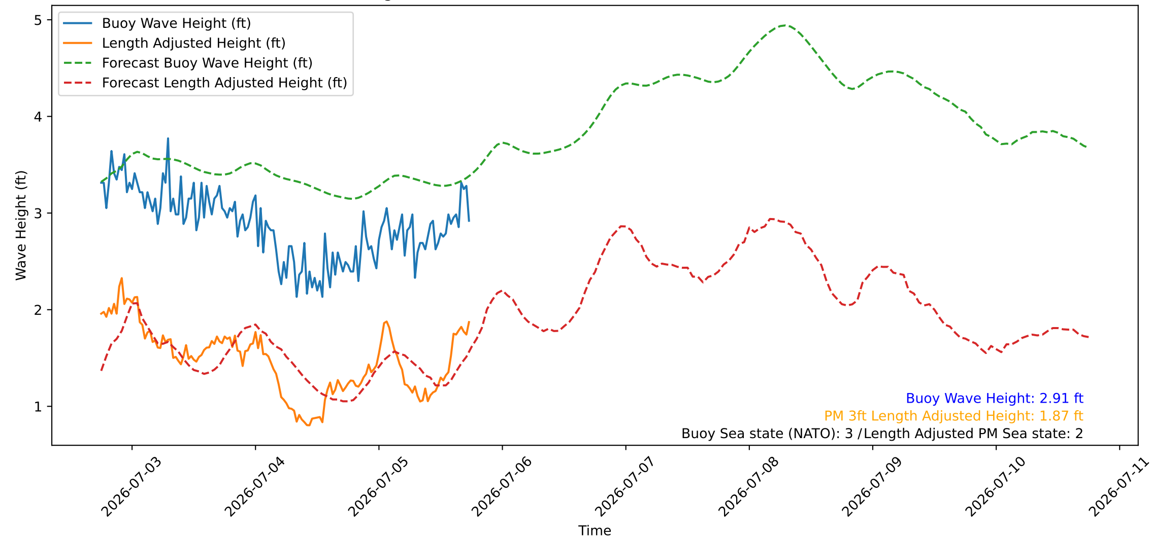
Wave Heights over Time for Oceanside Harbor at 2026-07-05 18:10:26
