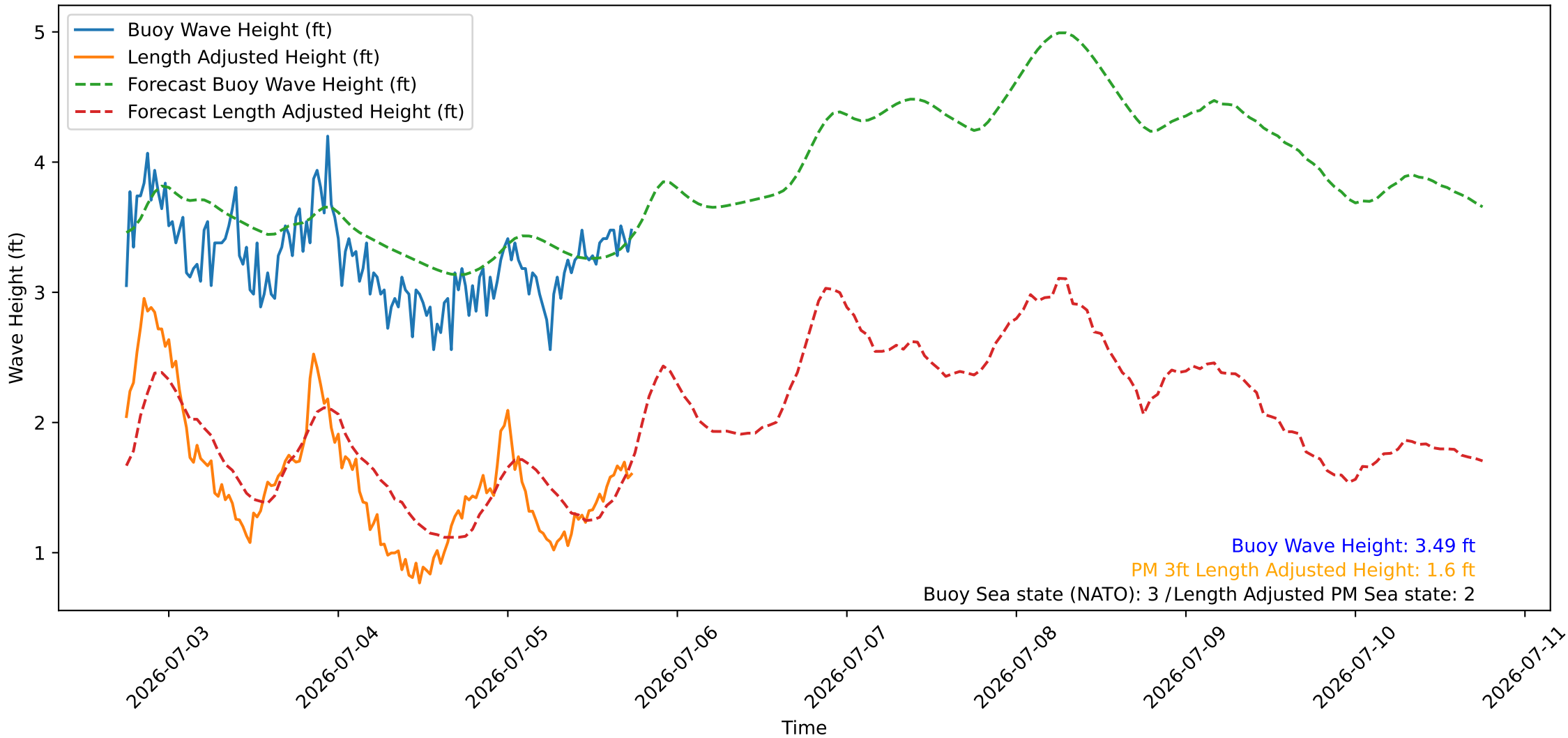
Wave Heights over Time for Green Beach at 2026-07-05 18:11:08
