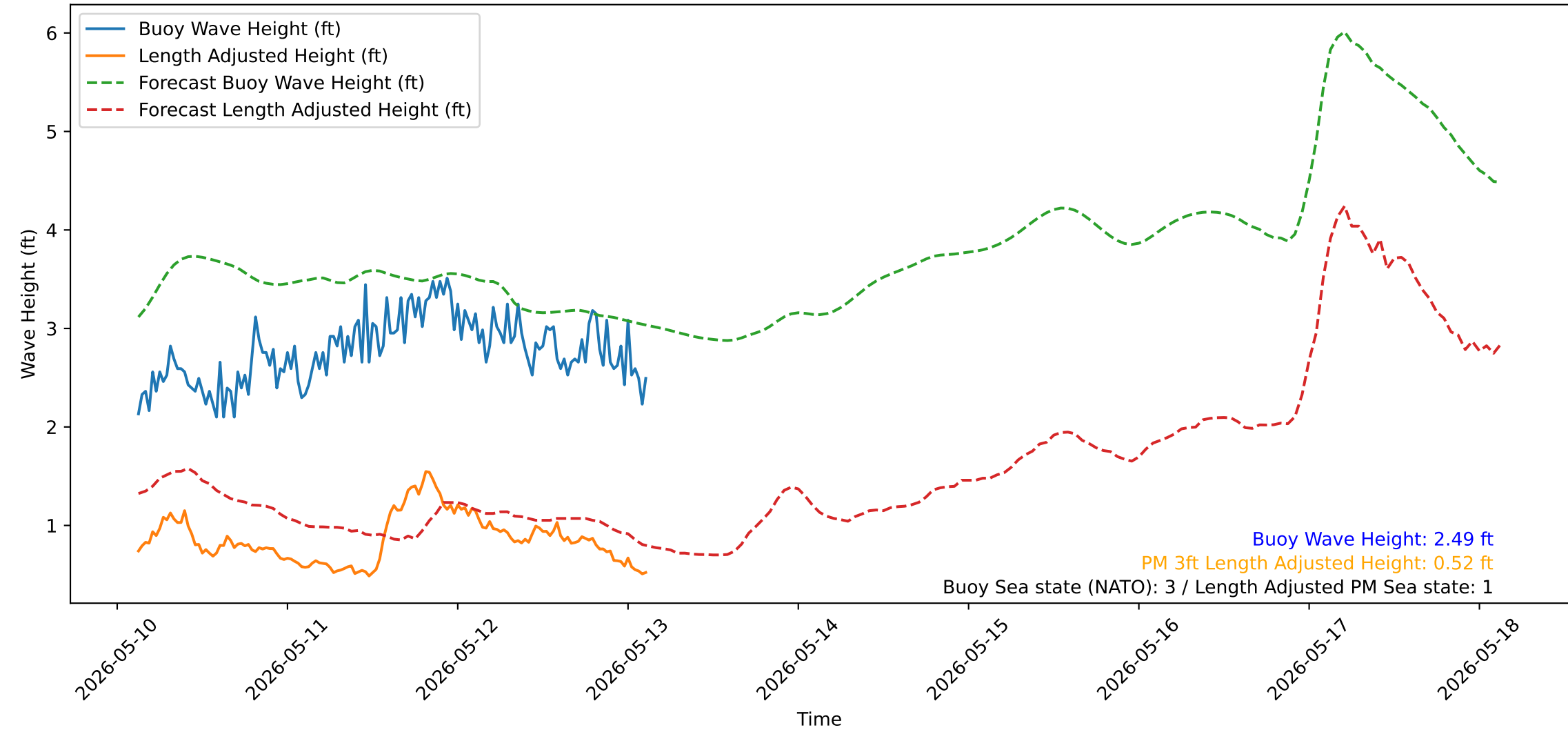
Wave Heights over Time for Green Beach at 2026-05-13 03:11:13
