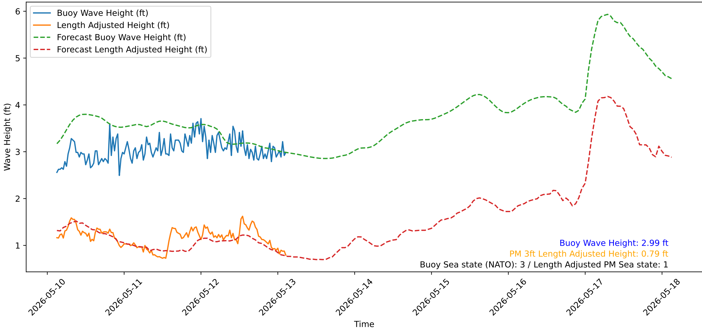
Wave Heights over Time for Oceanside Harbor at 2026-05-13 03:10:32
