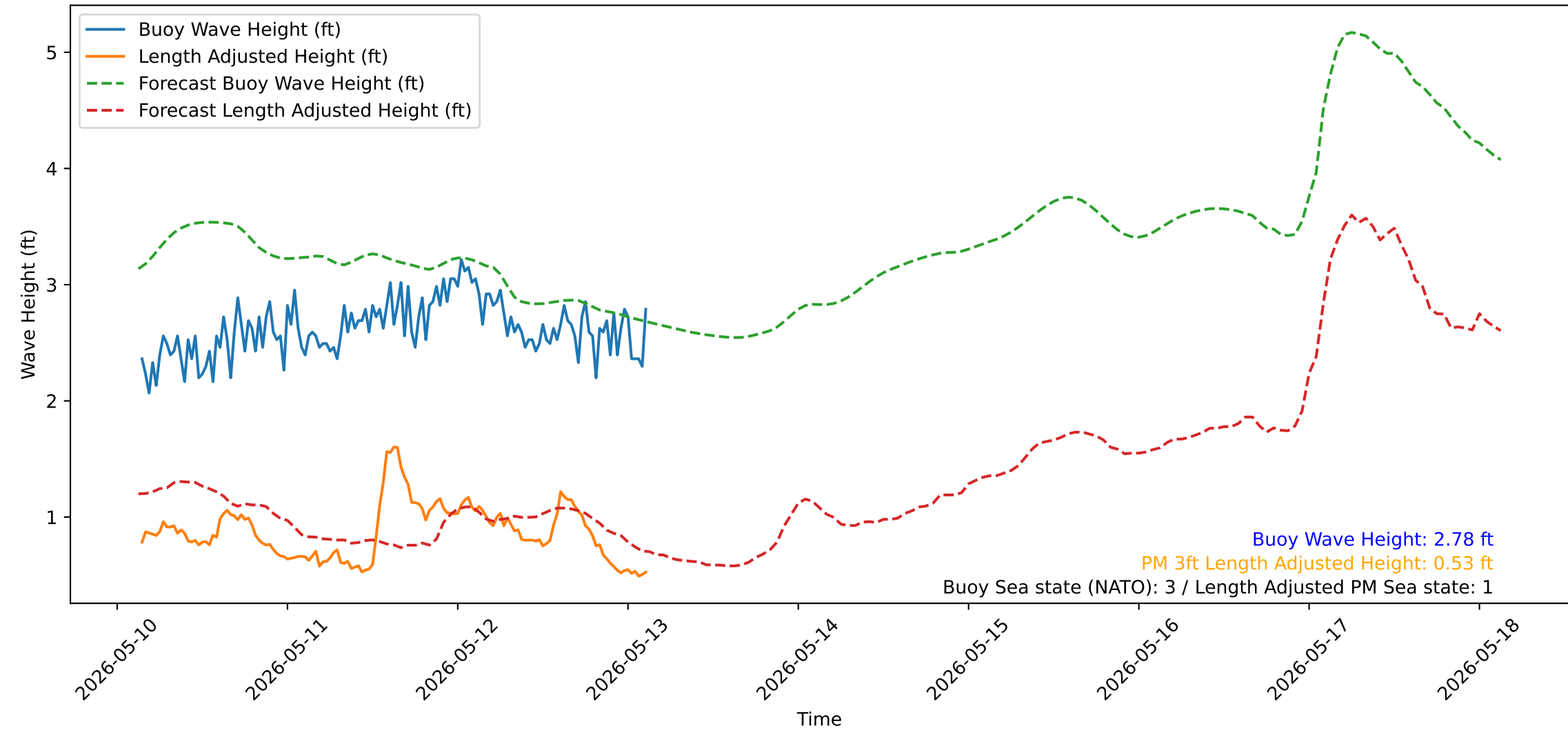
Wave Heights over Time for Red Beach at 2026-05-13 03:10:51
