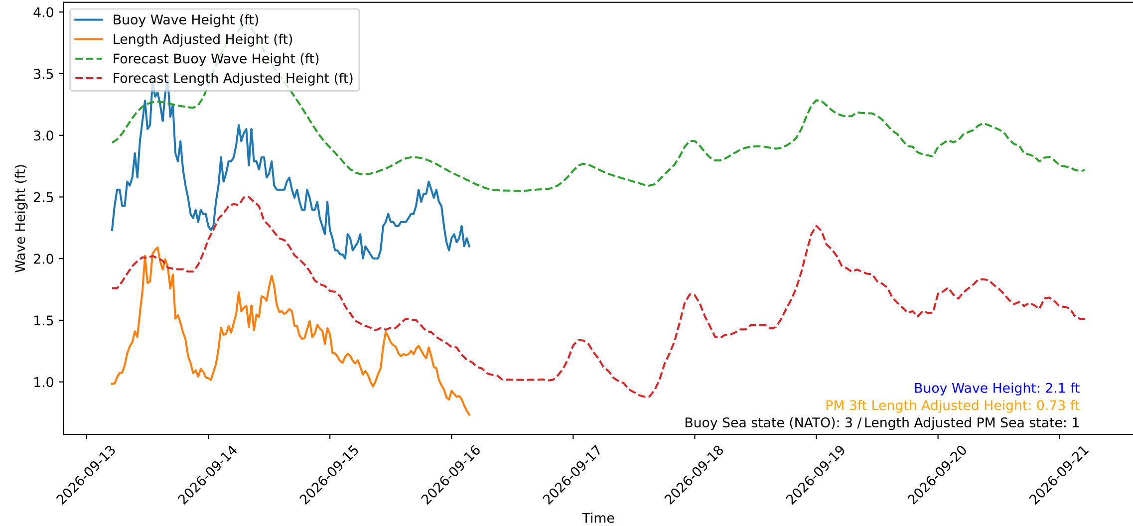
Wave Heights over Time for Red Beach at 2026-09-16 04:30:49
