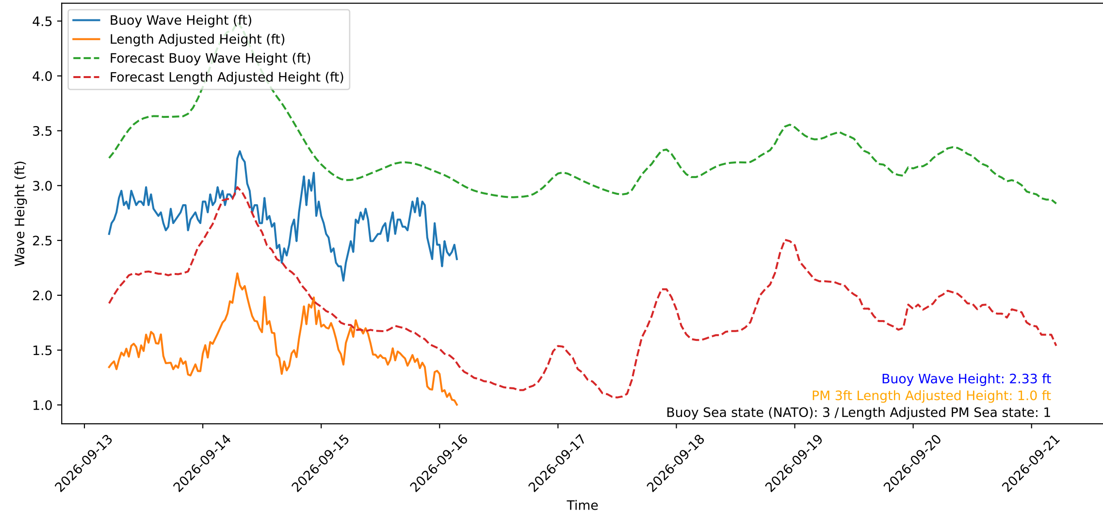
Wave Heights over Time for Green Beach at 2026-09-16 04:31:11
