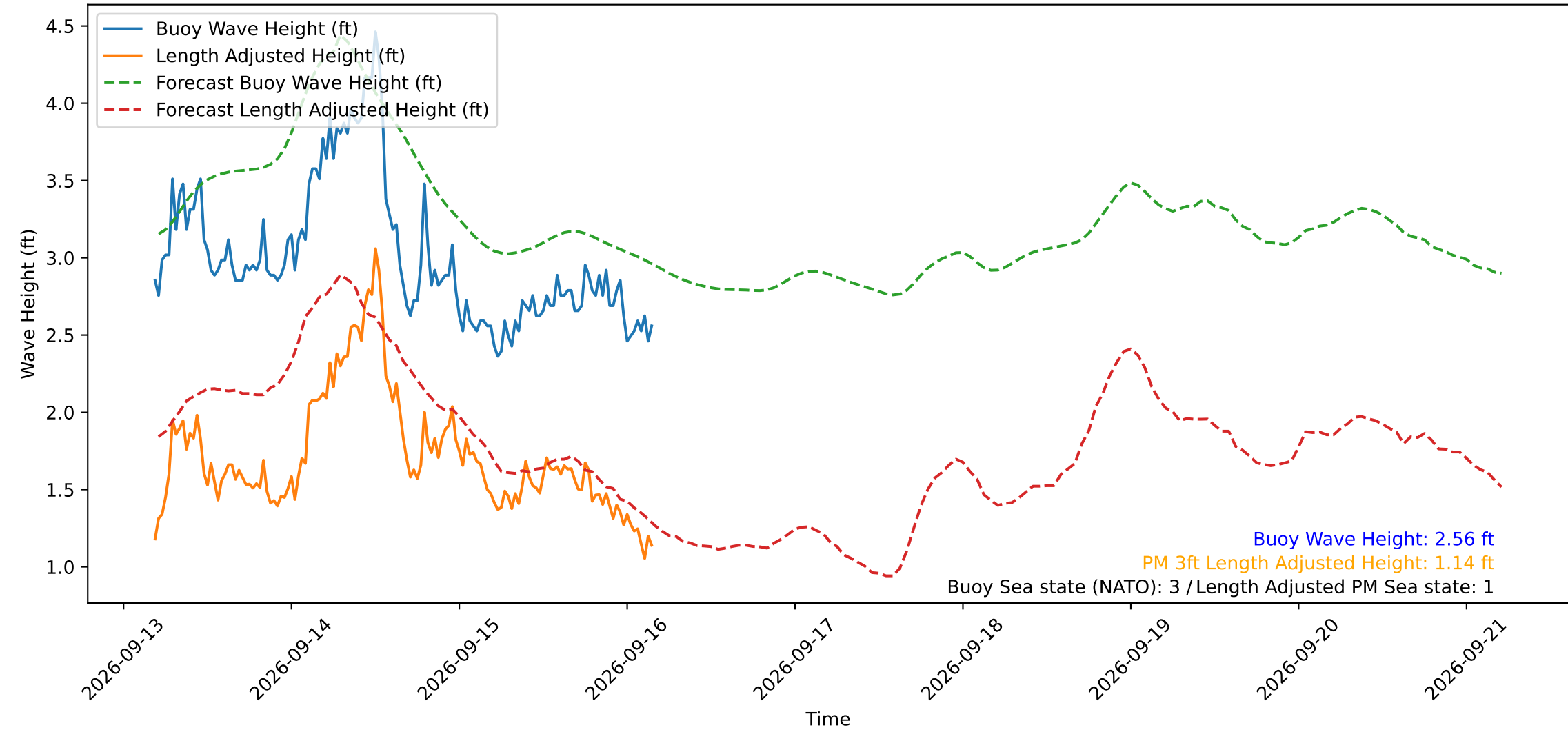
Wave Heights over Time for Oceanside Harbor at 2026-09-16 04:30:30
