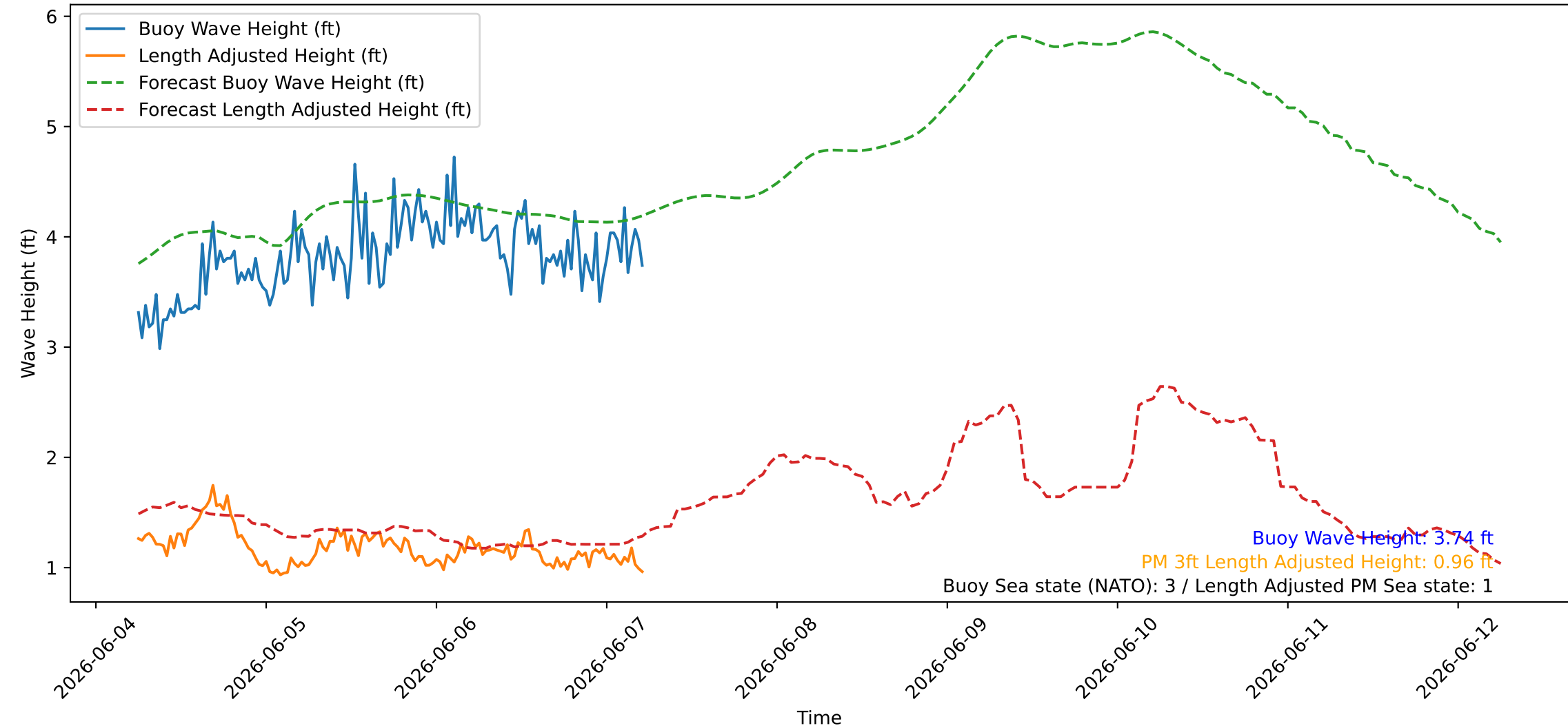
Wave Heights over Time for Green Beach at 2026-06-07 05:51:09
