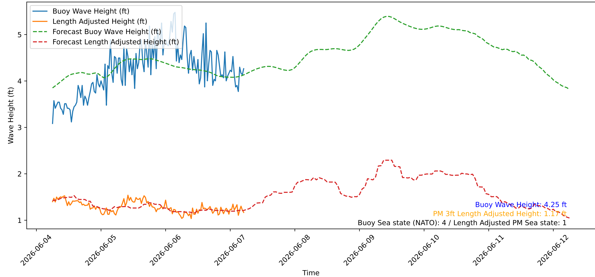
Wave Heights over Time for Oceanside Harbor at 2026-06-07 05:50:26
