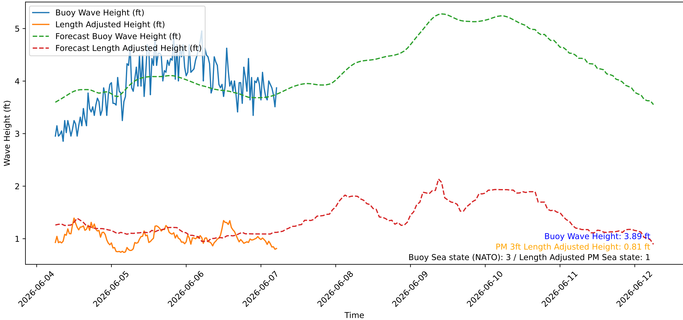
Wave Heights over Time for Red Beach at 2026-06-07 05:50:46
