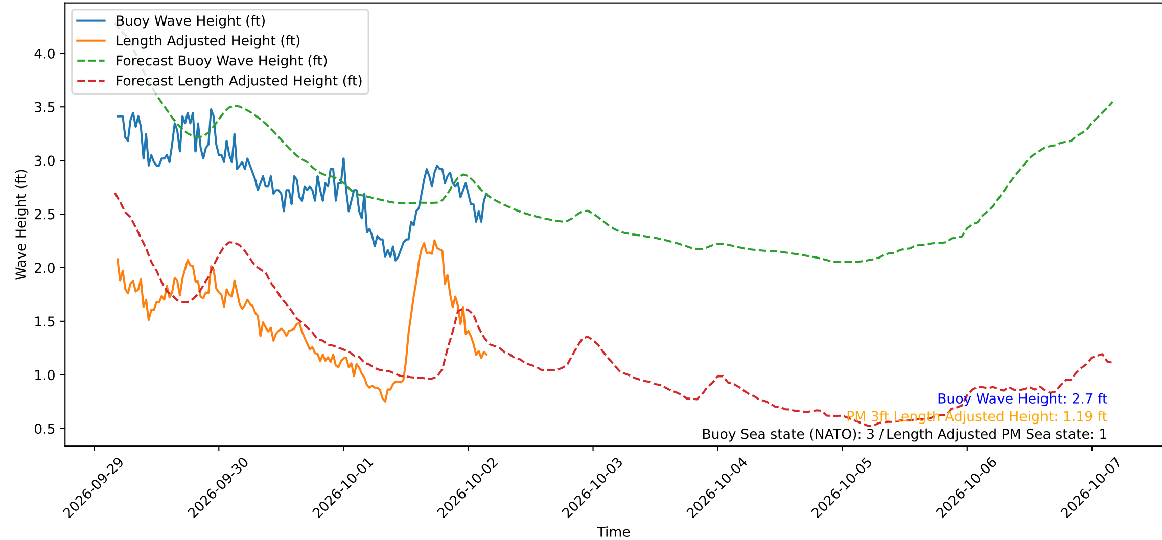
Wave Heights over Time for Red Beach at 2026-10-02 04:20:51
