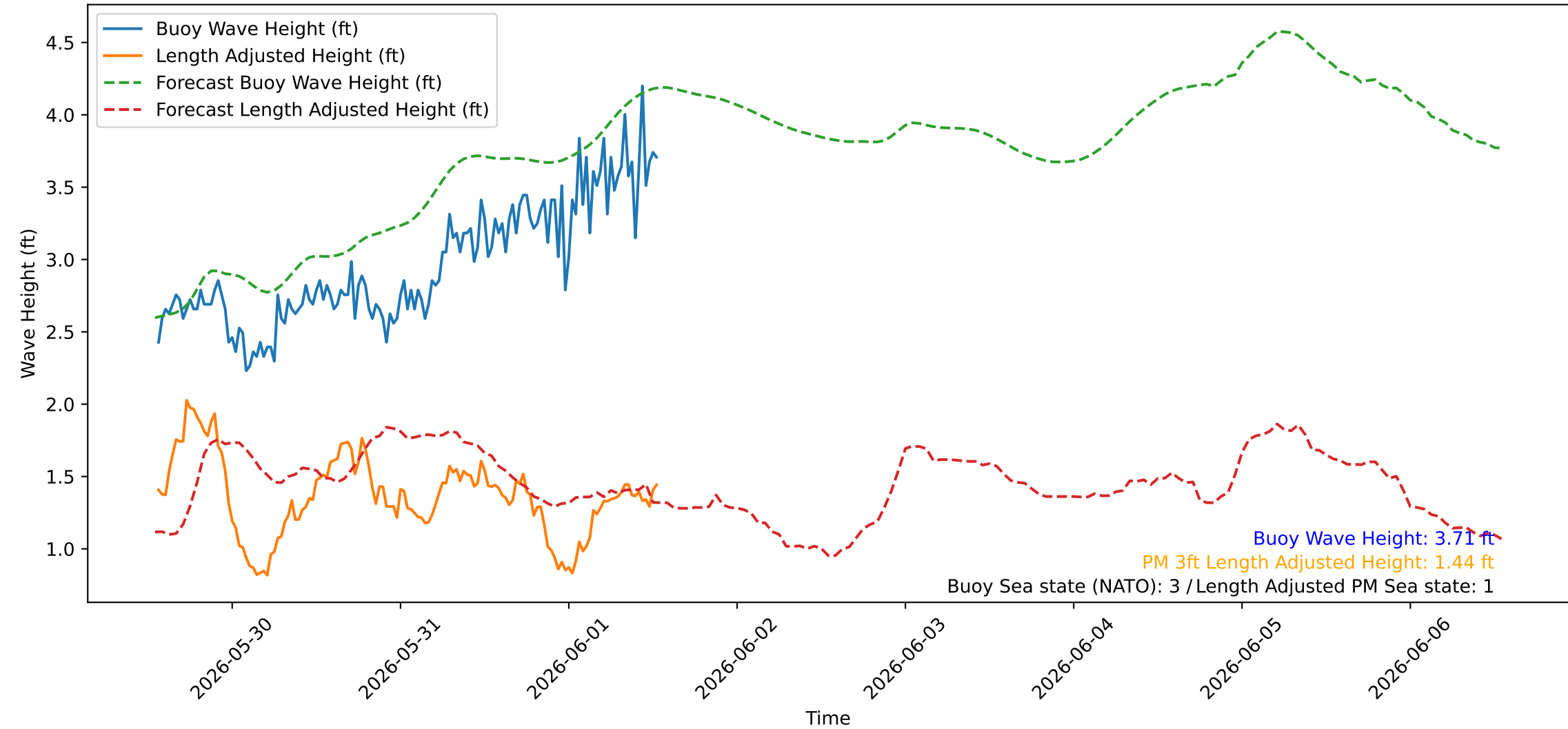
Wave Heights over Time for Red Beach at 2026-06-01 13:20:47
