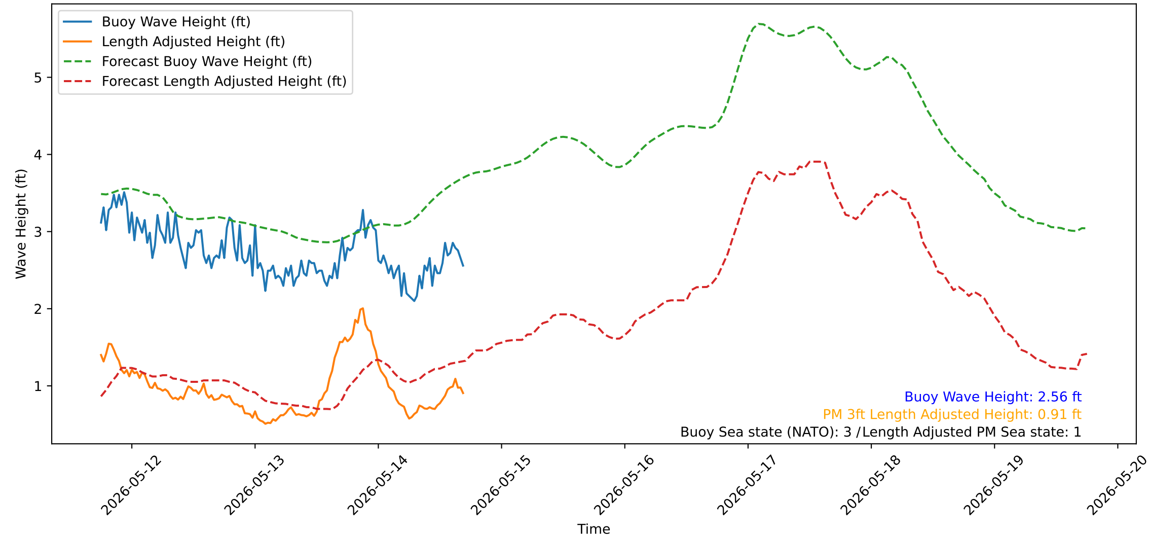
Wave Heights over Time for Green Beach at 2026-05-14 17:51:15
