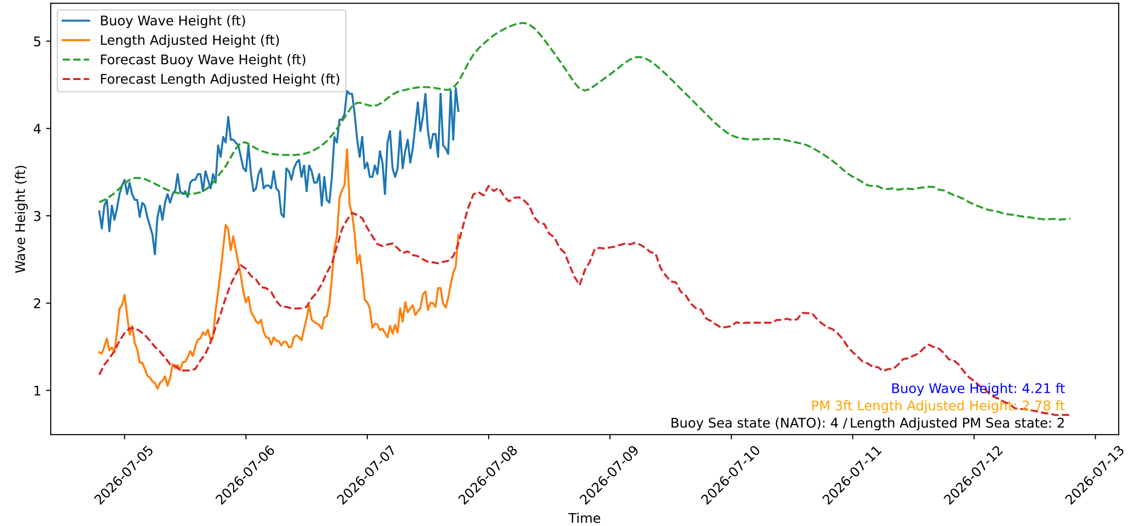
Wave Heights over Time for Green Beach at 2026-07-07 19:01:08
