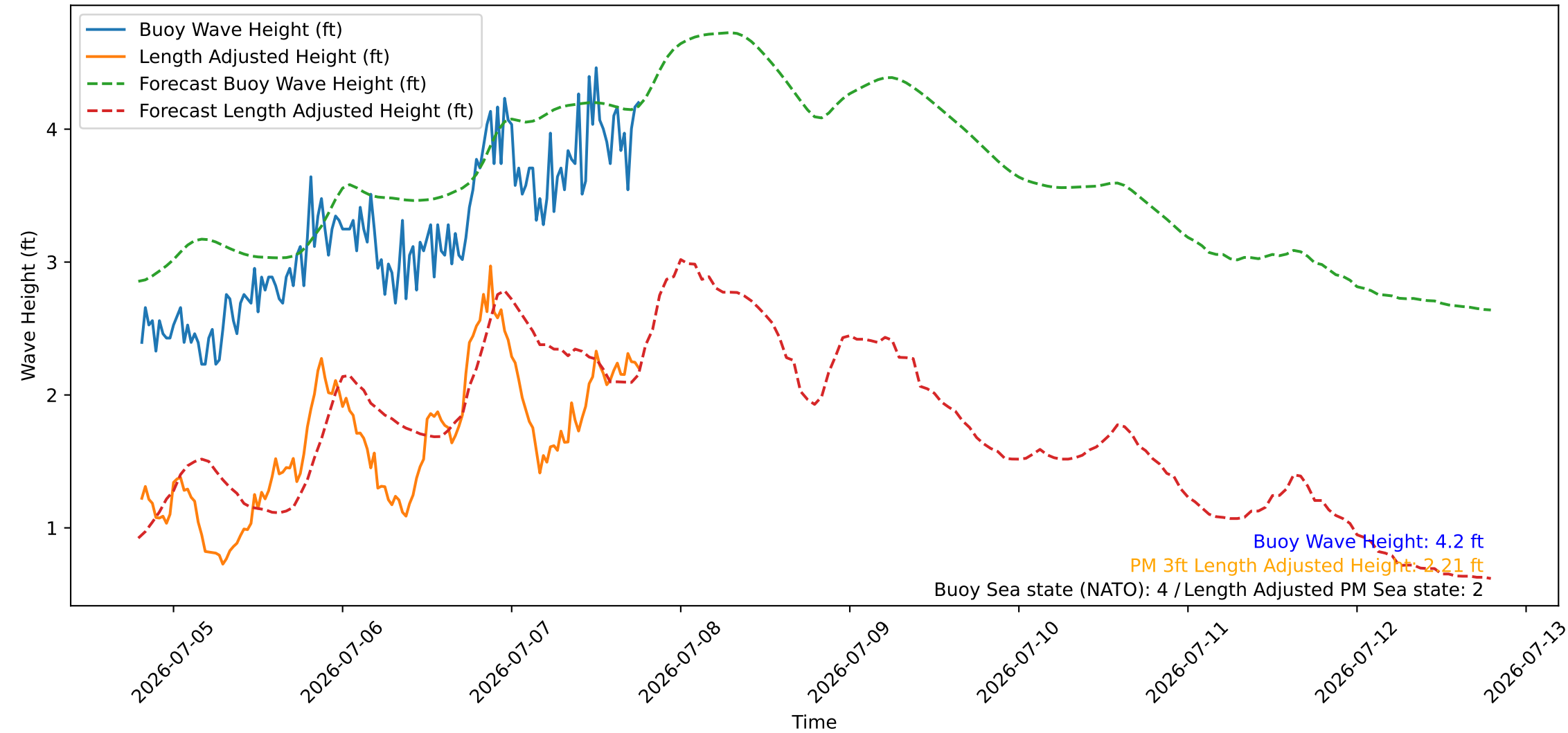
Wave Heights over Time for Red Beach at 2026-07-07 19:00:46
