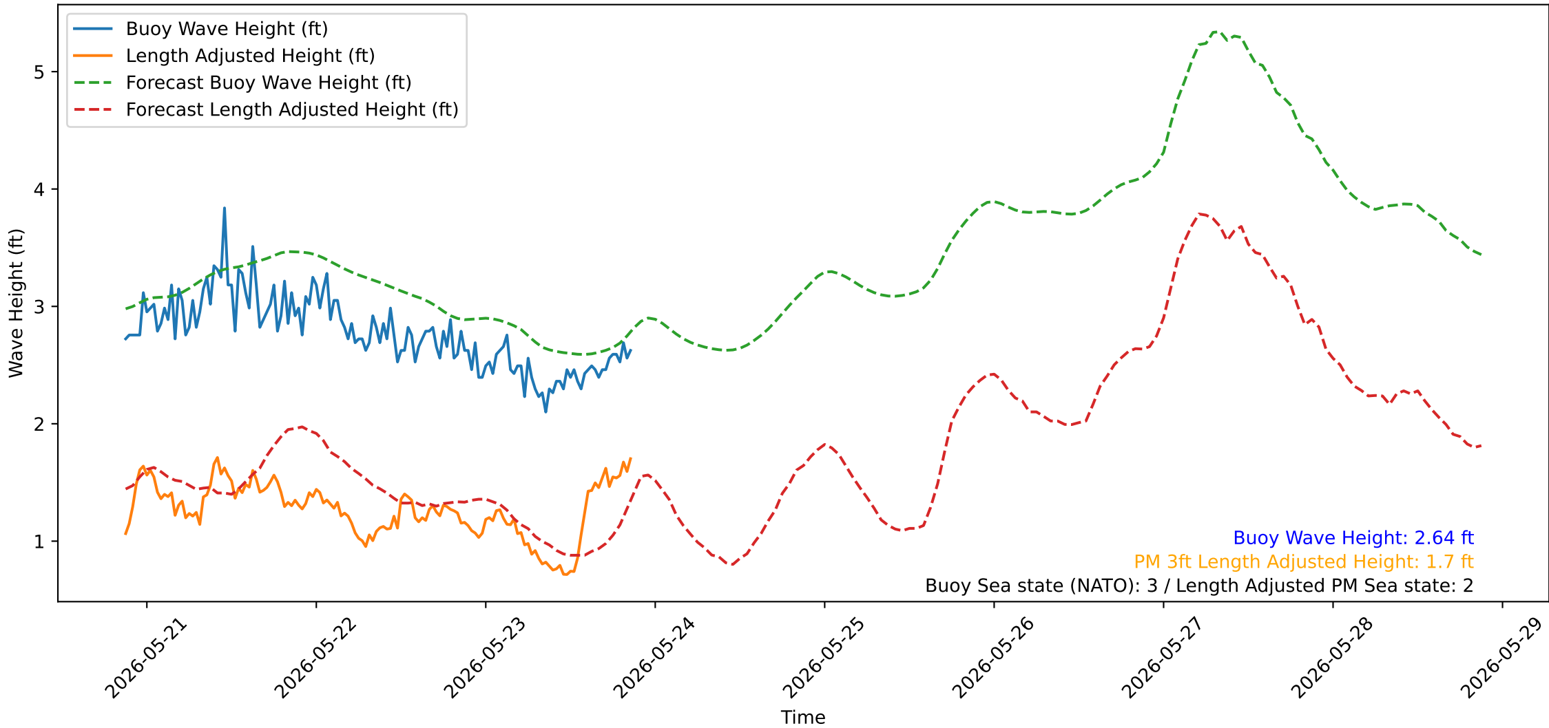
Wave Heights over Time for Oceanside Harbor at 2026-05-23 21:10:32
