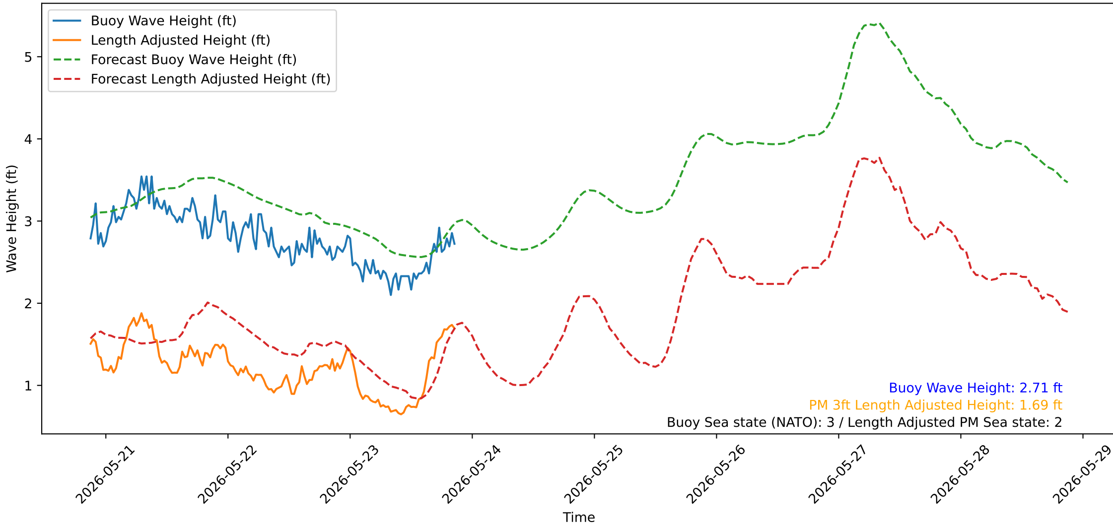
Wave Heights over Time for Green Beach at 2026-05-23 21:11:14
