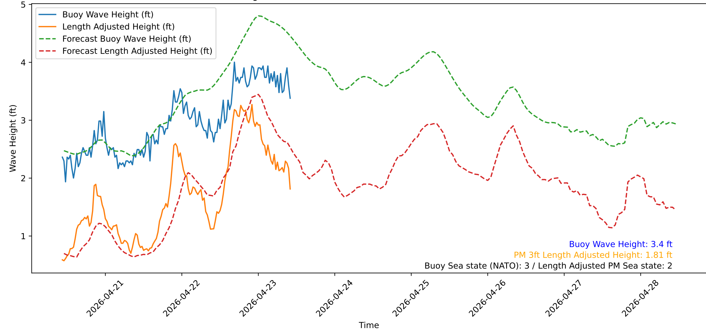
Wave Heights over Time for Green Beach at 2026-04-23 10:41:13
