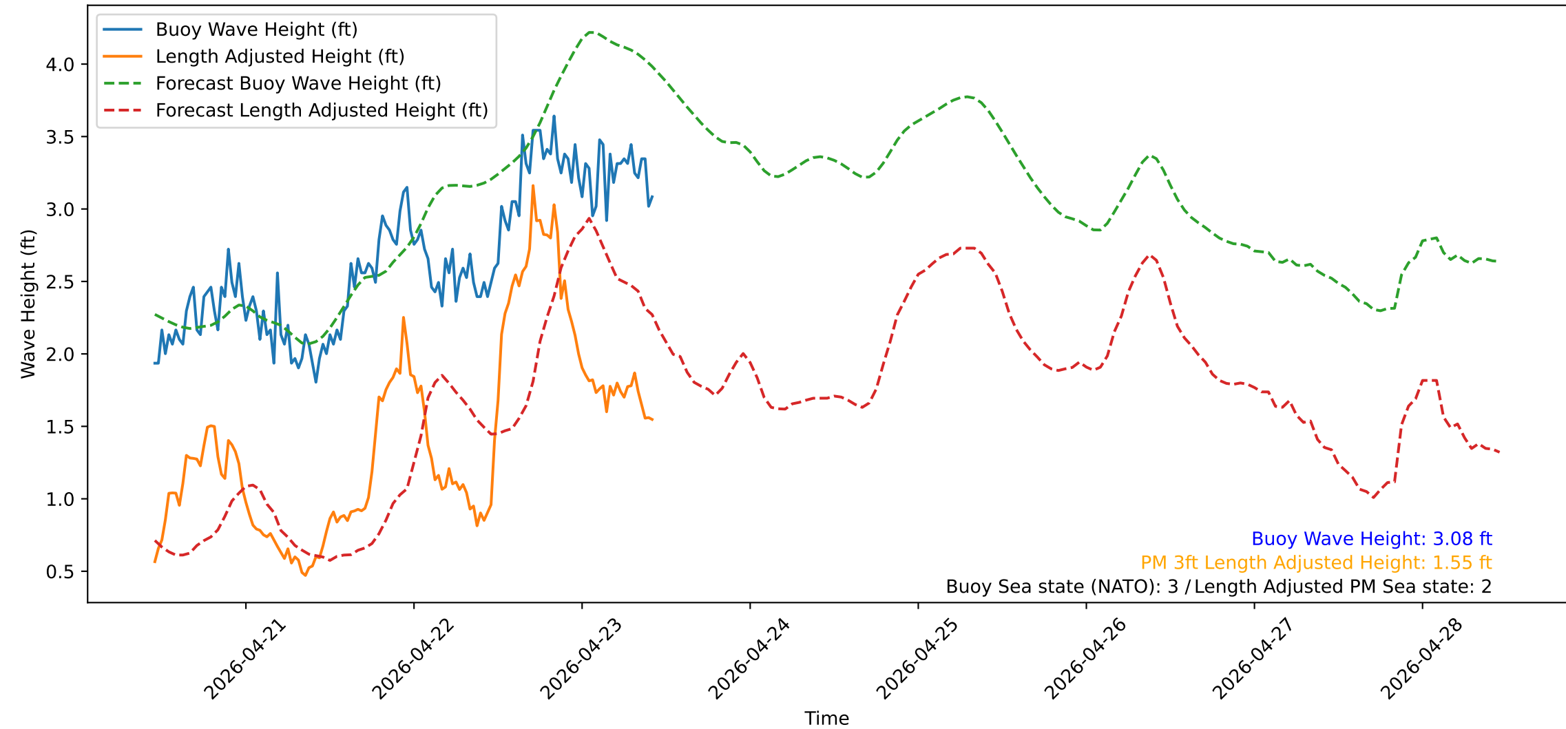
Wave Heights over Time for Red Beach at 2026-04-23 10:40:50
