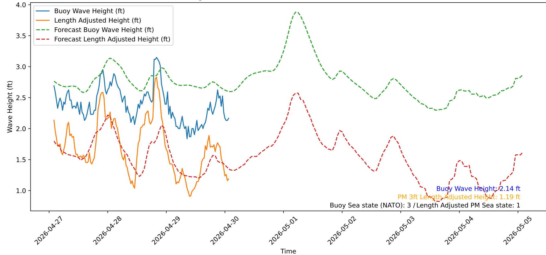
Wave Heights over Time for Green Beach at 2026-04-30 02:11:13
