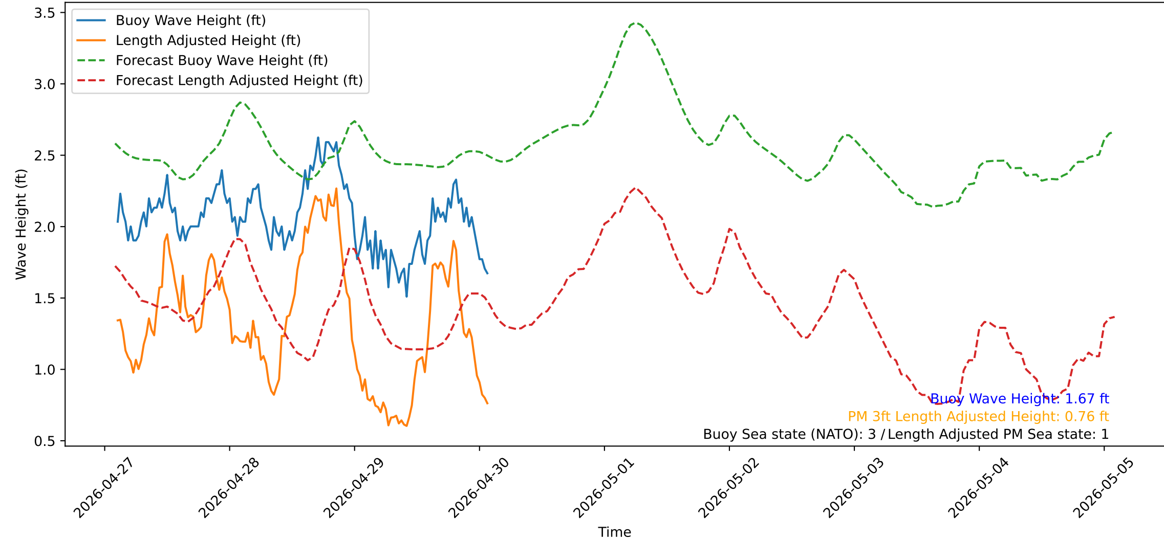
Wave Heights over Time for Red Beach at 2026-04-30 02:10:50
