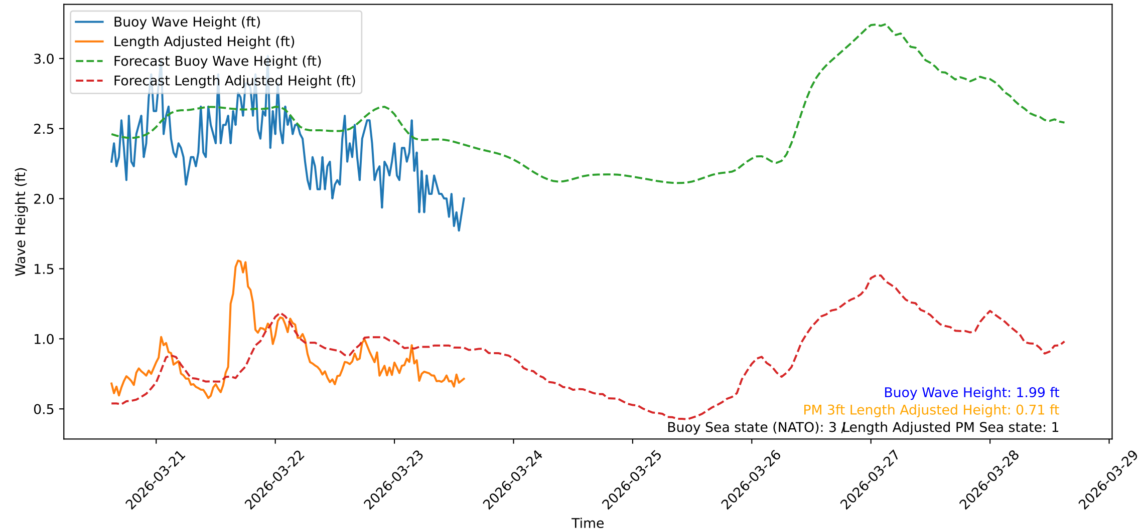
Wave Heights over Time for Oceanside Harbor at 2026-03-23 14:50:30
