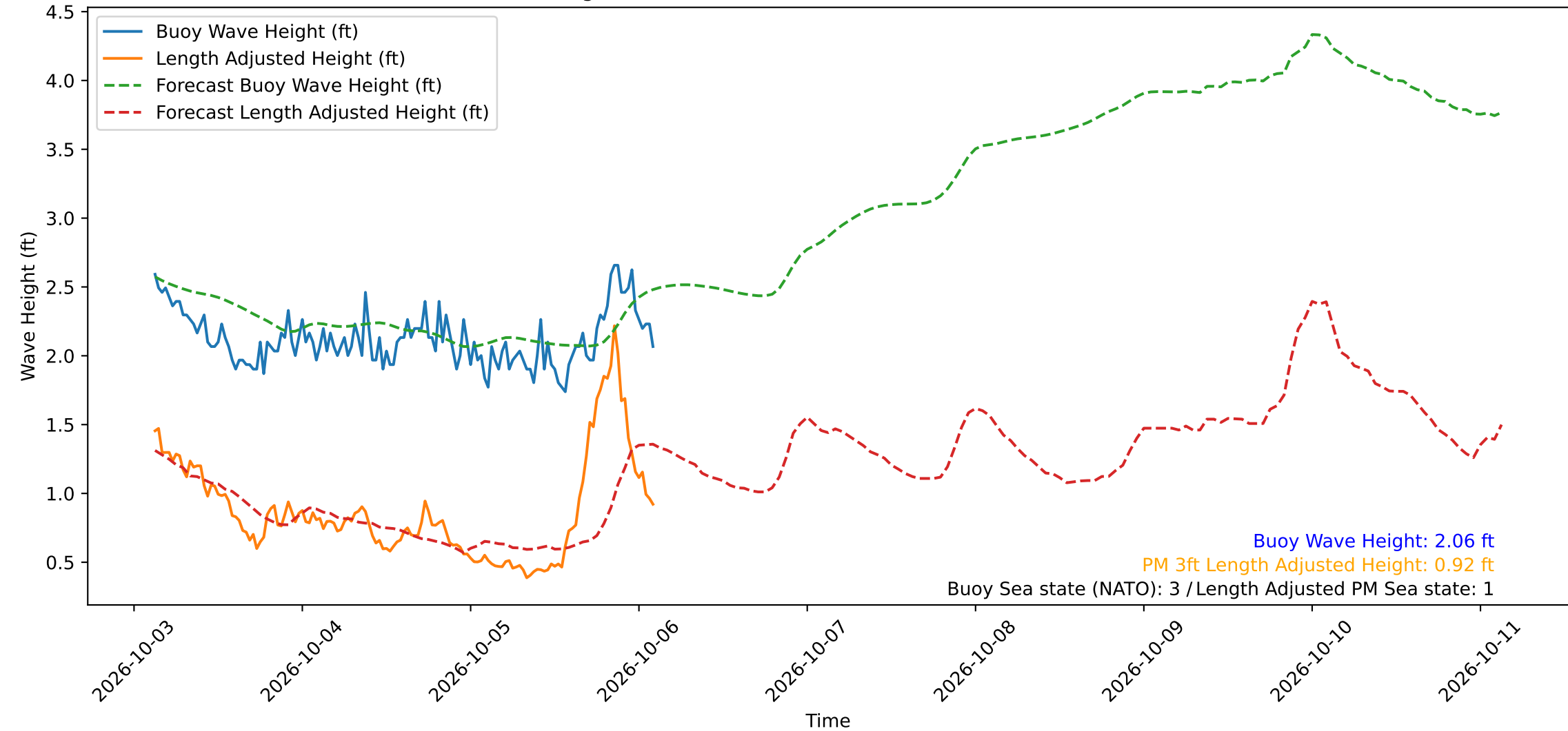
Wave Heights over Time for Red Beach at 2026-10-06 02:40:49
