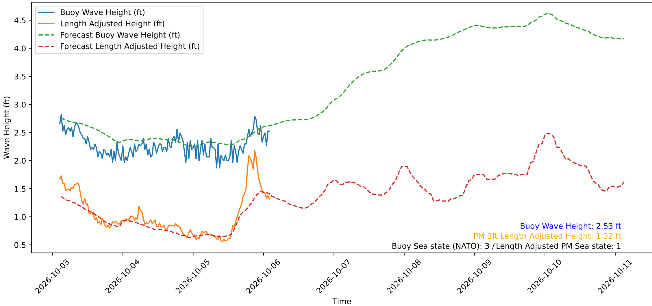
Wave Heights over Time for Oceanside Harbor at 2026-10-06 02:40:29
