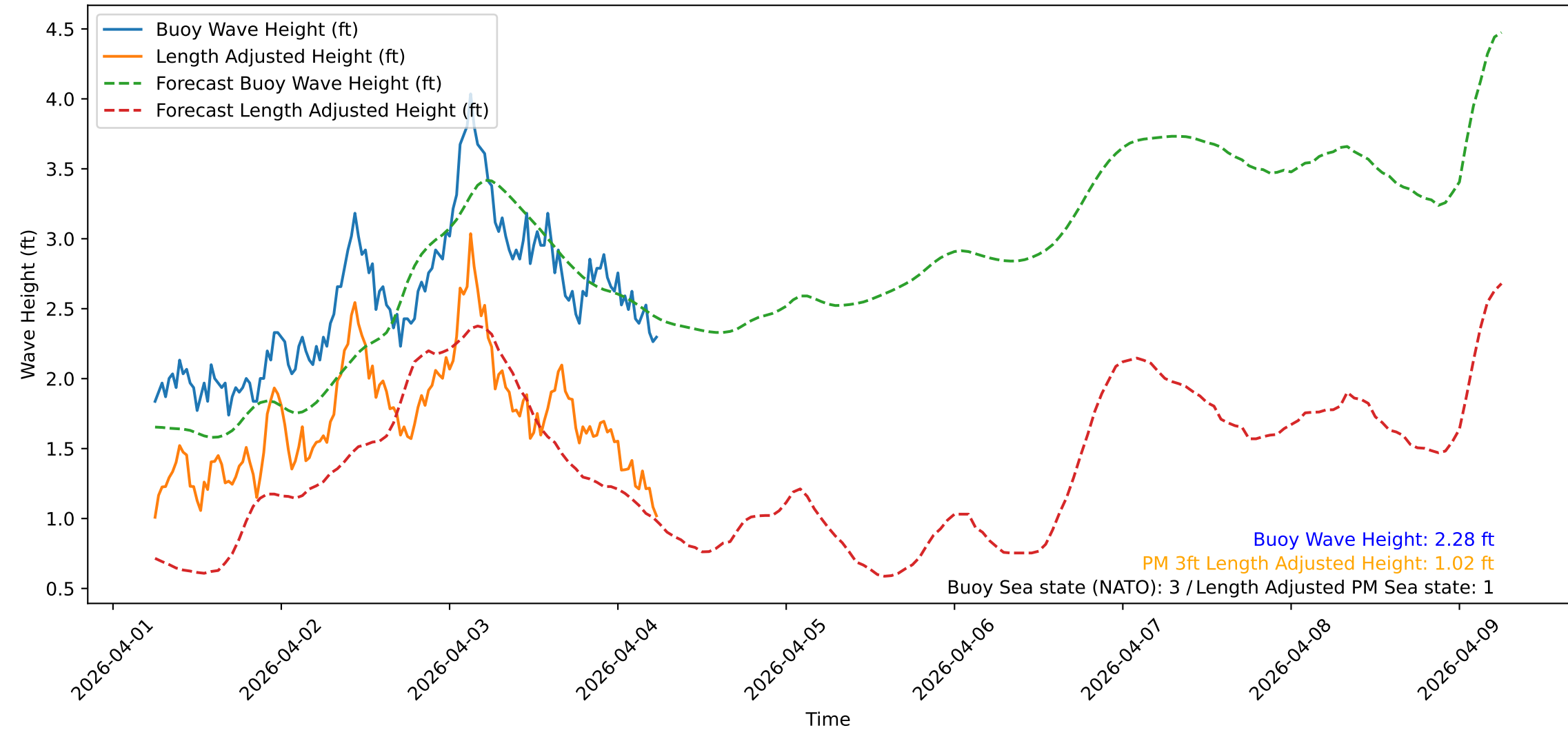
Wave Heights over Time for Oceanside Harbor at 2026-04-04 06:10:31
