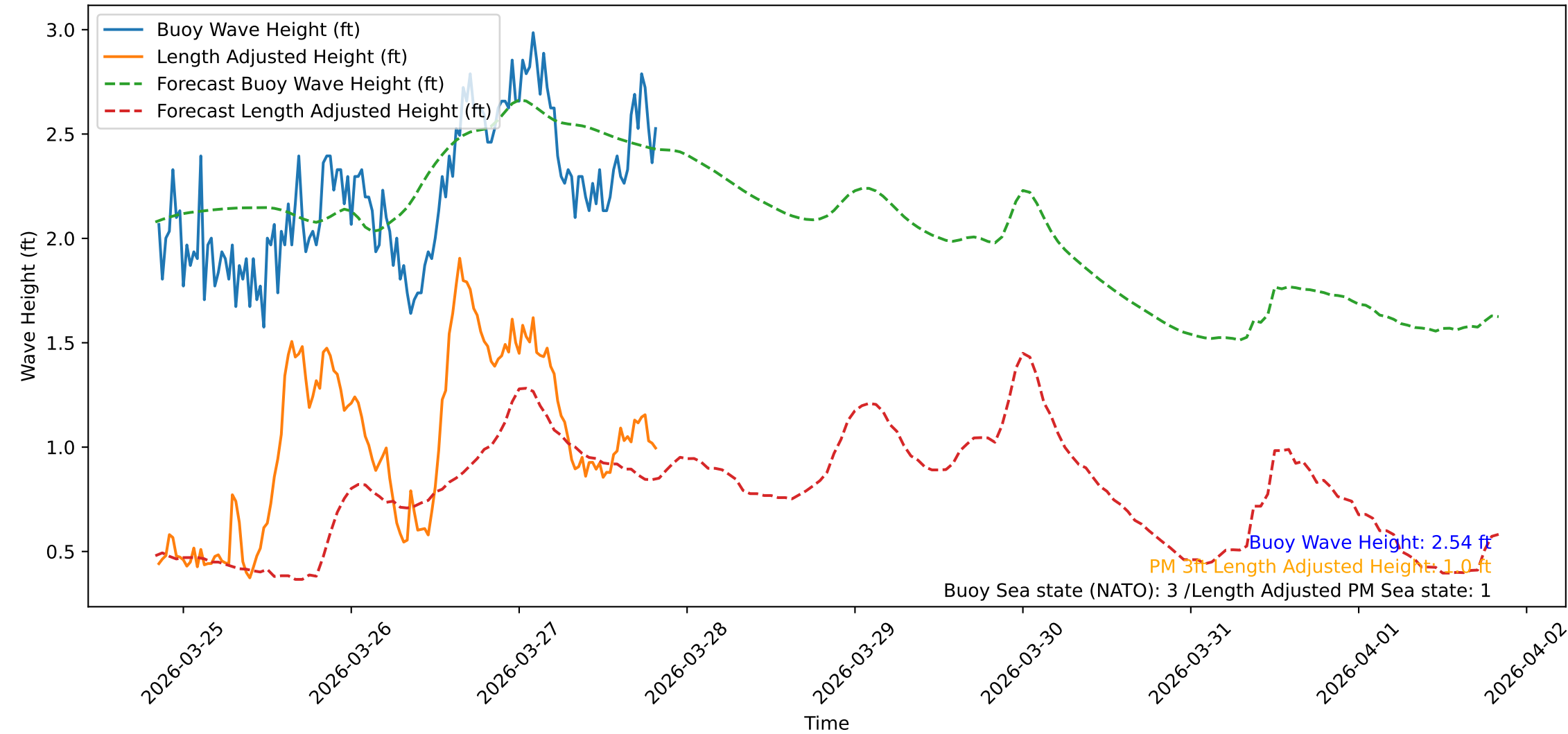
Wave Heights over Time for Red Beach at 2026-03-27 20:10:47
