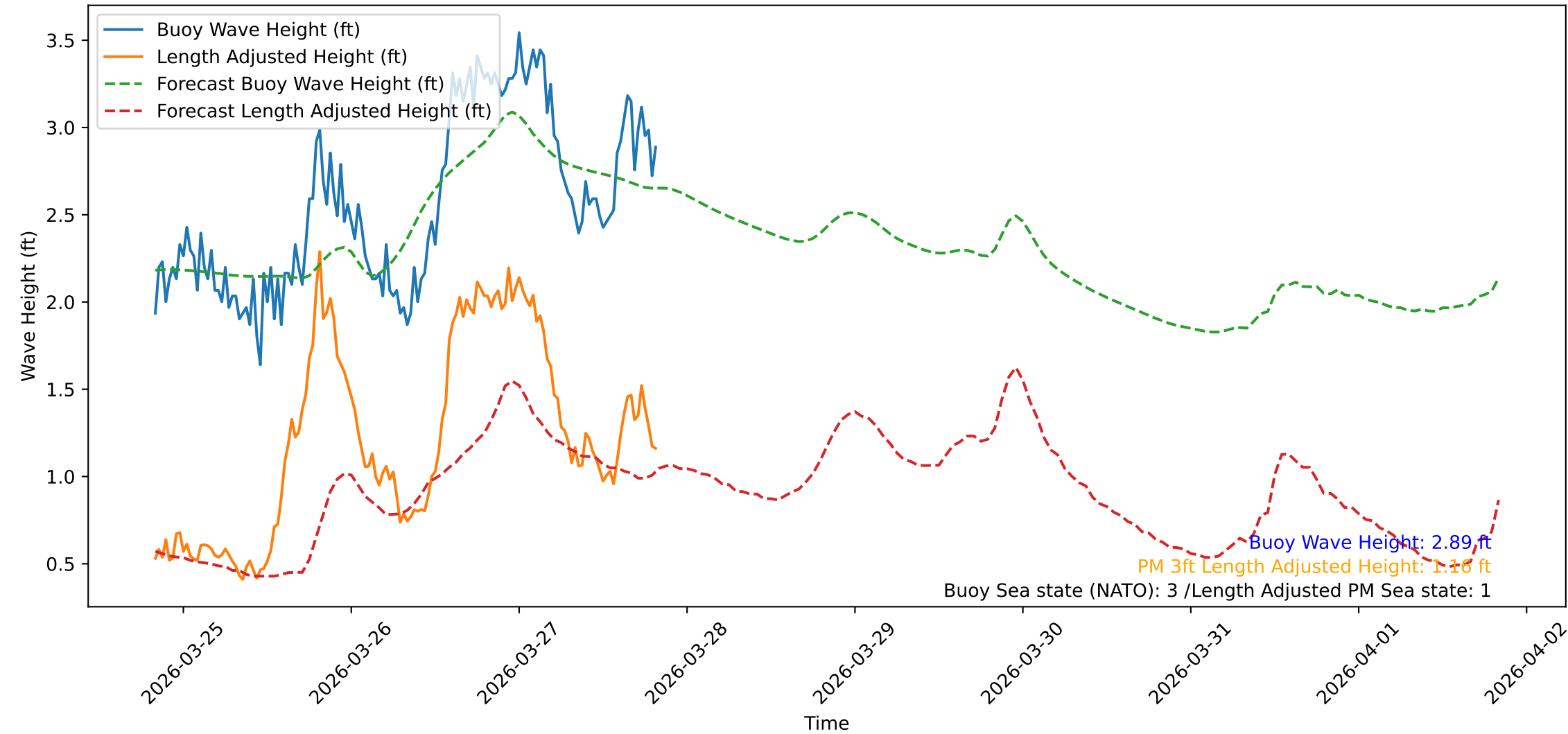
Wave Heights over Time for Green Beach at 2026-03-27 20:11:09
