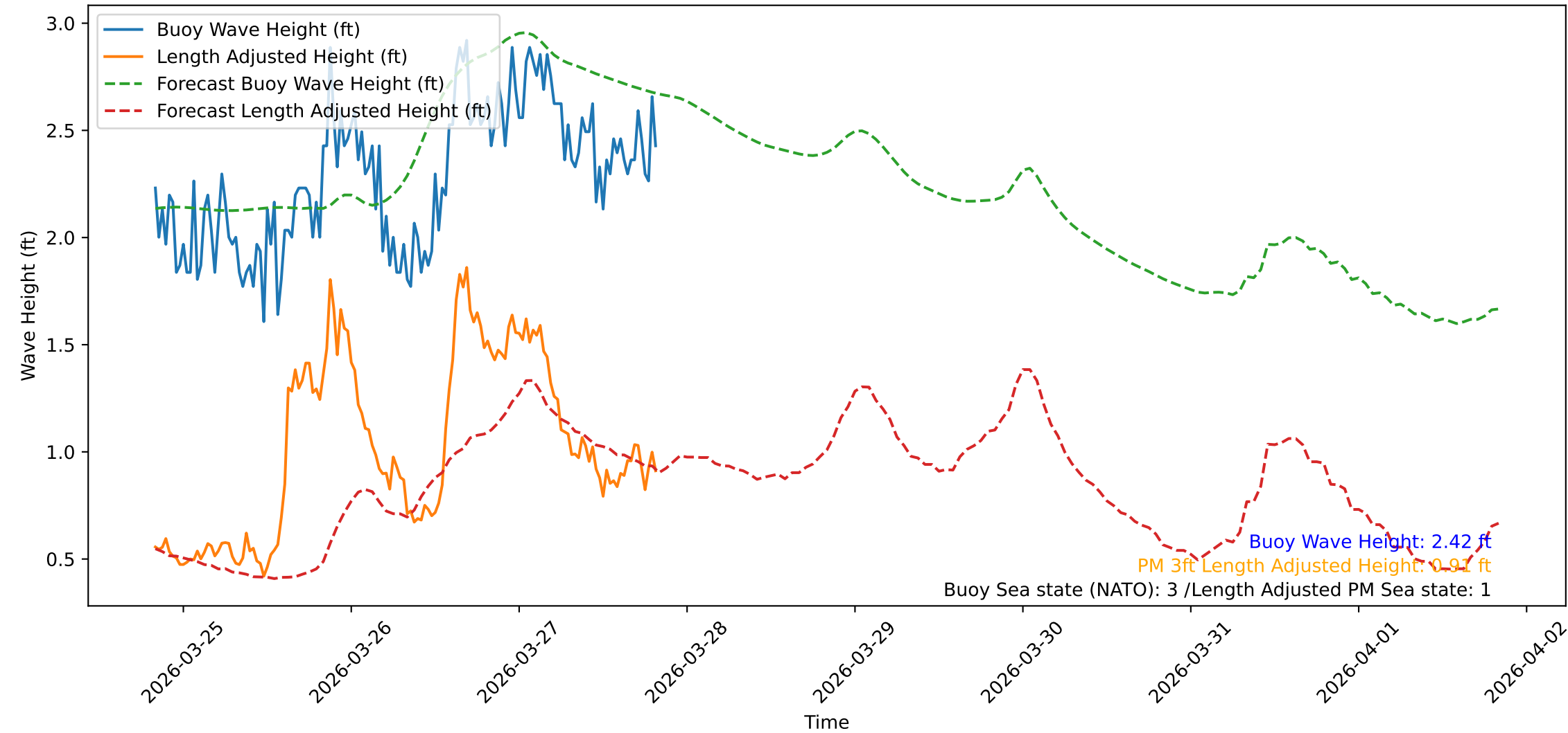
Wave Heights over Time for Oceanside Harbor at 2026-03-27 20:10:31
