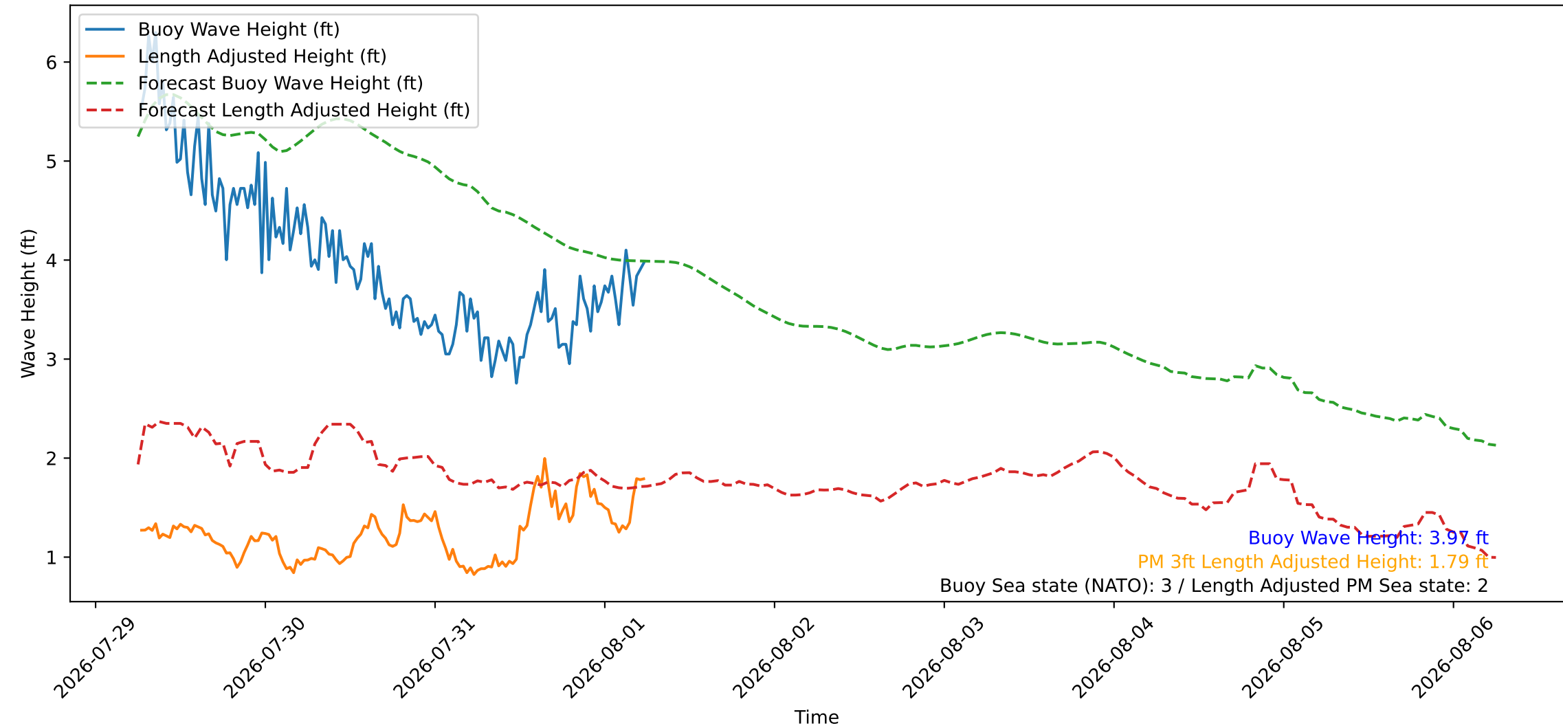
Wave Heights over Time for Green Beach at 2026-08-01 06:21:10
