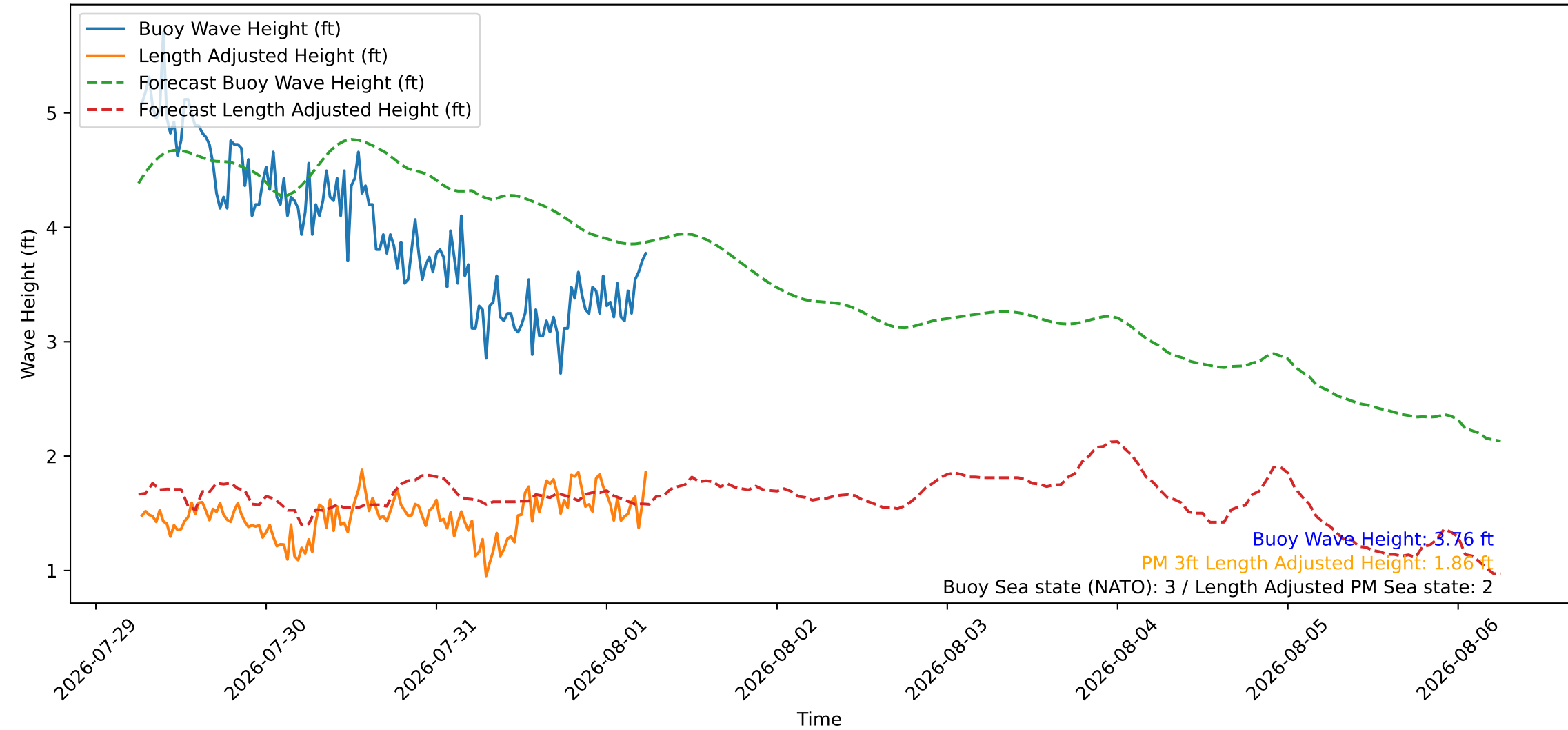
Wave Heights over Time for Oceanside Harbor at 2026-08-01 06:20:27
