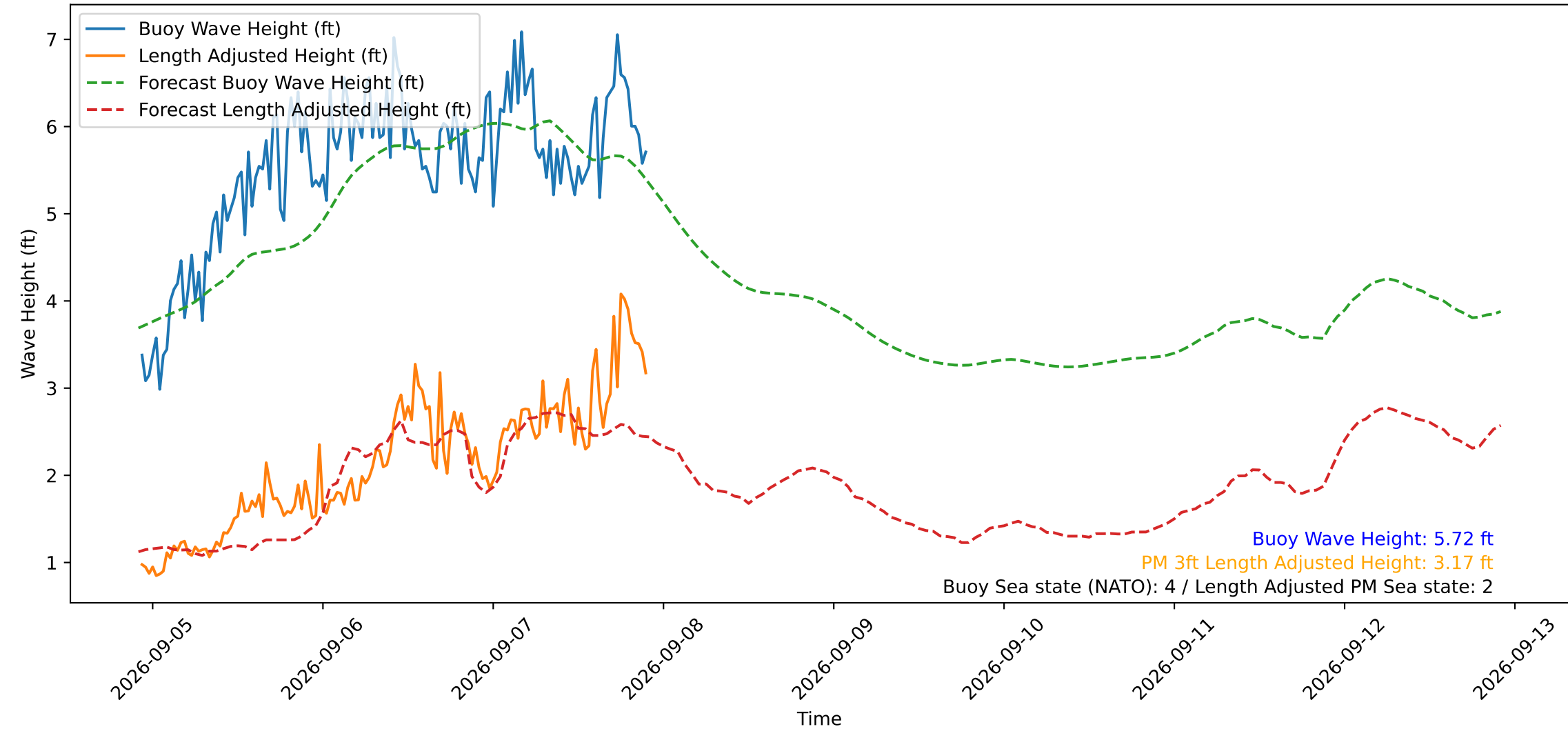
Wave Heights over Time for Oceanside Harbor at 2026-09-07 22:20:29
