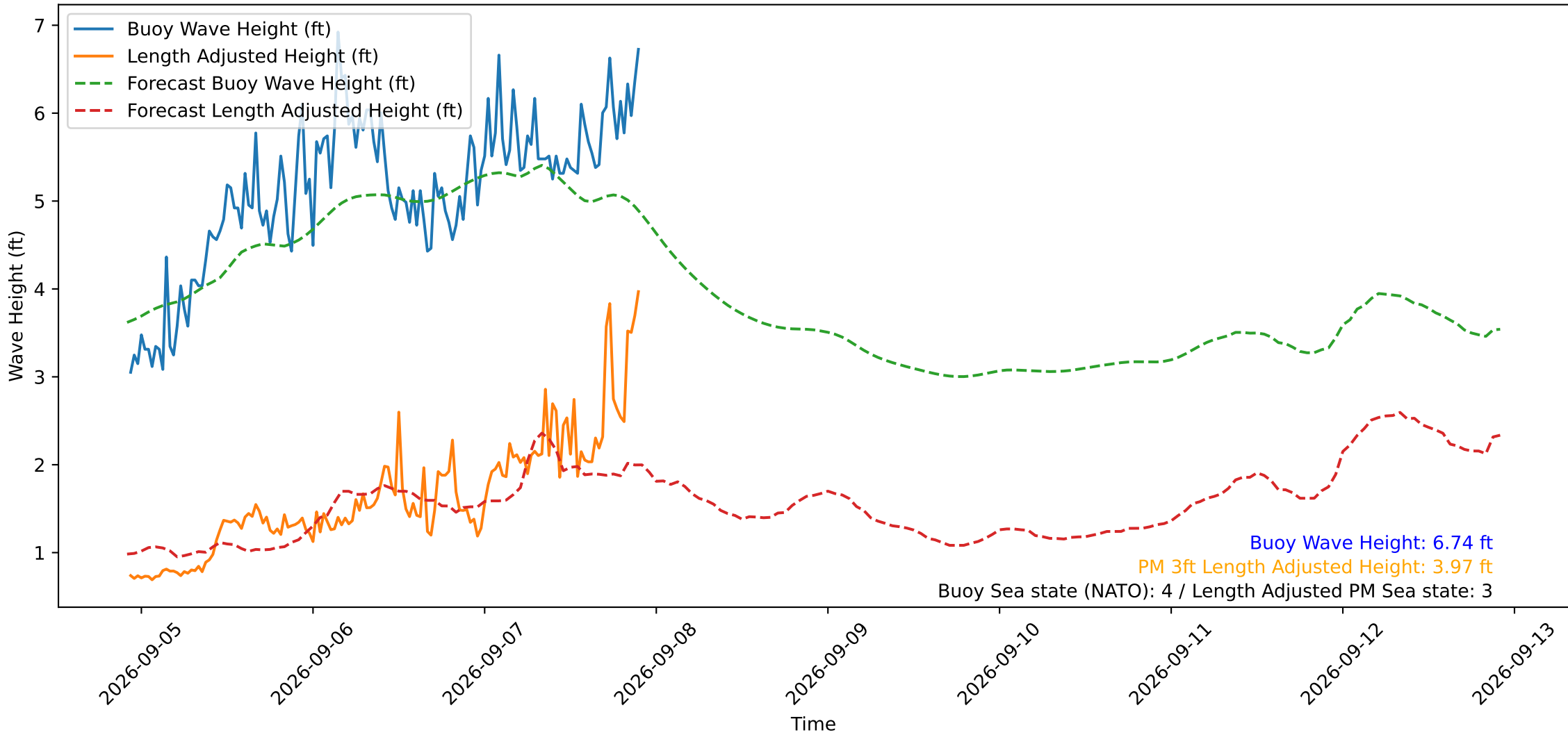
Wave Heights over Time for Red Beach at 2026-09-07 22:20:51
