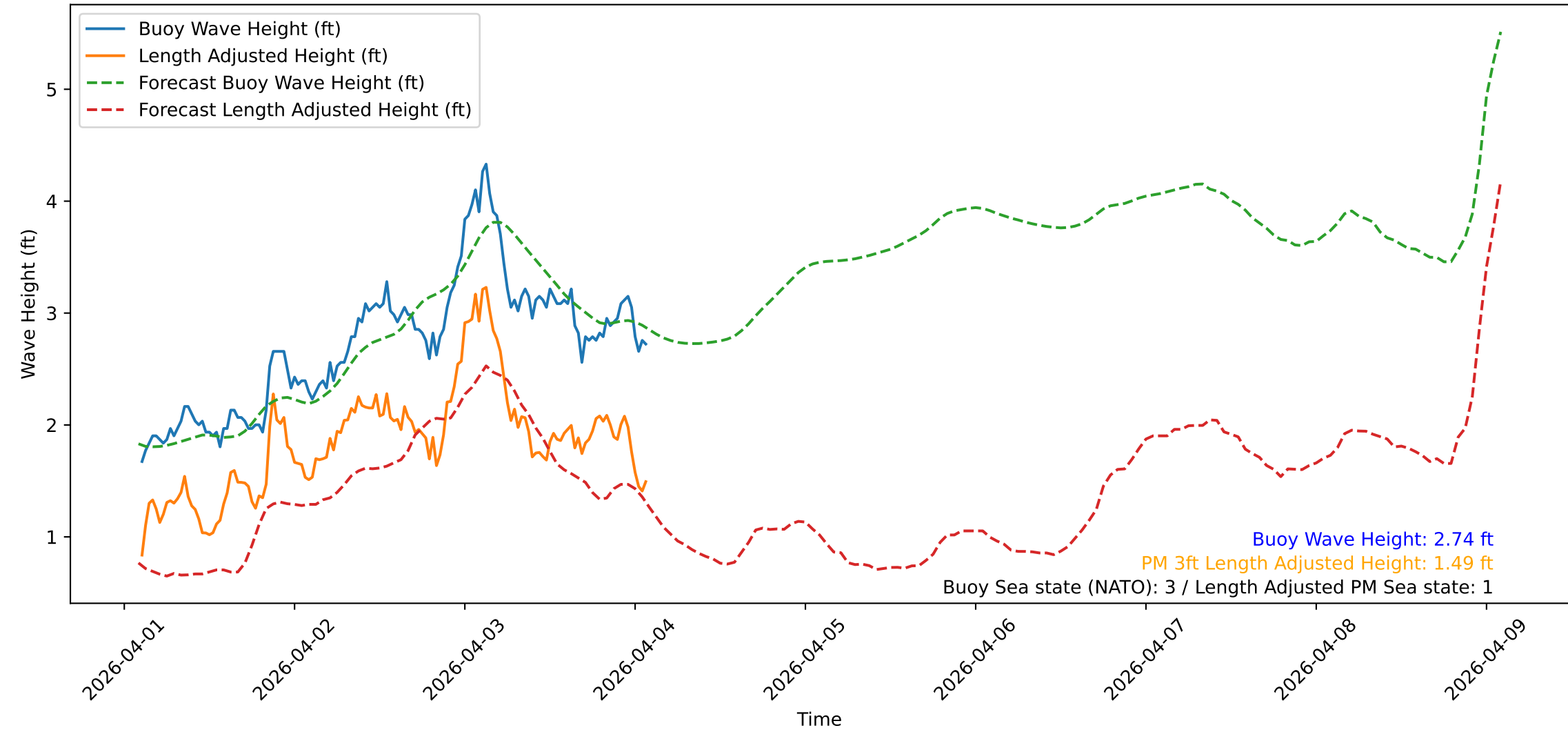
Wave Heights over Time for Green Beach at 2026-04-04 02:21:10
