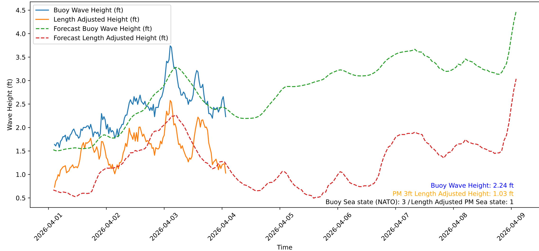
Wave Heights over Time for Red Beach at 2026-04-04 02:20:48
