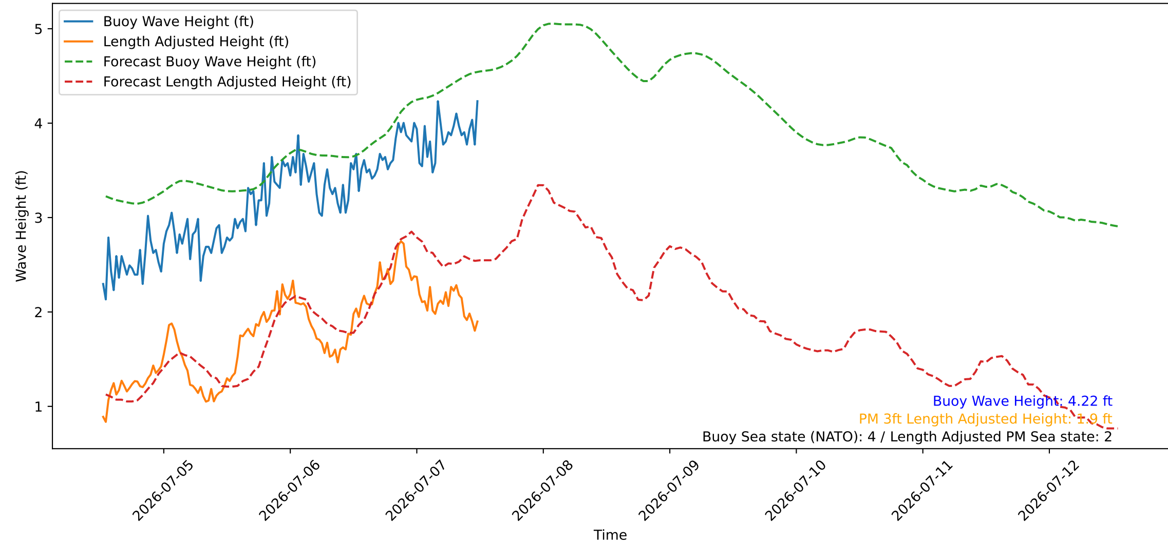
Wave Heights over Time for Oceanside Harbor at 2026-07-07 12:30:27
