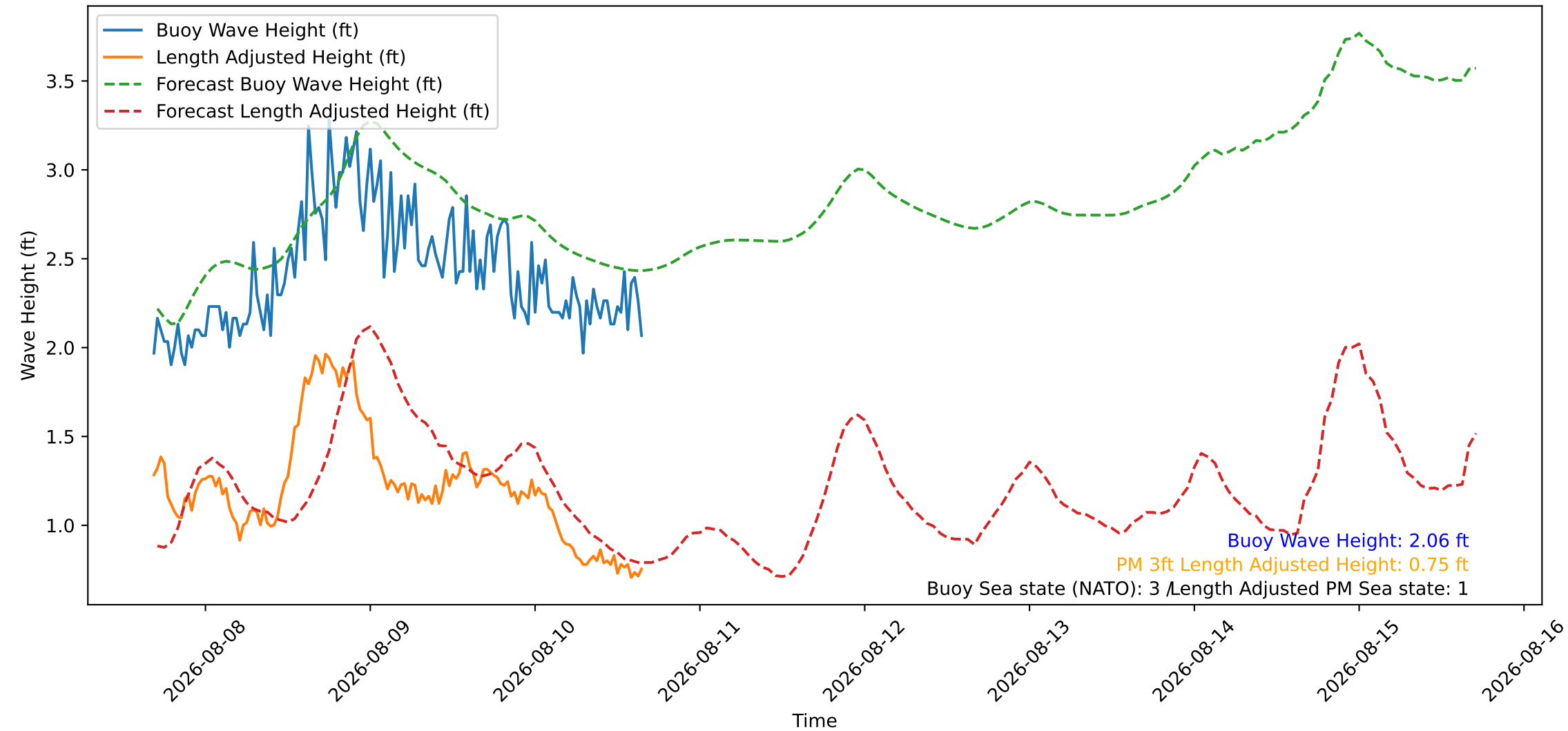
Wave Heights over Time for Oceanside Harbor at 2026-08-10 16:30:27
