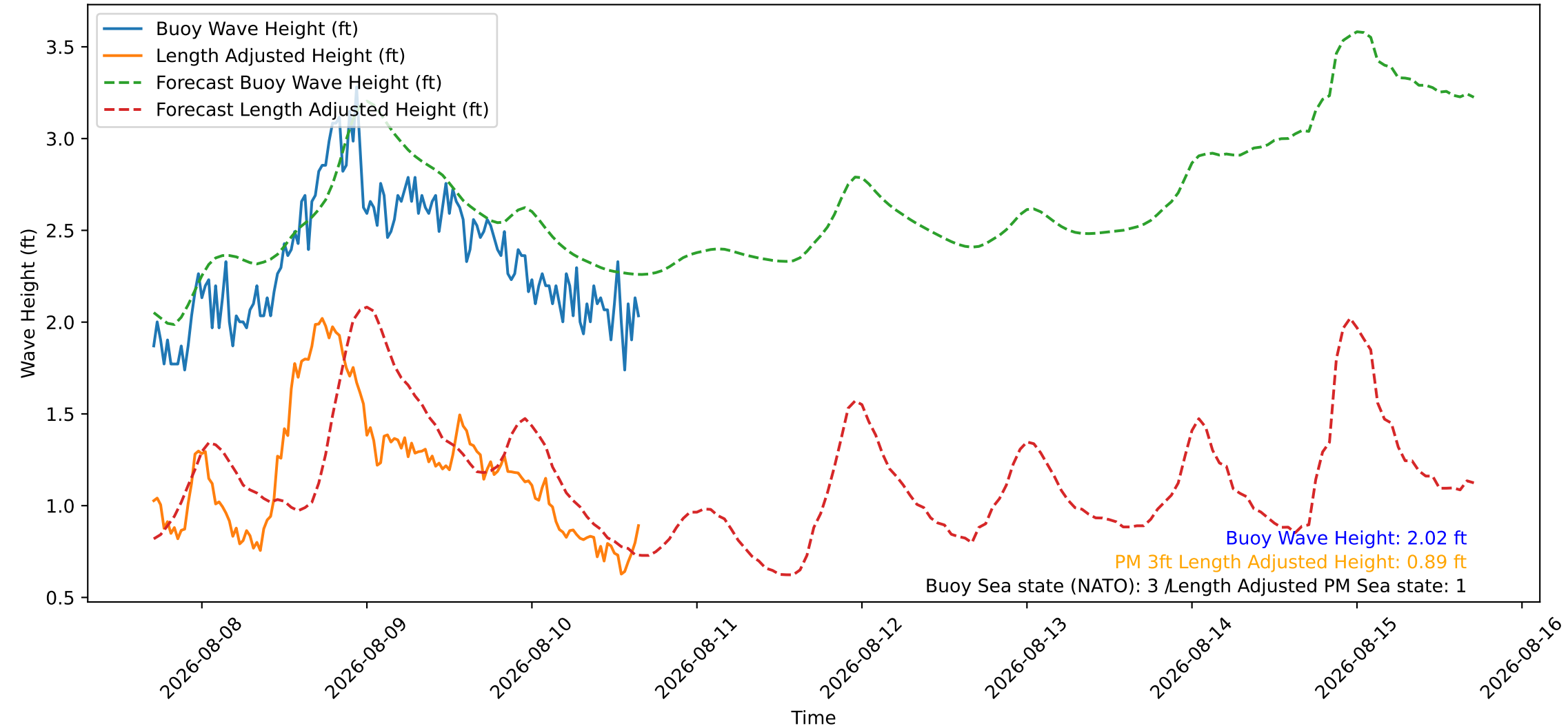
Wave Heights over Time for Red Beach at 2026-08-10 16:30:47
