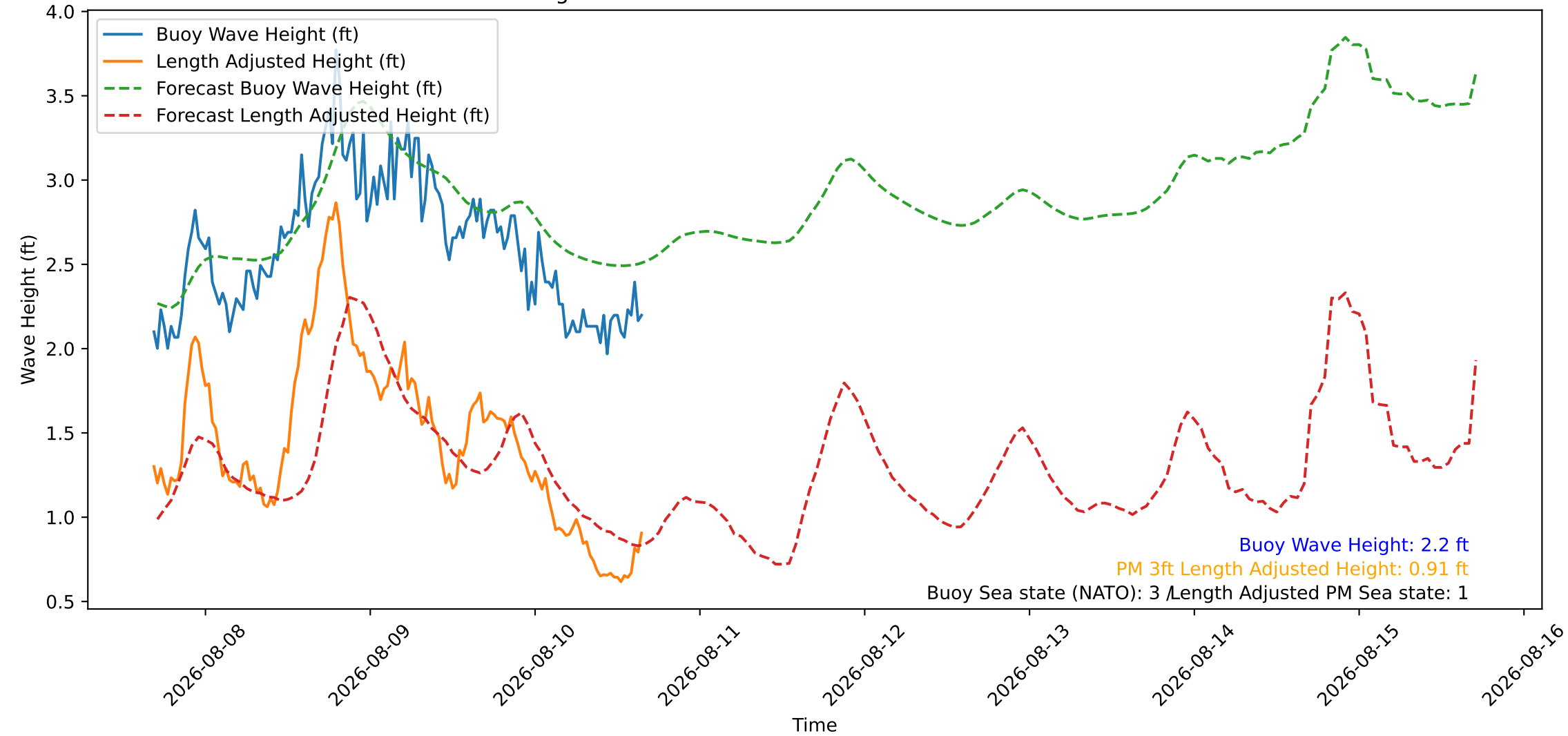
Wave Heights over Time for Green Beach at 2026-08-10 16:31:10
