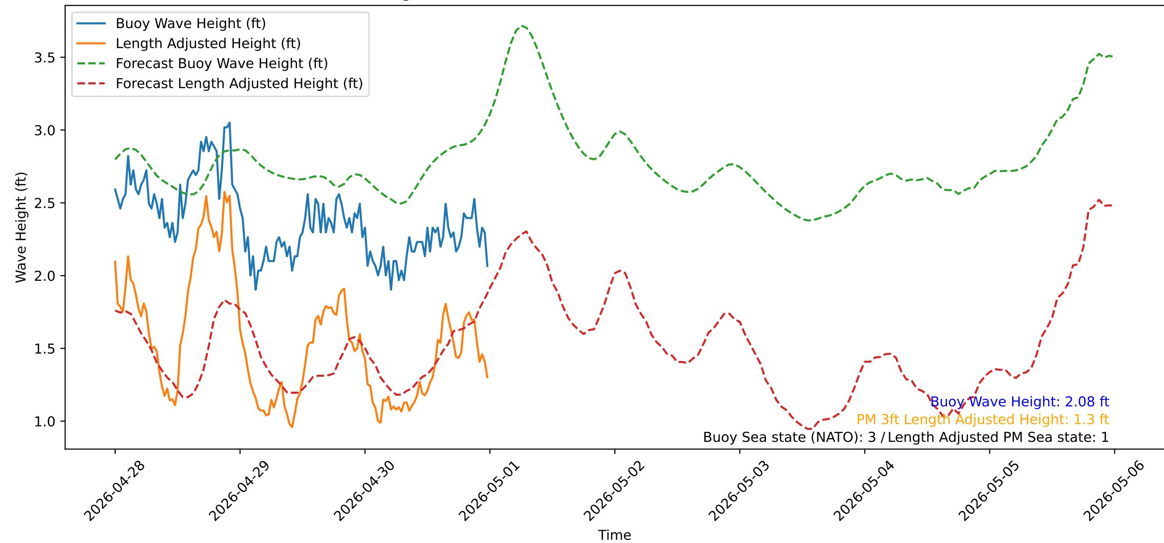
Wave Heights over Time for Oceanside Harbor at 2026-05-01 00:10:32
