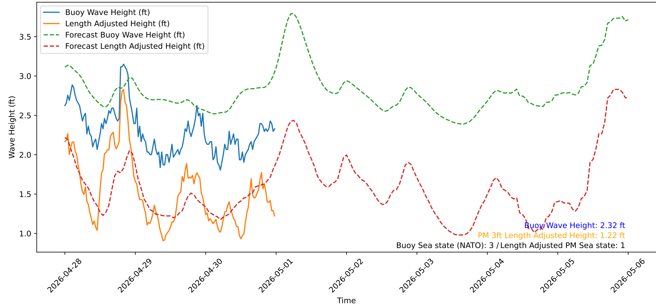
Wave Heights over Time for Green Beach at 2026-05-01 00:11:13
