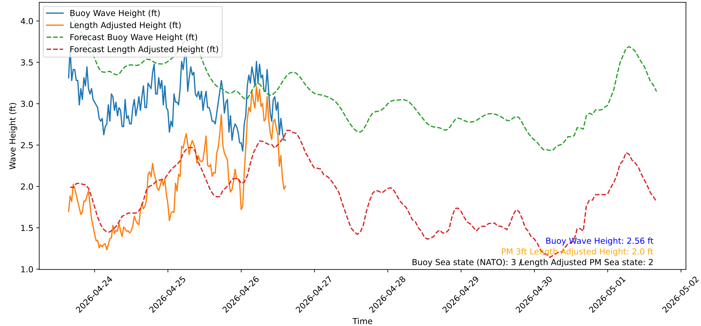
Wave Heights over Time for Green Beach at 2026-04-26 15:31:13
