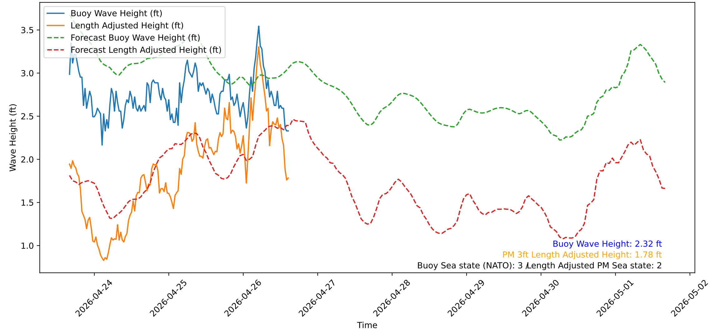
Wave Heights over Time for Red Beach at 2026-04-26 15:30:50
