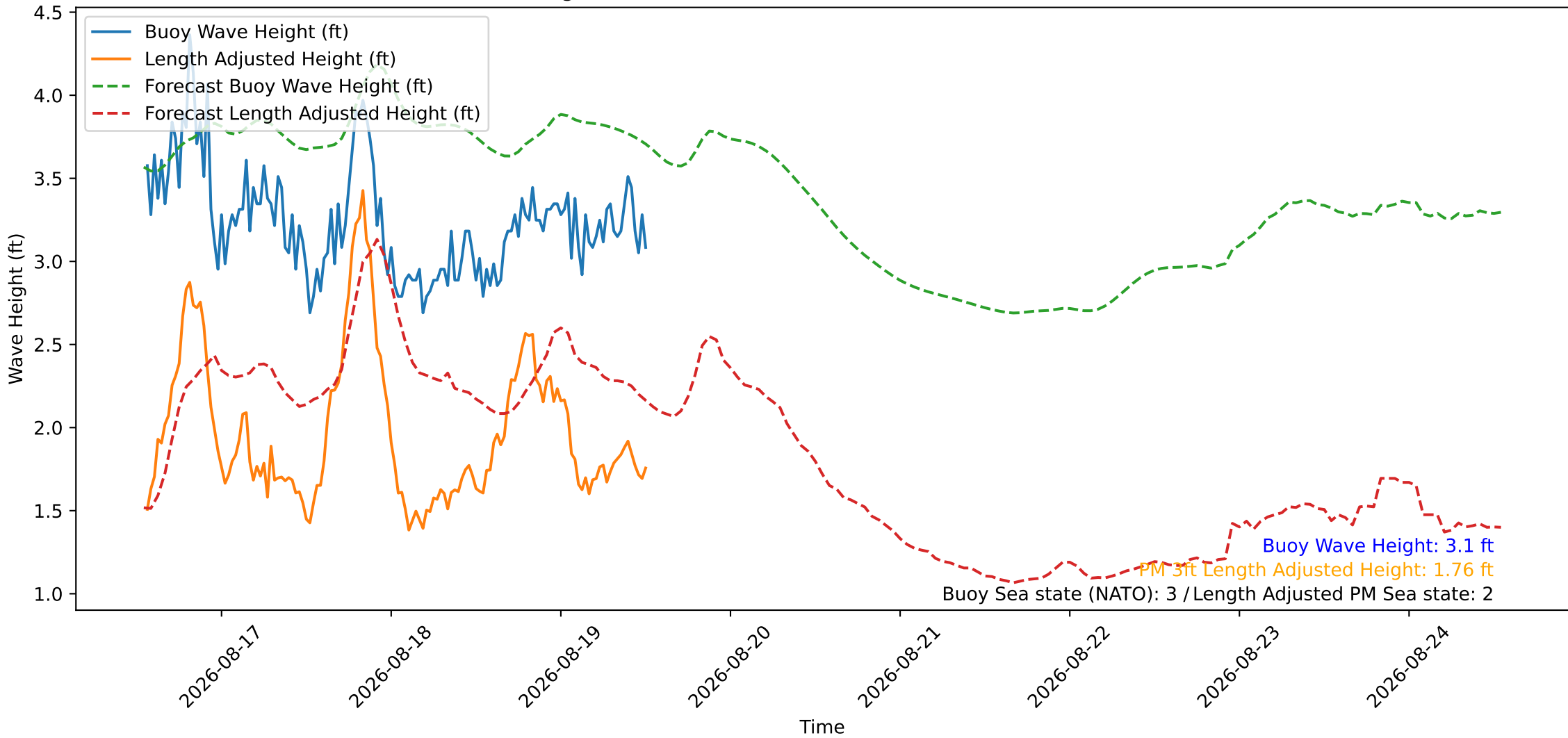
Wave Heights over Time for Green Beach at 2026-08-19 13:01:09
