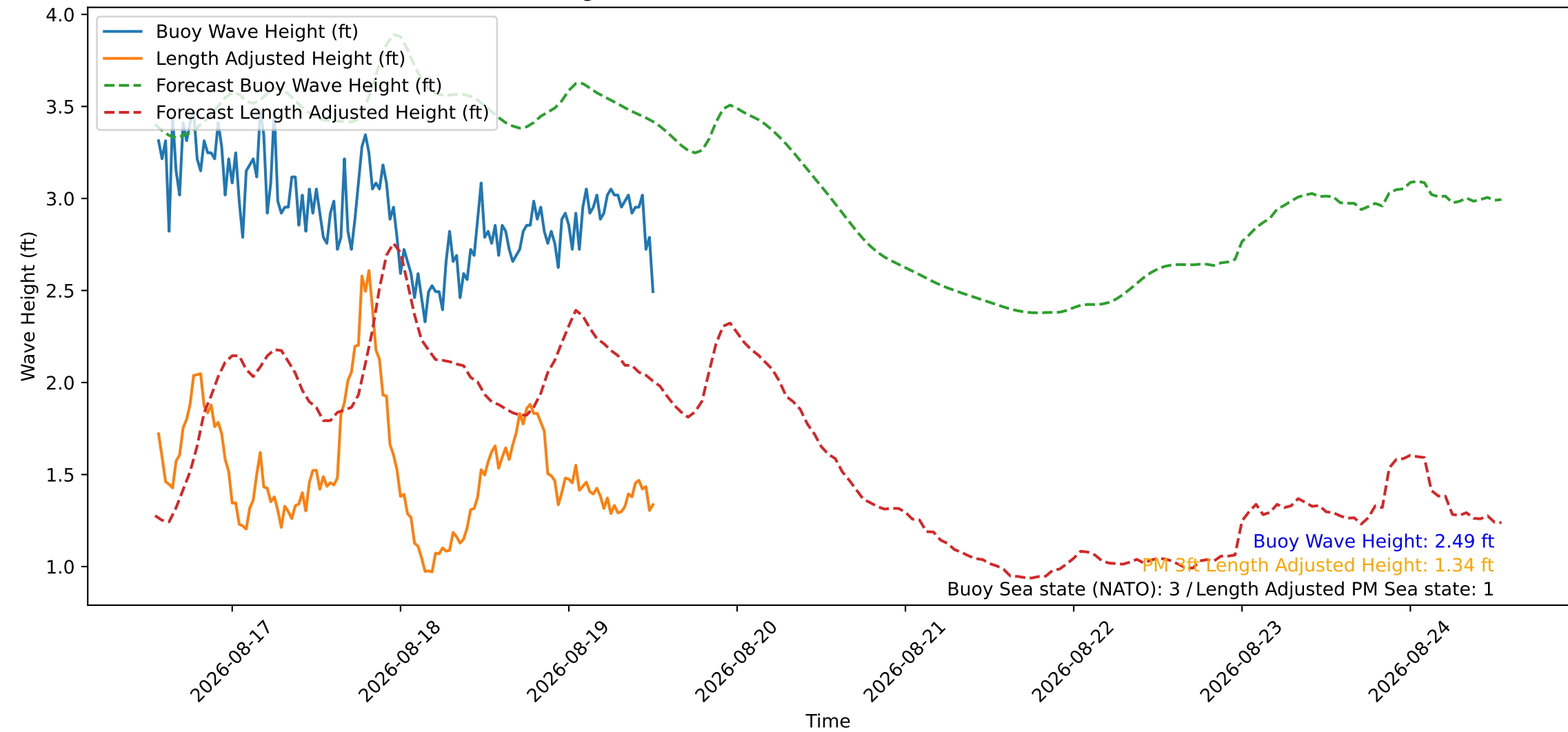
Wave Heights over Time for Red Beach at 2026-08-19 13:00:46
