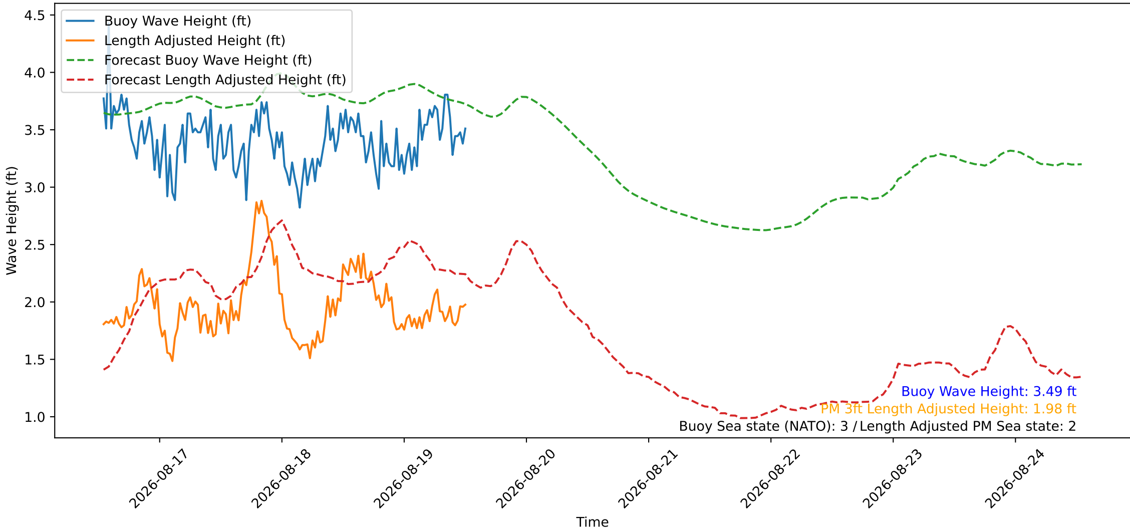
Wave Heights over Time for Oceanside Harbor at 2026-08-19 13:00:26
