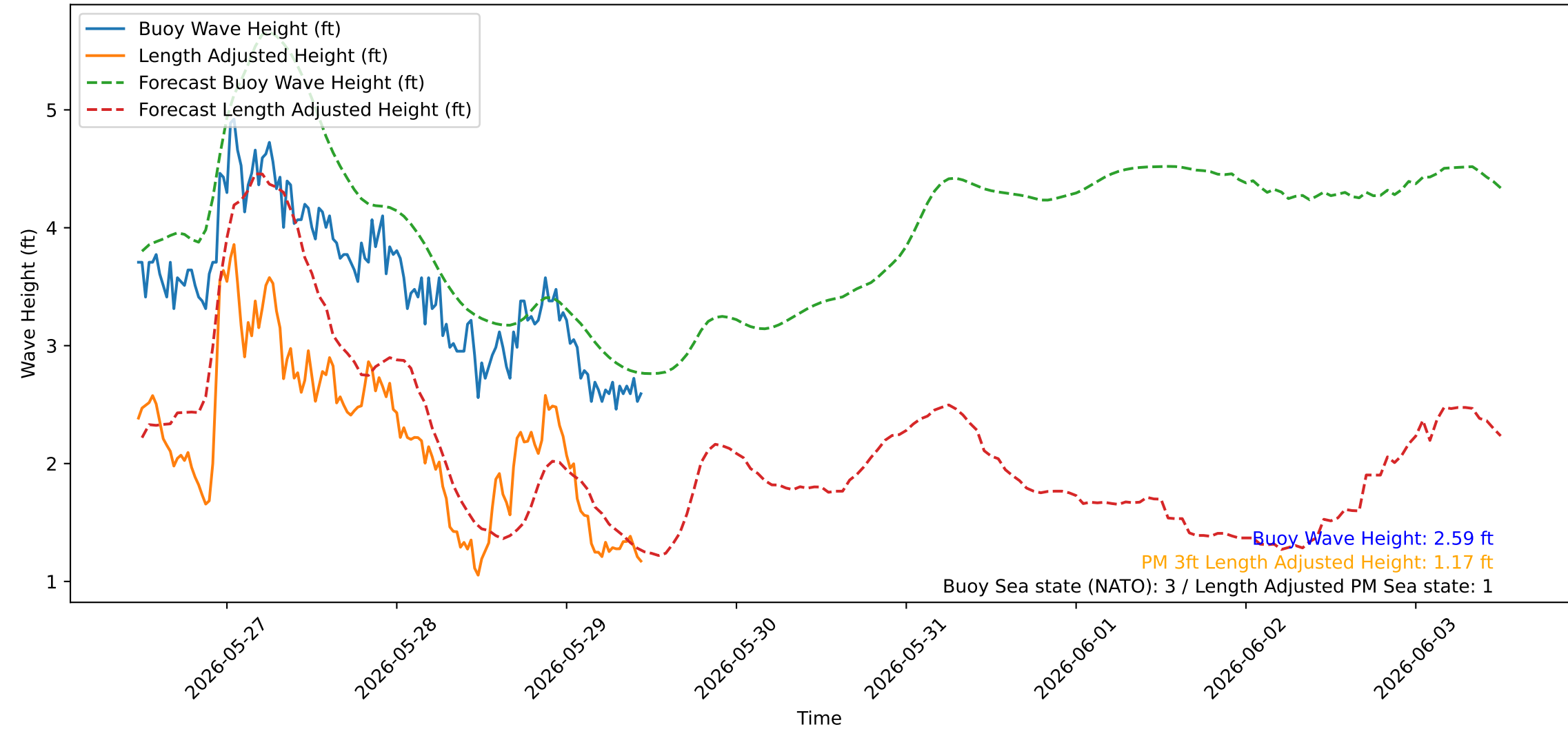
Wave Heights over Time for Green Beach at 2026-05-29 11:31:04
