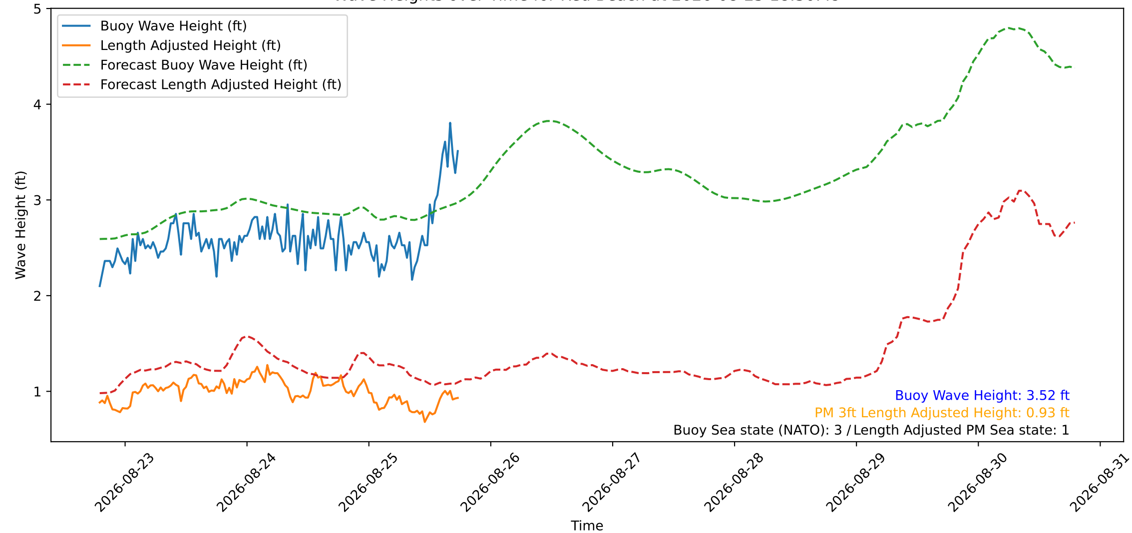
Wave Heights over Time for Red Beach at 2026-08-25 18:30:49
