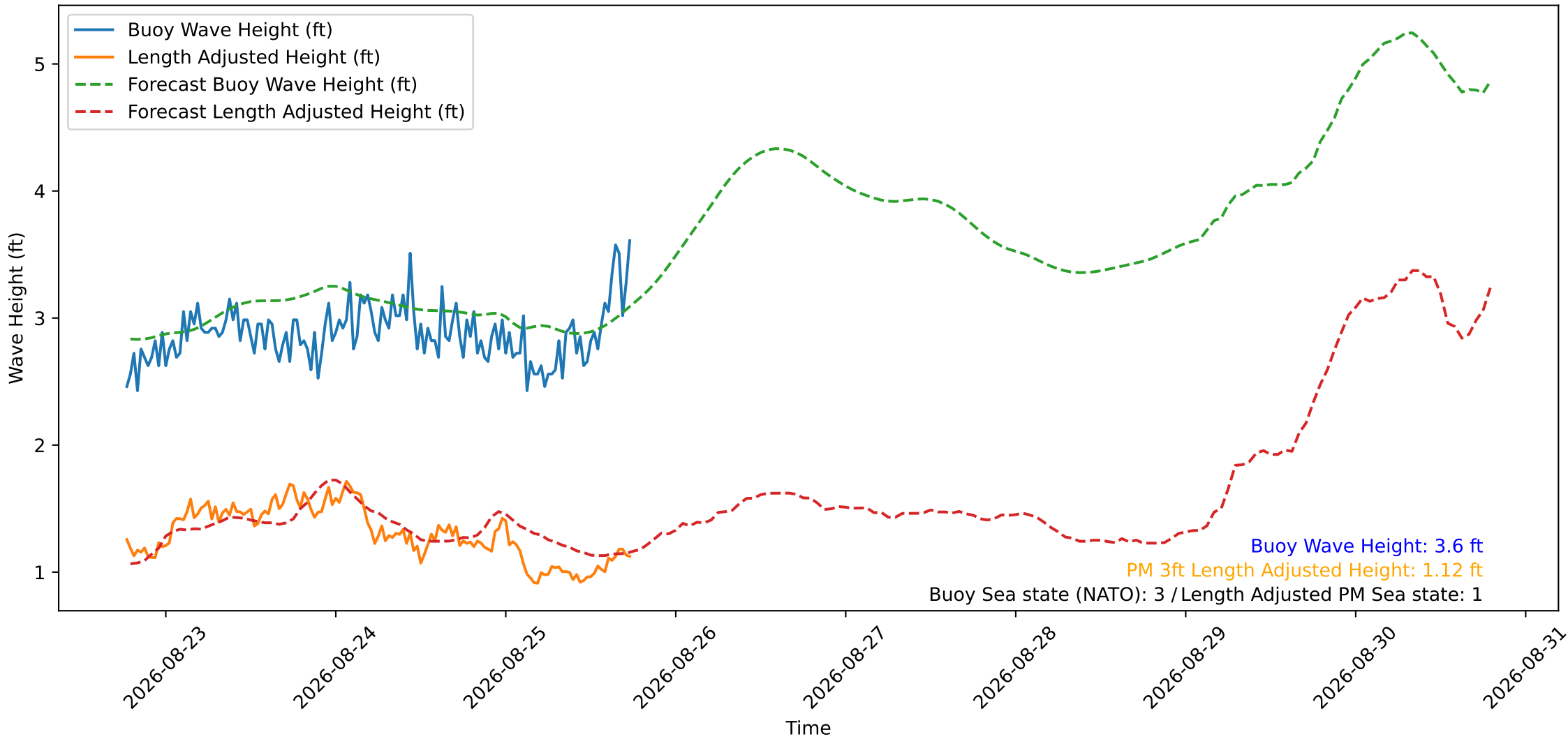
Wave Heights over Time for Oceanside Harbor at 2026-08-25 18:30:30
