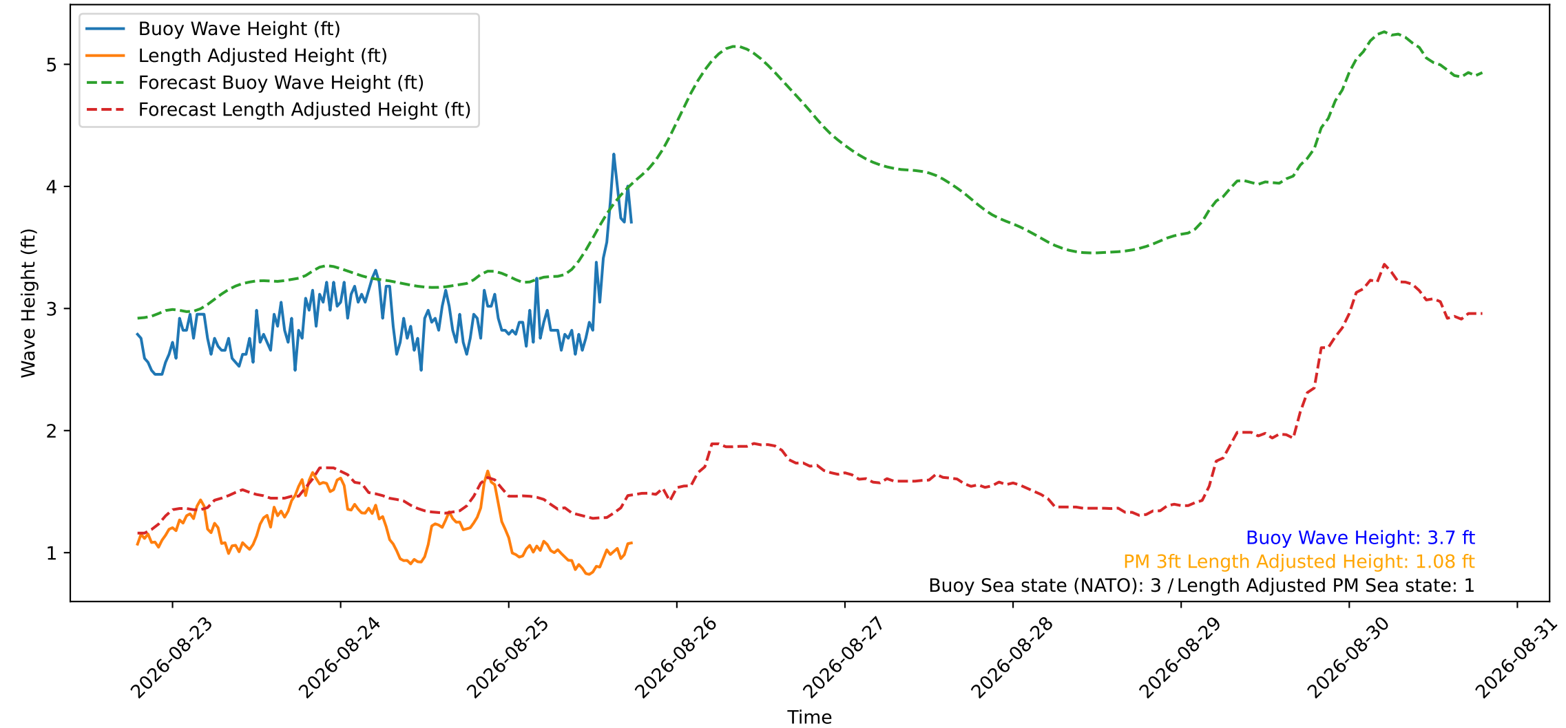
Wave Heights over Time for Green Beach at 2026-08-25 18:31:12
