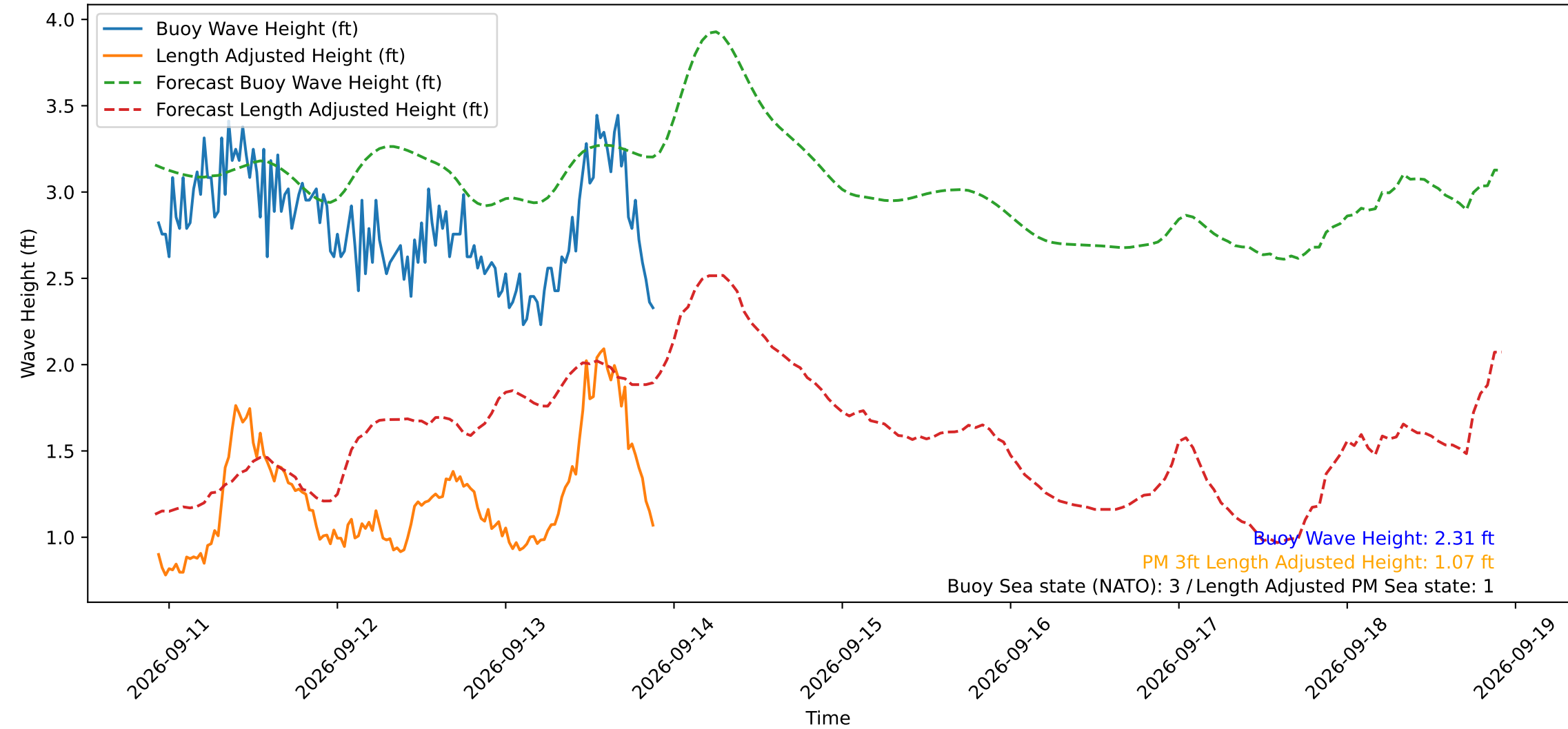
Wave Heights over Time for Red Beach at 2026-09-13 22:00:50
