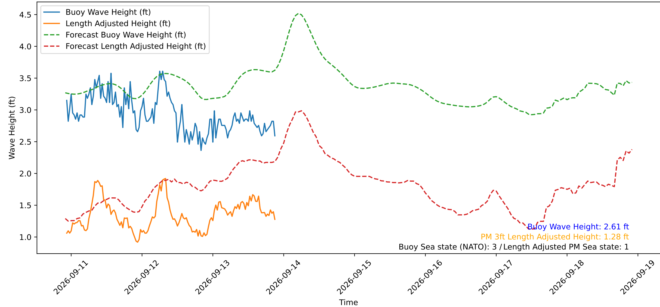
Wave Heights over Time for Green Beach at 2026-09-13 22:01:12
