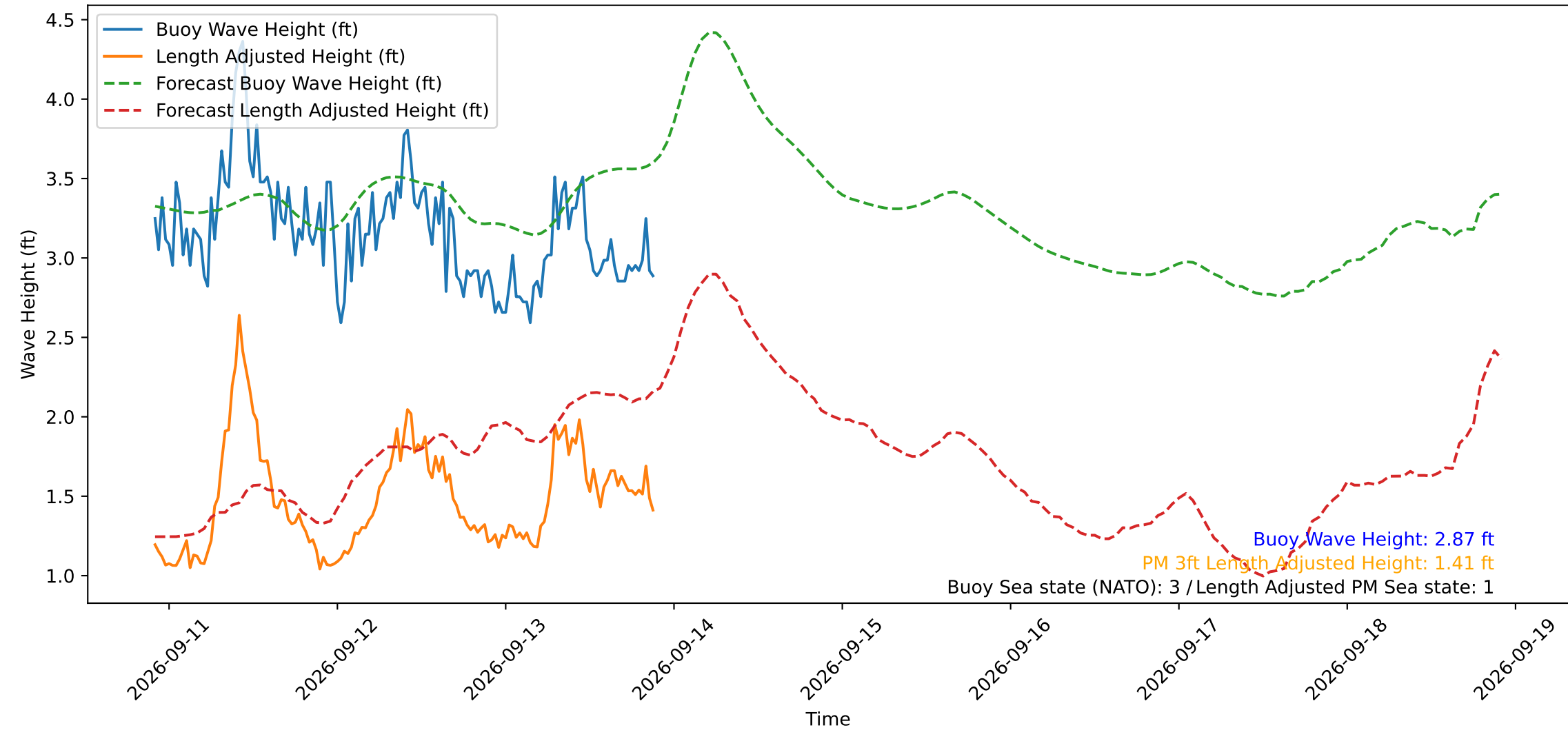
Wave Heights over Time for Oceanside Harbor at 2026-09-13 22:00:30
