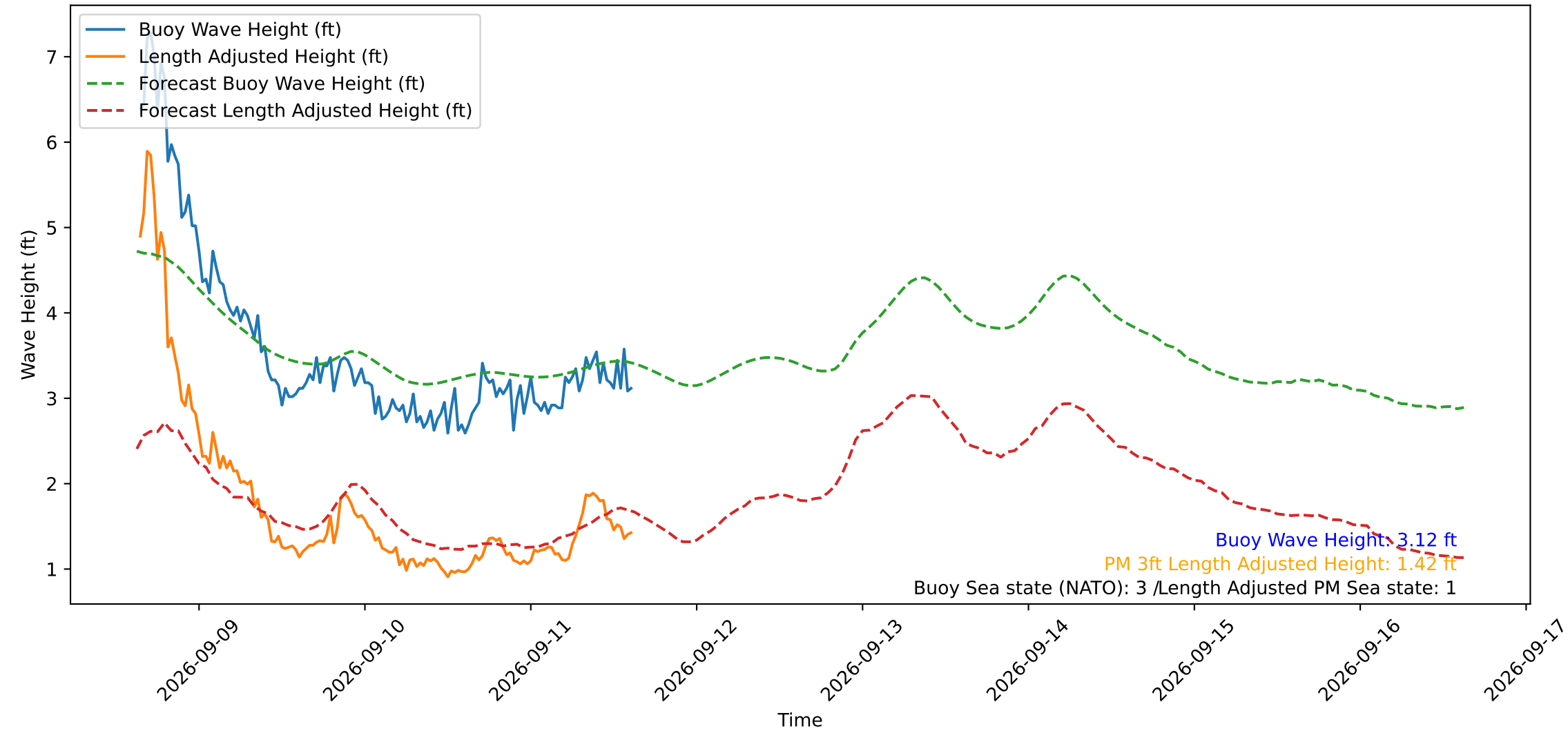
Wave Heights over Time for Green Beach at 2026-09-11 15:21:16
