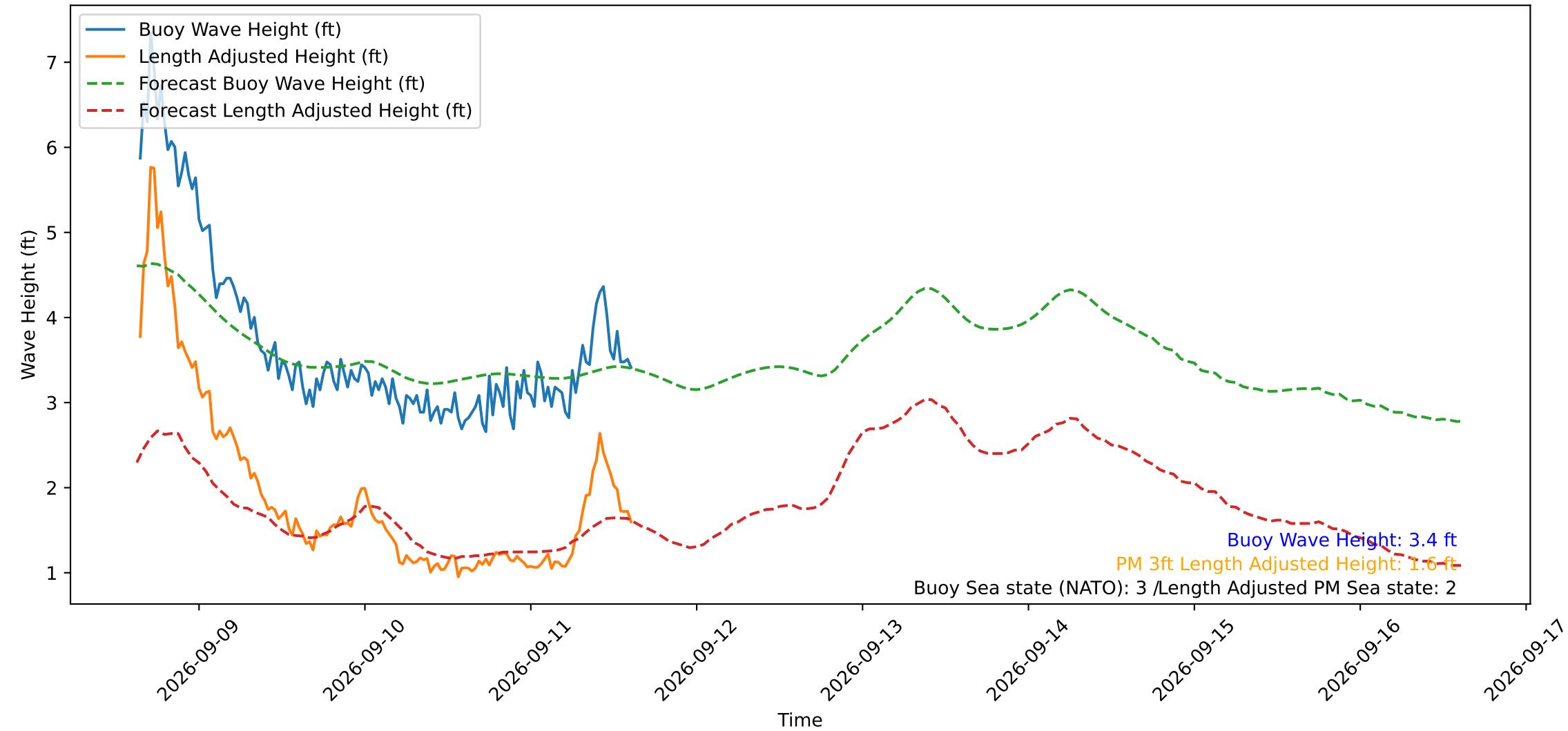
Wave Heights over Time for Oceanside Harbor at 2026-09-11 15:20:30
