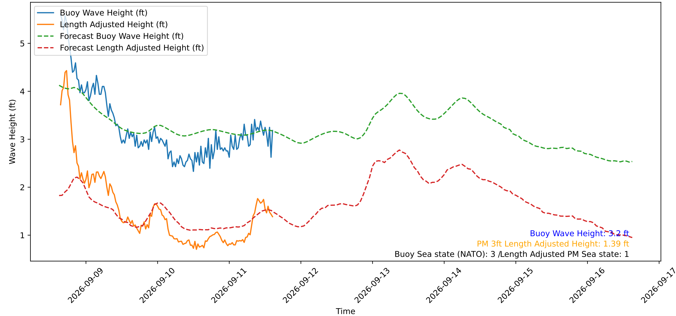
Wave Heights over Time for Red Beach at 2026-09-11 15:20:51
