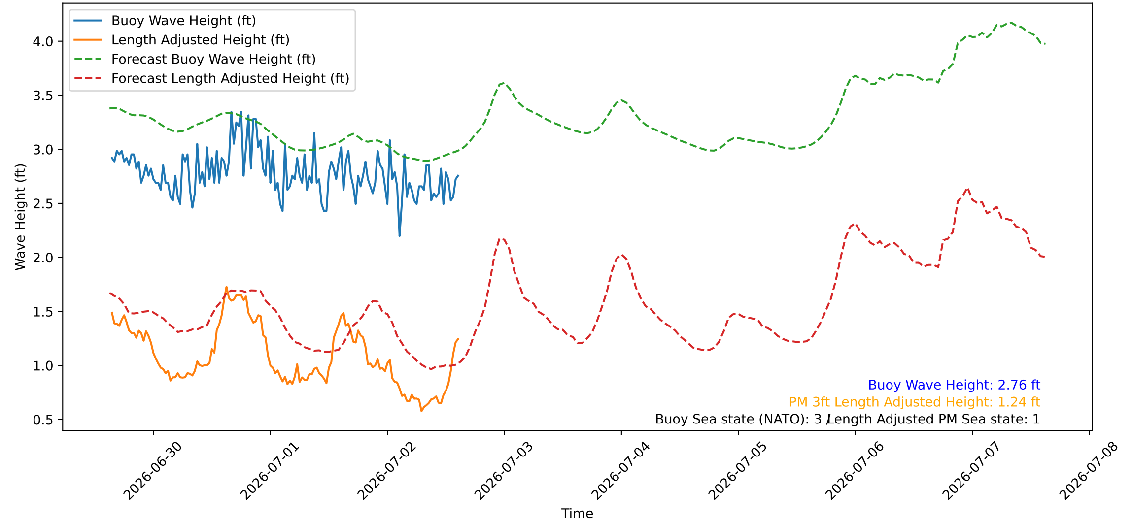
Wave Heights over Time for Red Beach at 2026-07-02 15:10:46
