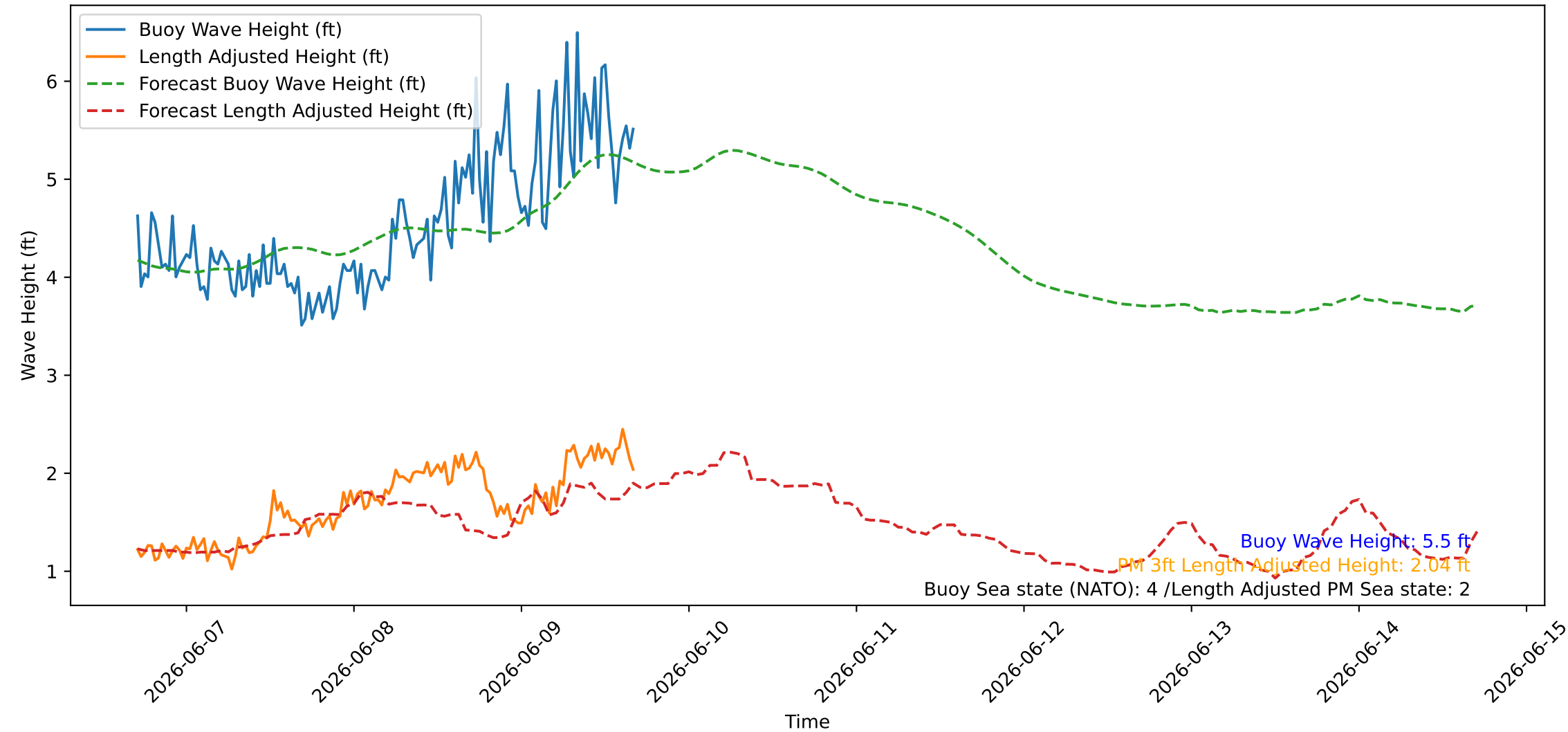
Wave Heights over Time for Oceanside Harbor at 2026-06-09 17:00:26
