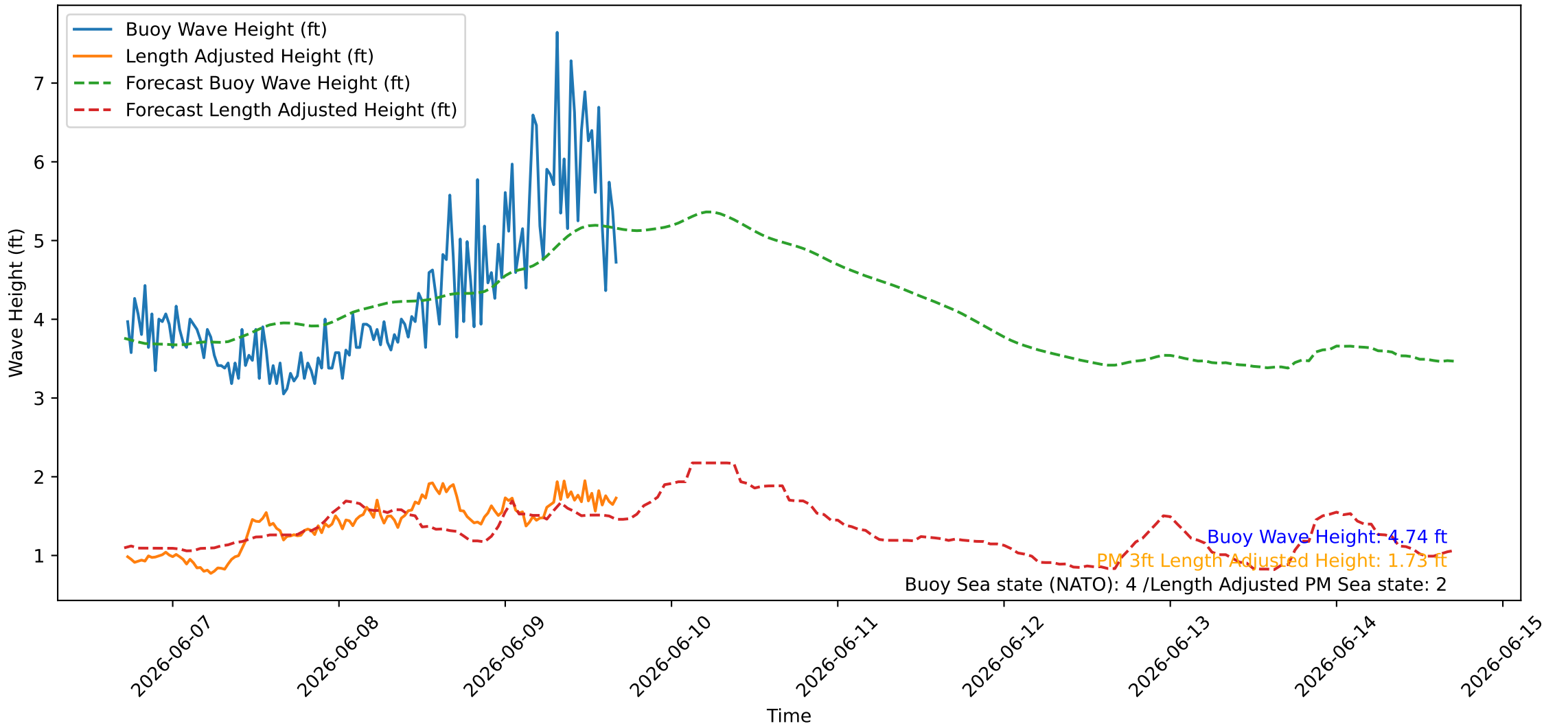
Wave Heights over Time for Red Beach at 2026-06-09 17:00:45
