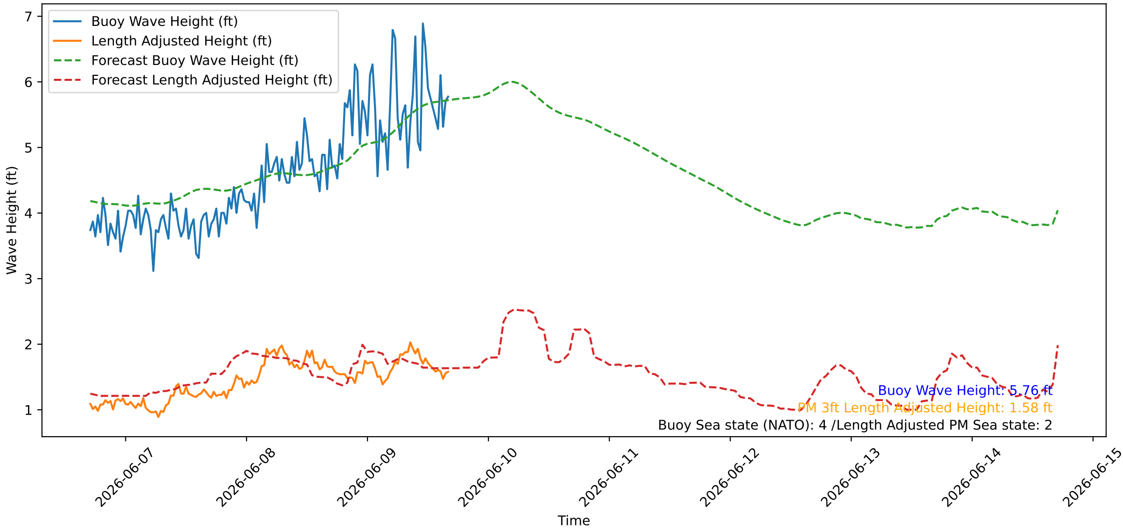
Wave Heights over Time for Green Beach at 2026-06-09 17:01:07
