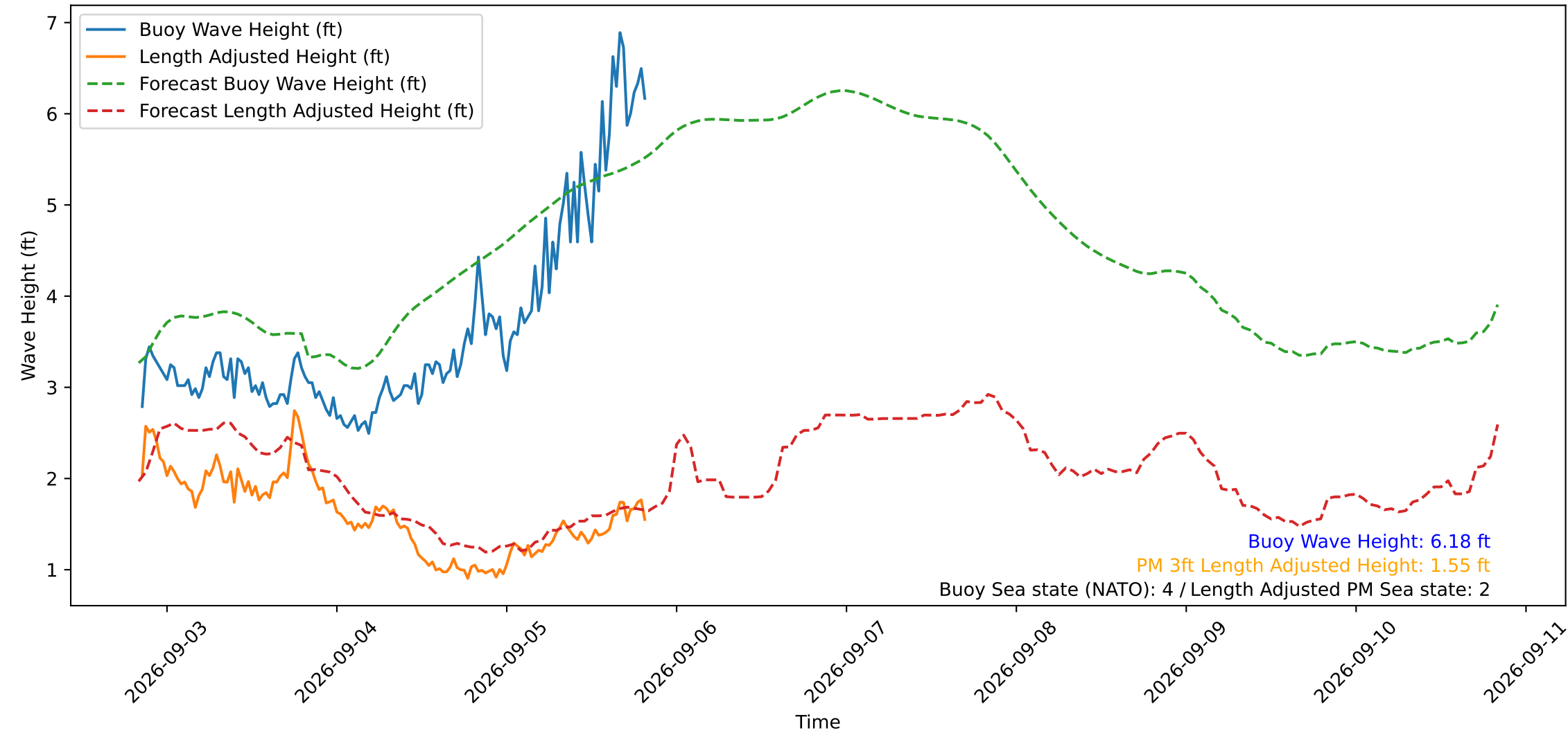
Wave Heights over Time for Green Beach at 2026-09-05 20:21:15
