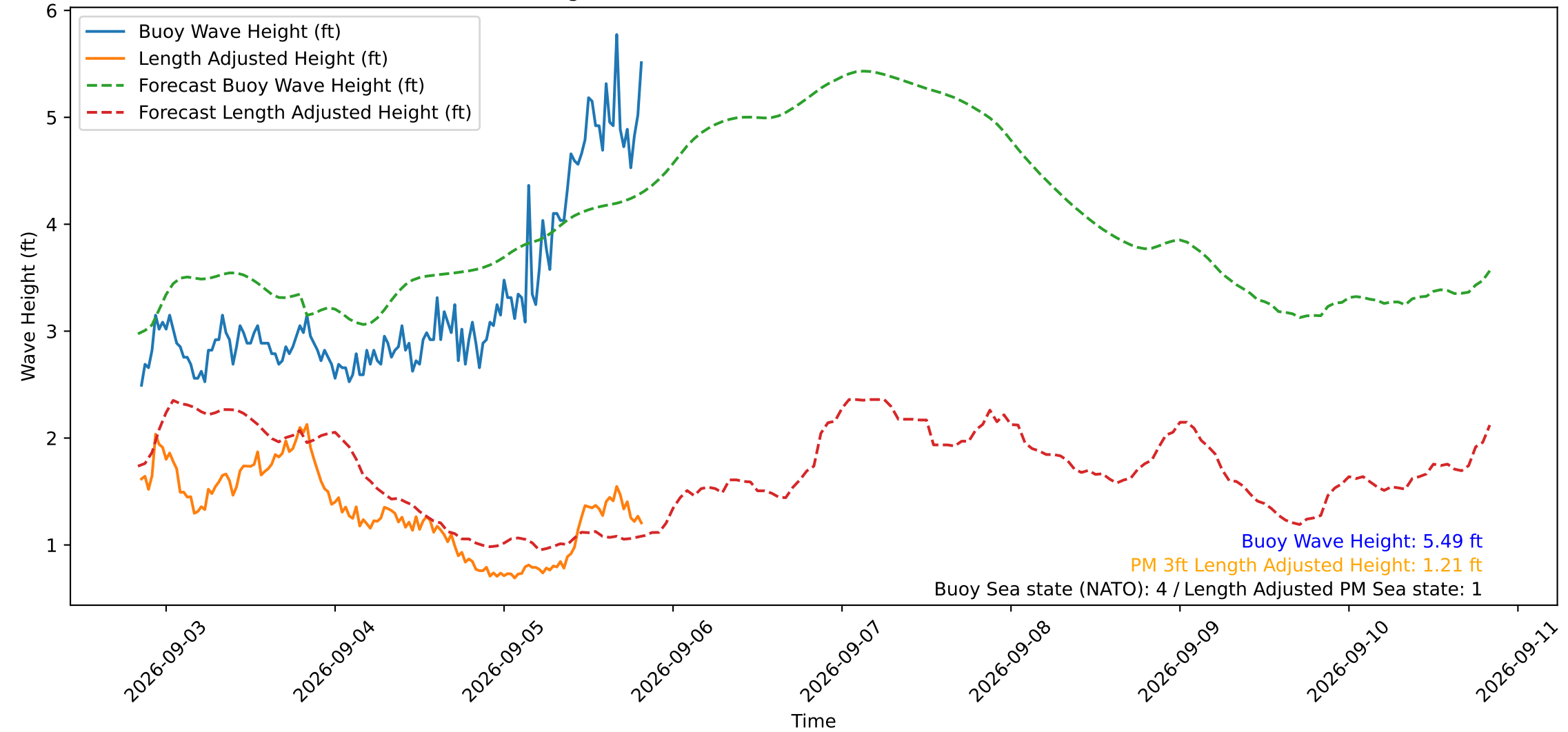
Wave Heights over Time for Red Beach at 2026-09-05 20:20:51
