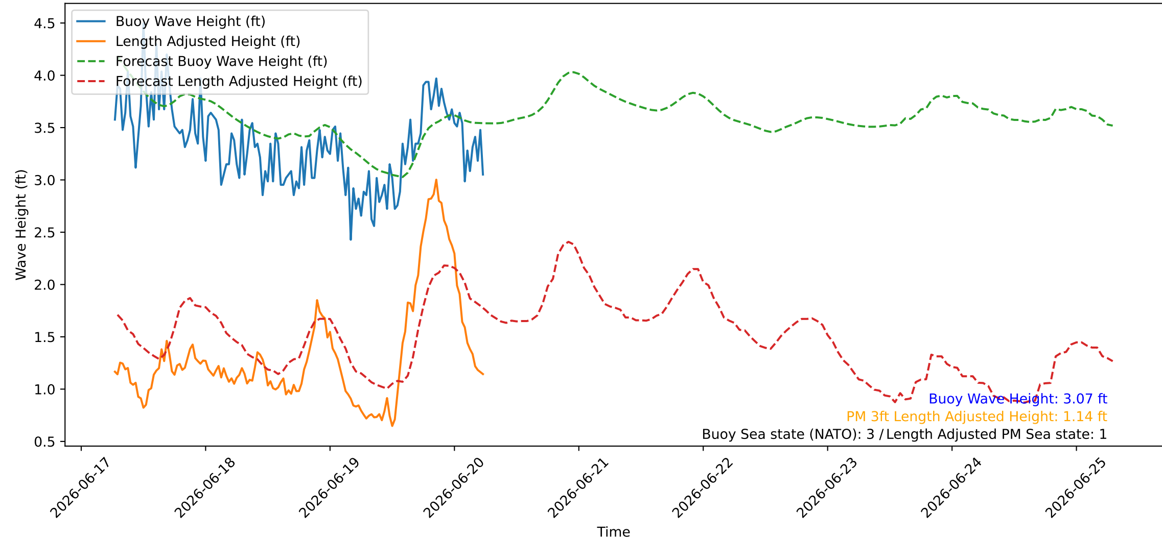
Wave Heights over Time for Green Beach at 2026-06-20 06:31:08
