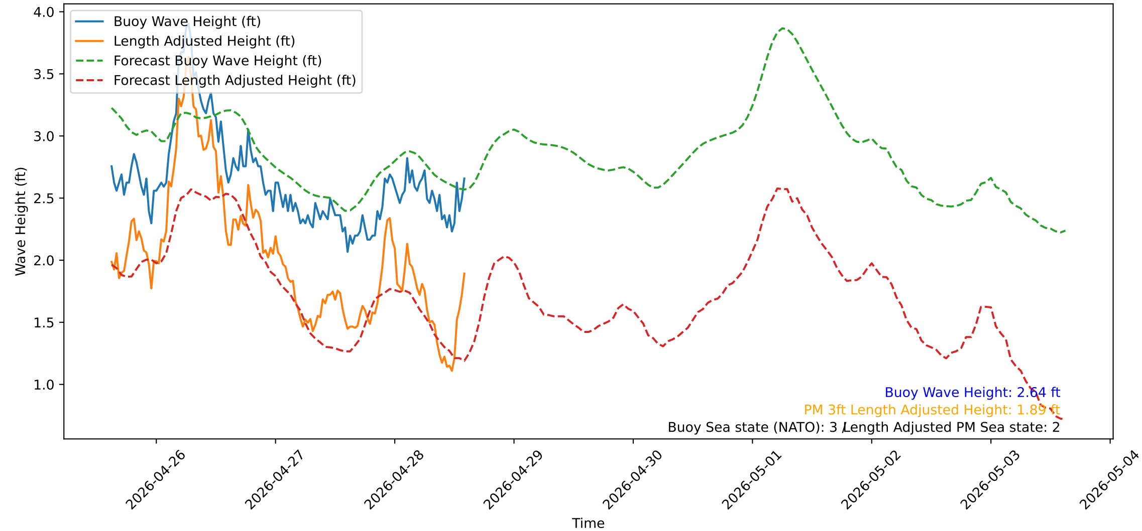
Wave Heights over Time for Oceanside Harbor at 2026-04-28 14:50:32
