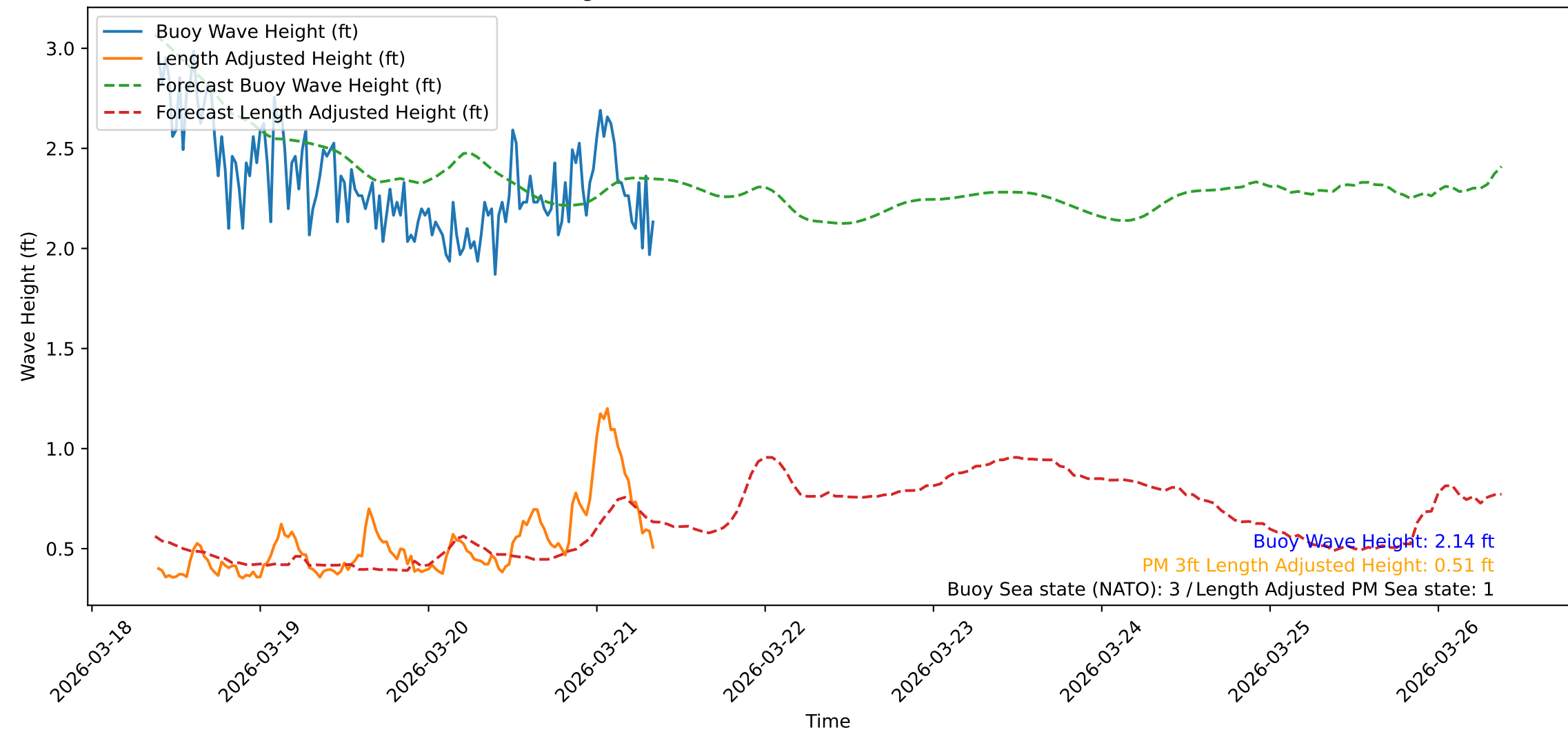
Wave Heights over Time for Red Beach at 2026-03-21 09:00:48
