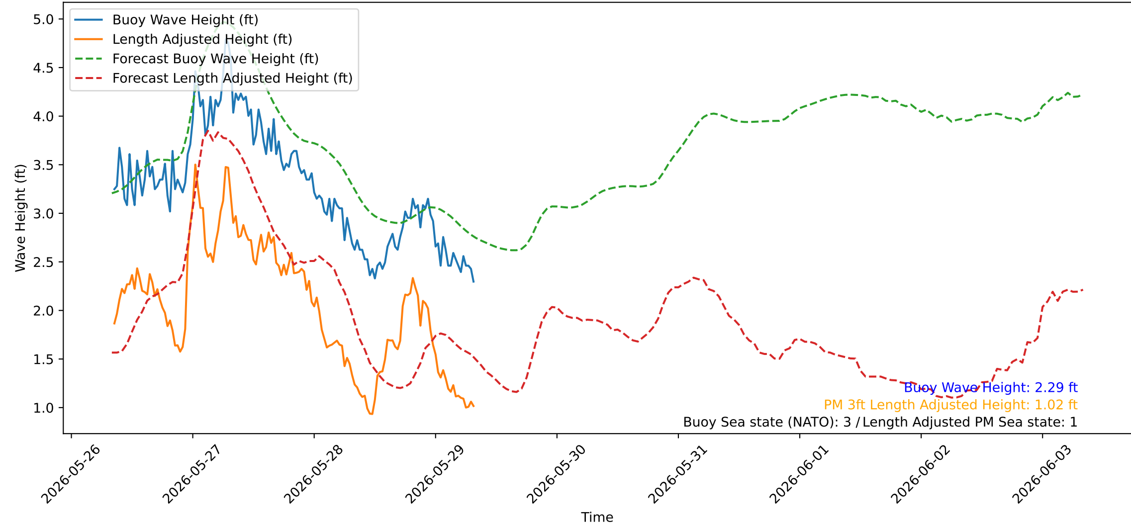
Wave Heights over Time for Red Beach at 2026-05-29 08:20:42
