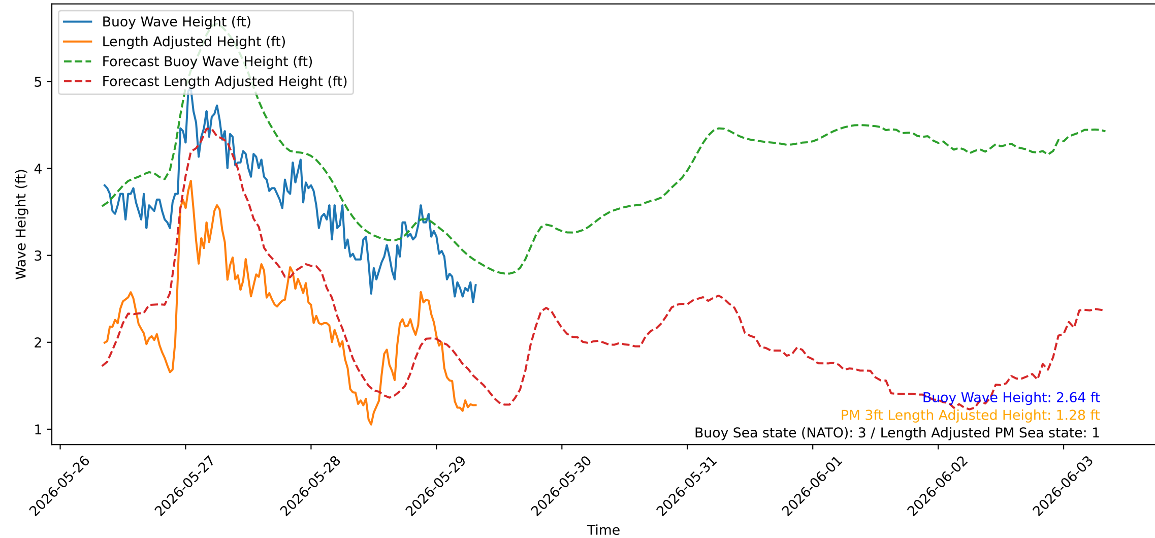
Wave Heights over Time for Green Beach at 2026-05-29 08:21:05
